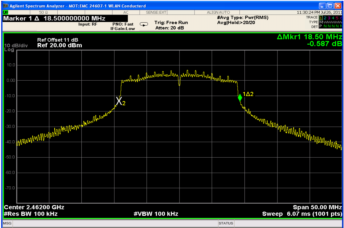
20 dB Bandwidth Channel 11 @ 13Mbps
