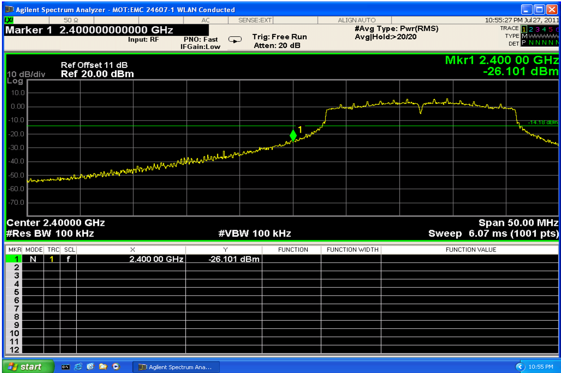
Channel 1 @ 14.4Mbps – Lower Band Edge
