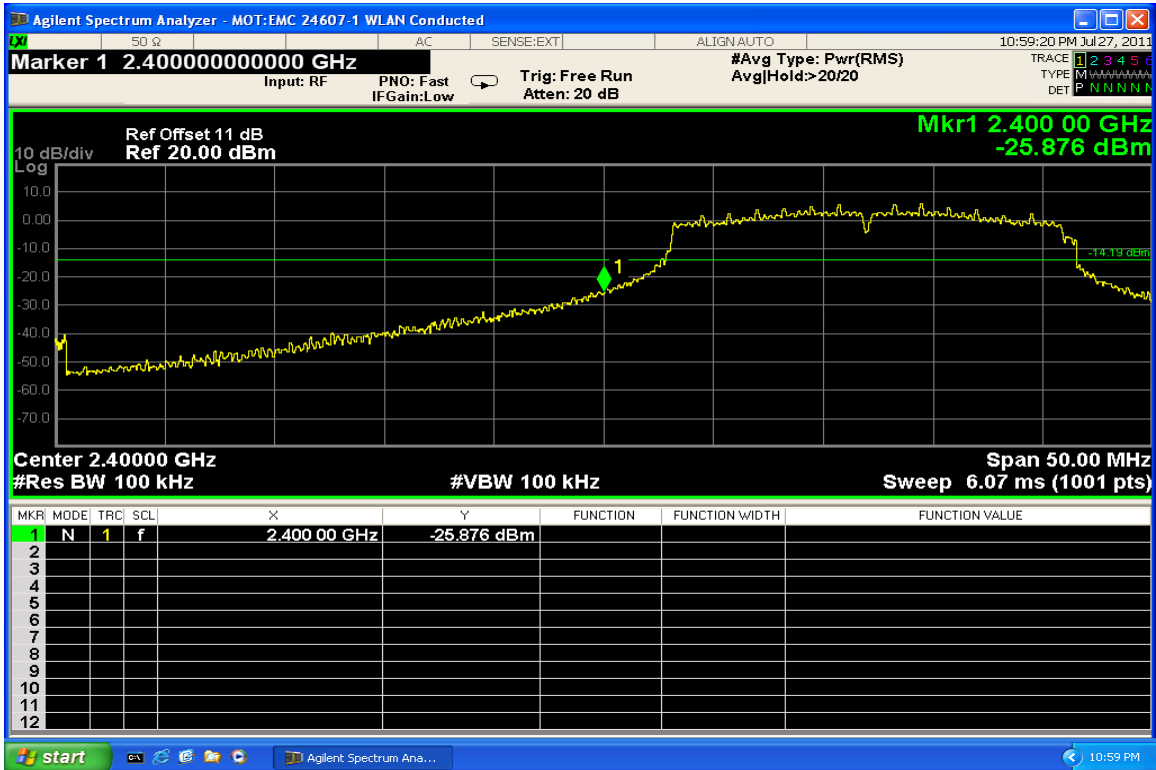
Channel 1 @ 13Mbps – Lower Band Edge
