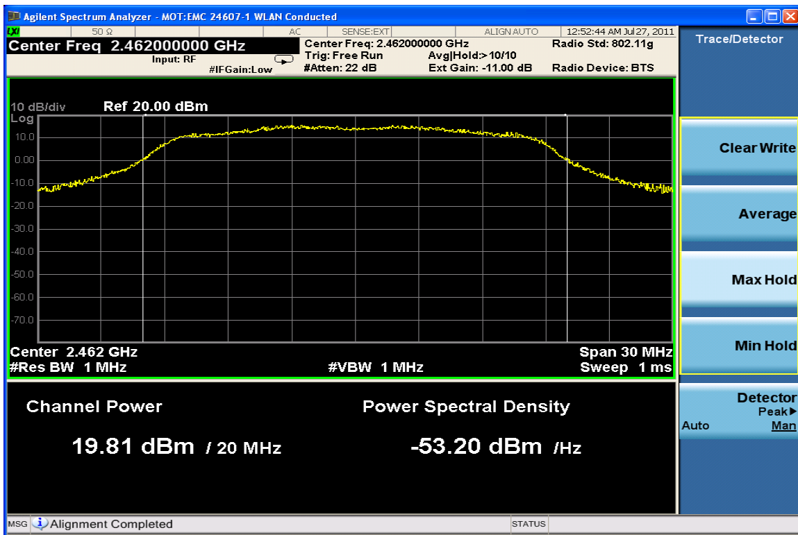
Max. Power Channel 11 @ 13Mbps
