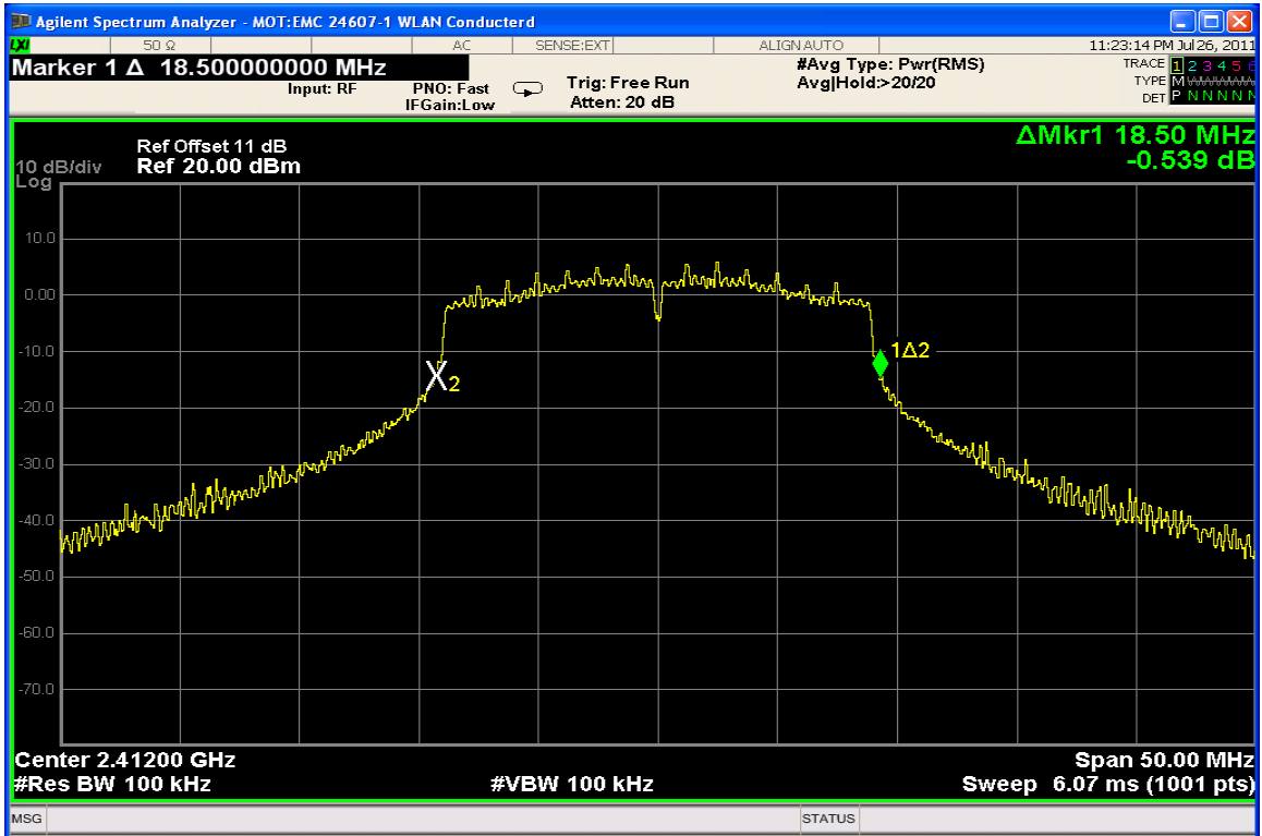
20 dB Bandwidth Channel 1 @ 13Mbps
