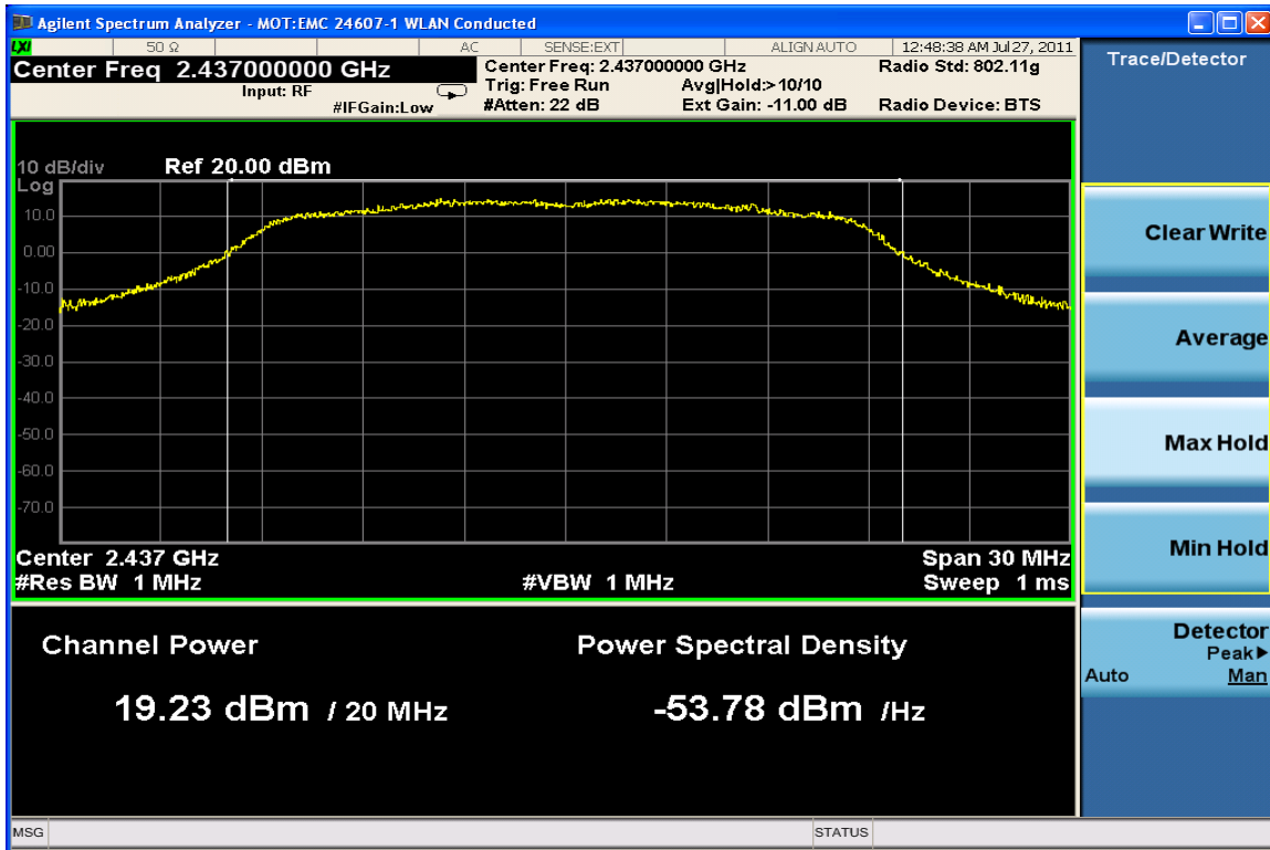
Max. Power Channel 6 @ 13Mbps
