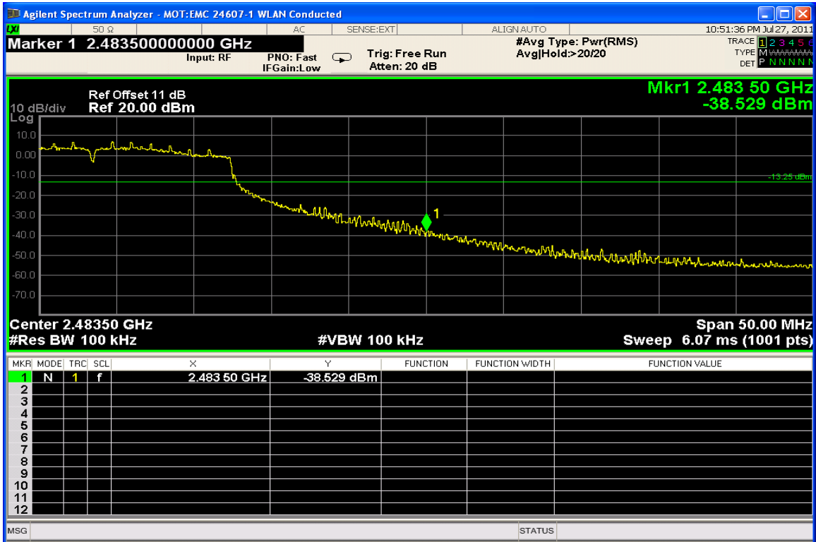
Channel 11 @ 14.4Mbps – Upper Band Edge
