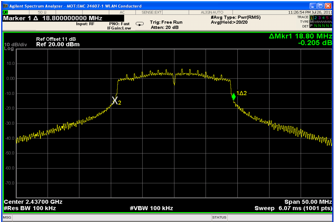
20 dB Bandwidth Channel 6 @ 13Mbps
