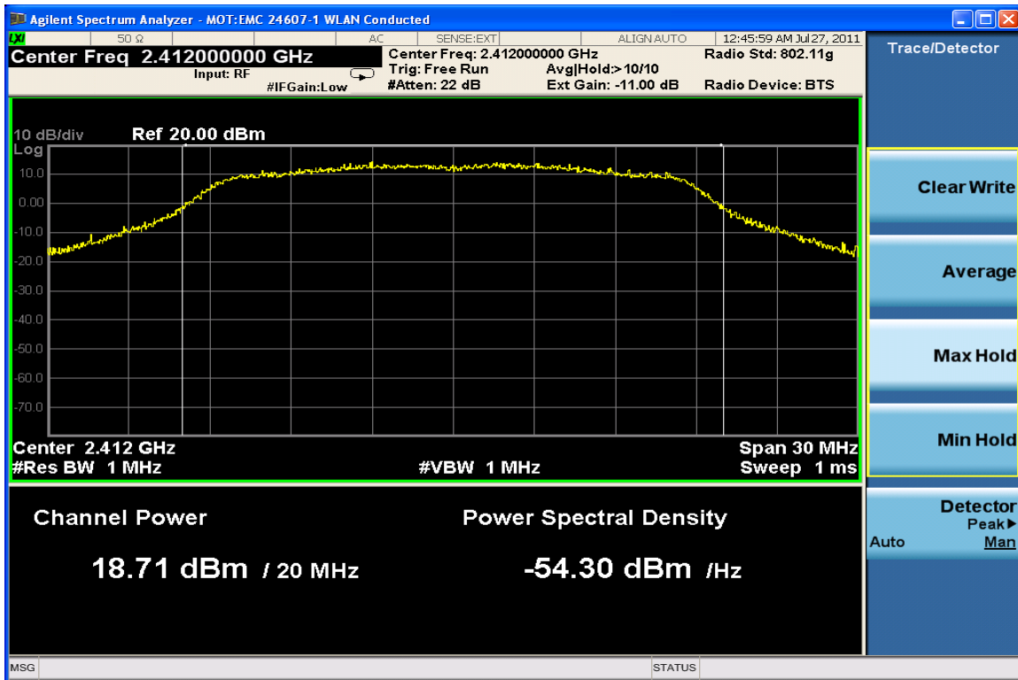
Max. Power Channel 1 @ 13Mbps
