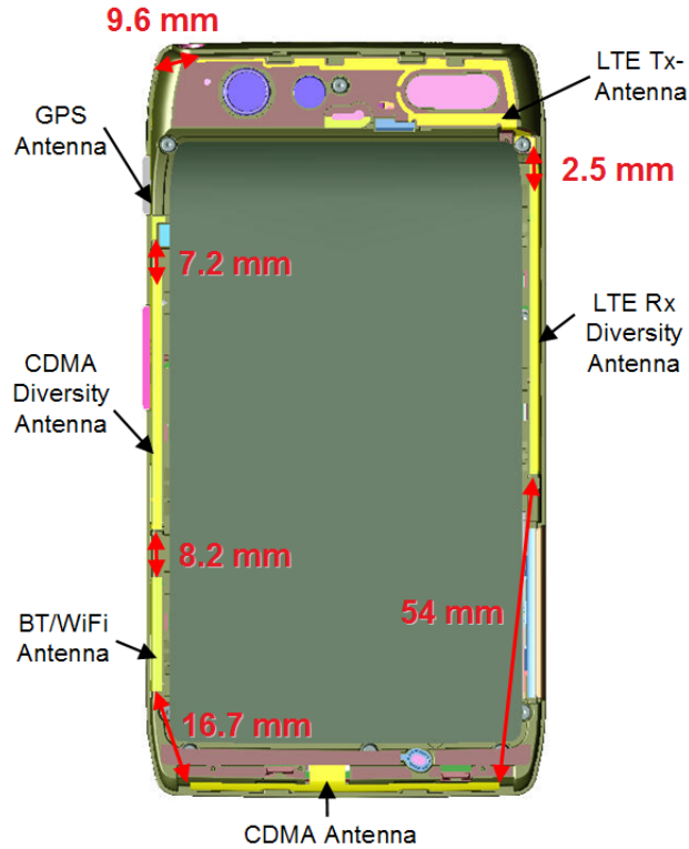
Figure 2: Antenna Separation Distances
