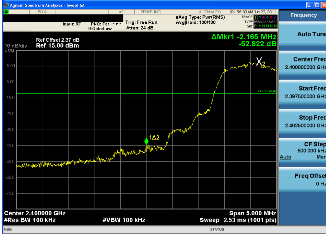
Plot 6-10. Band Edge Plot (Bluetooth, 2Mbps – Ch. 0)
