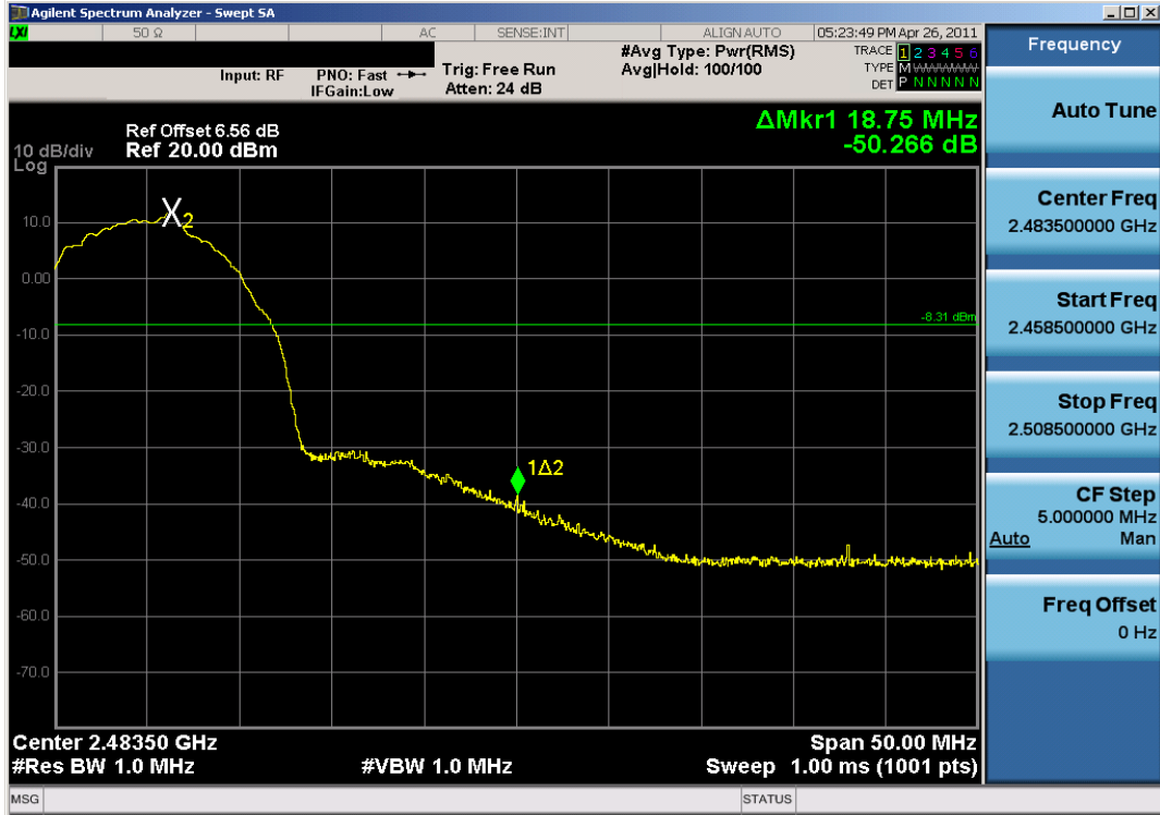
Plot 6-22. Band Edge Plot (802.11b – Ch. 11)
