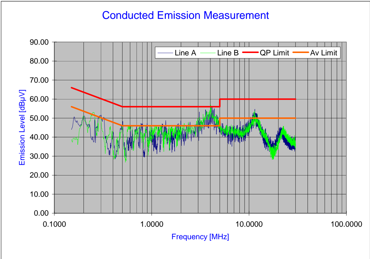
Plot 6-39. Line Conducted Plot with 802.11n
