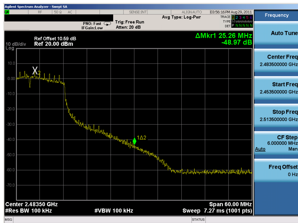
Plot 6-29. Band Edge Plot (802.11n – Ch. 10)
