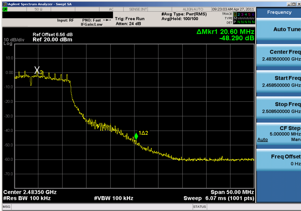
Plot 6-26. Band Edge Plot (802.11g – Ch. 11)
