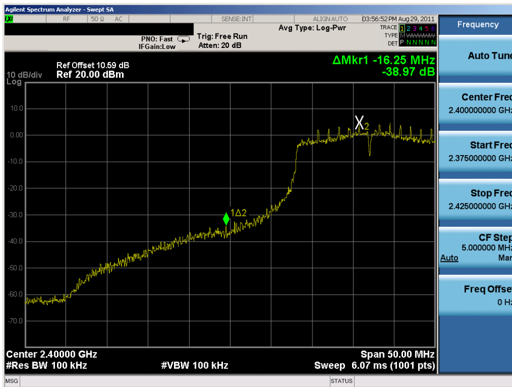
Plot 6-28. Band Edge Plot (802.11n – Ch. 2)
