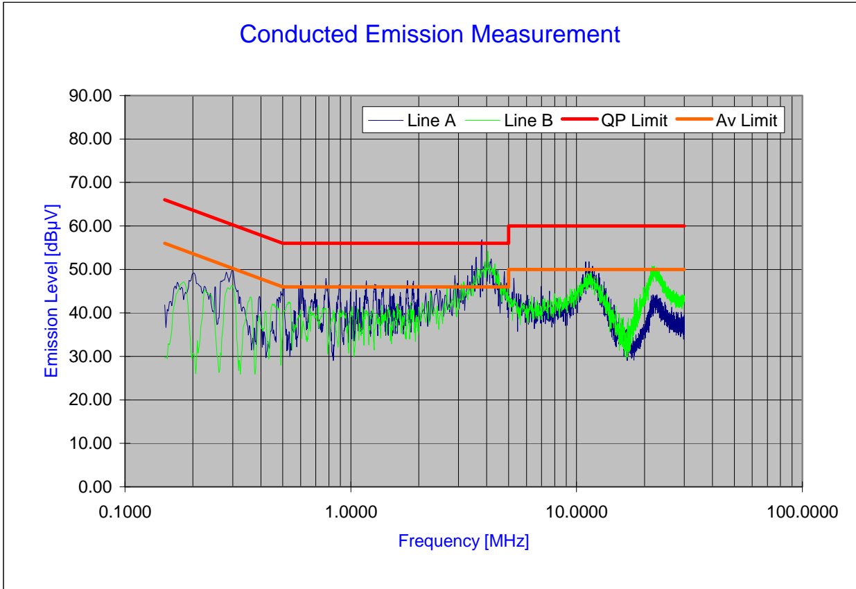
Plot 6-37. Line Conducted Plot with 802.11b
