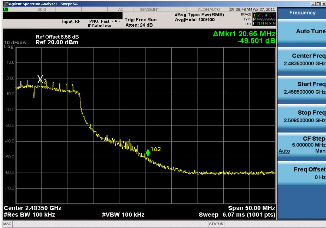
Plot 6-30. Band Edge Plot (802.11n – Ch. 11)
