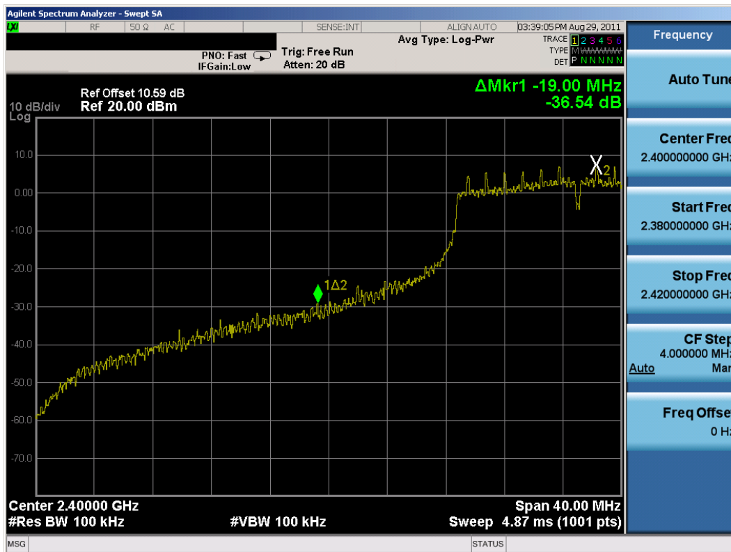
Plot 6-24. Band Edge Plot (802.11g – Ch. 2)
