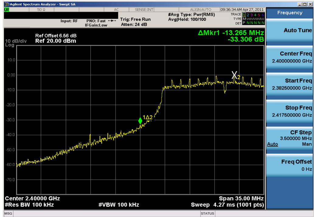
Plot 6-27. Band Edge Plot (802.11n – Ch. 1)
