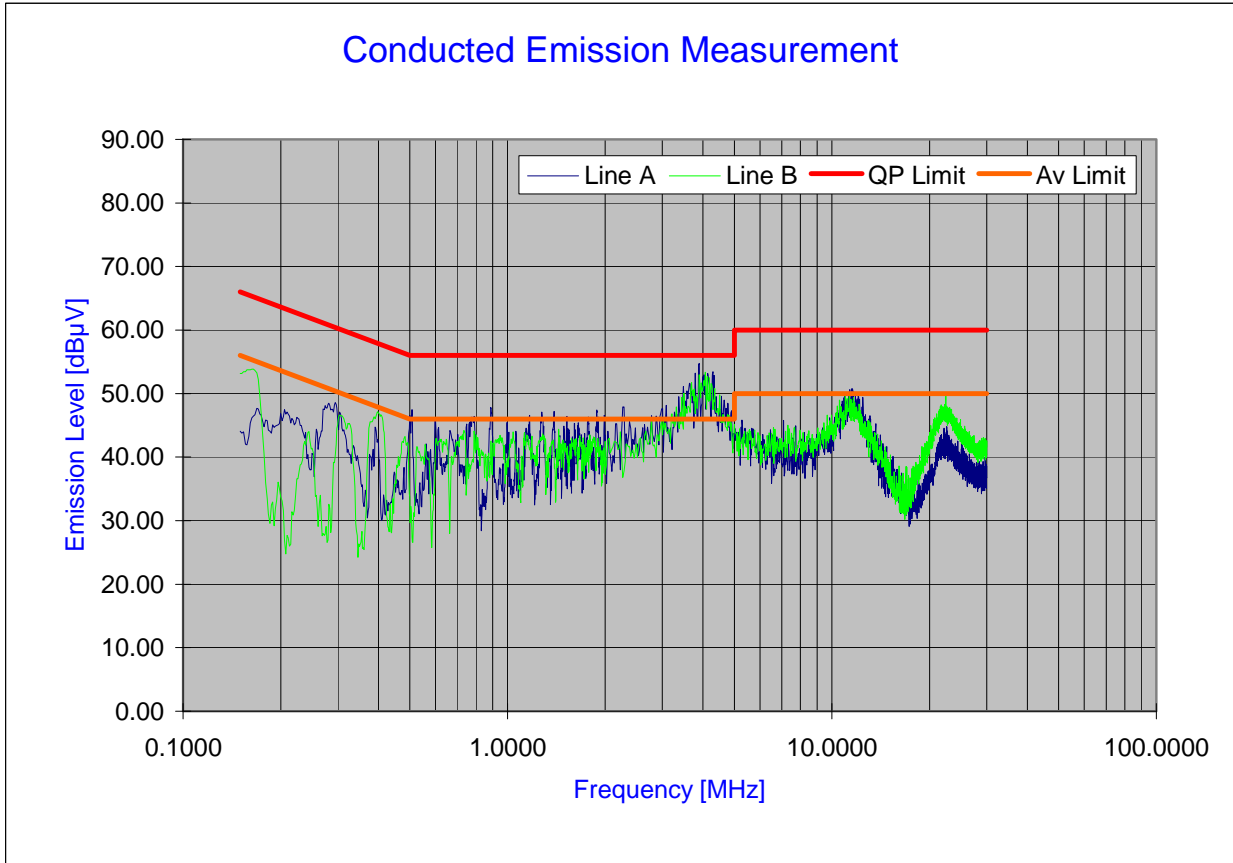
Plot 6-38. Line Conducted Plot with 802.11g
