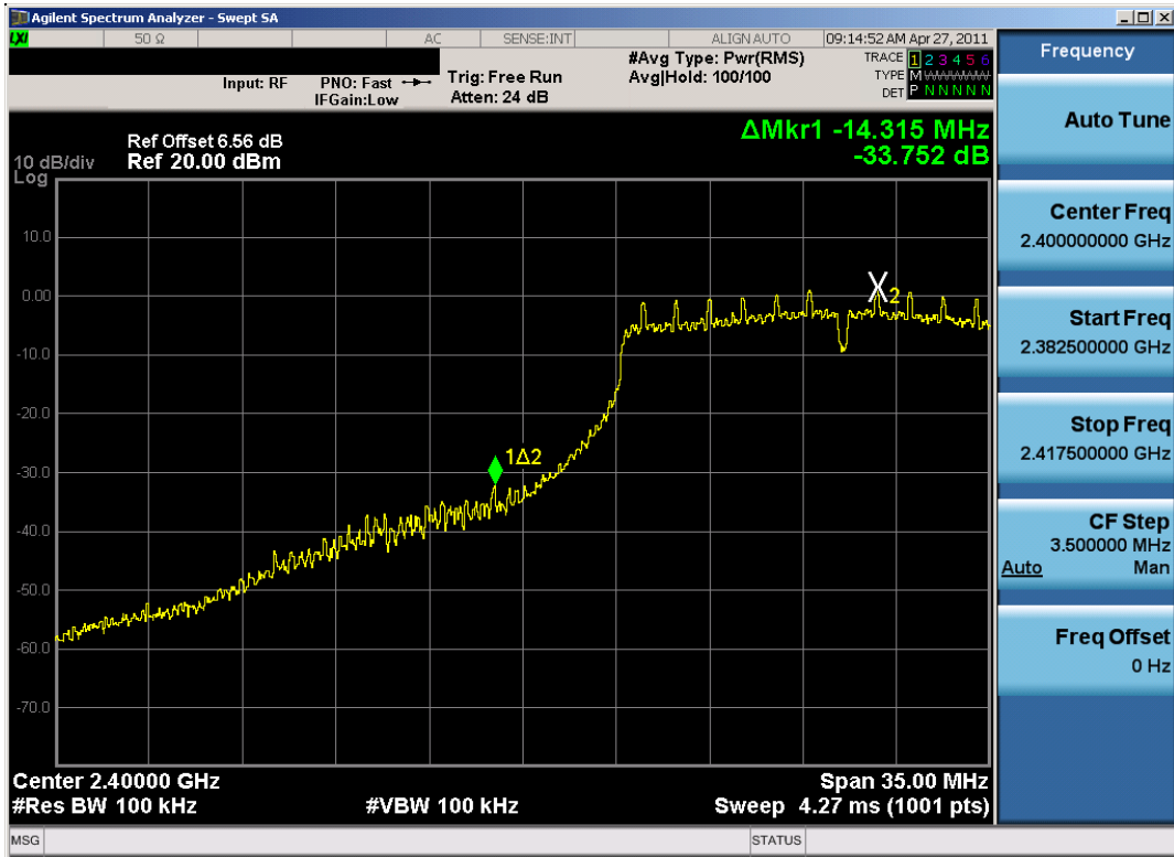
Plot 6-23. Band Edge Plot (802.11g – Ch. 1)
