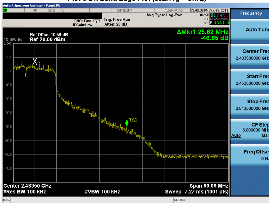
Plot 6-25. Band Edge Plot (802.11g – Ch. 10)
