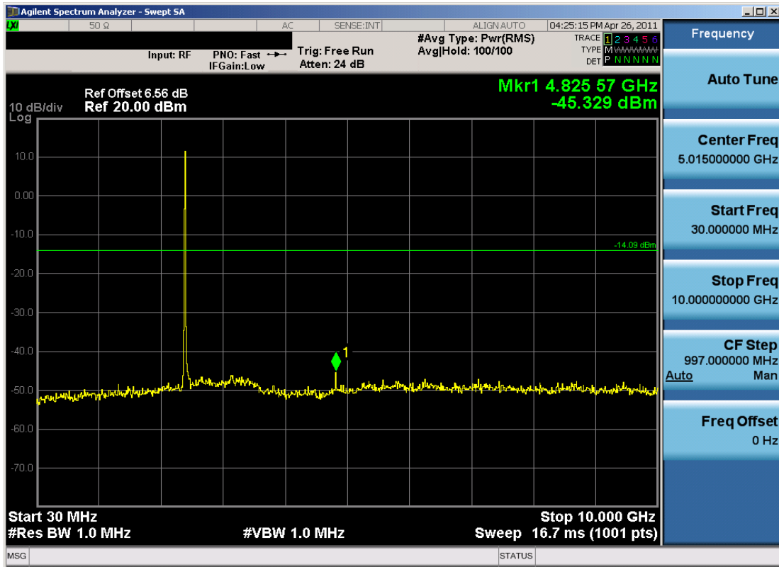
Plot 6-31. Conducted Spurious Plot (802.11b – Ch. 1)
