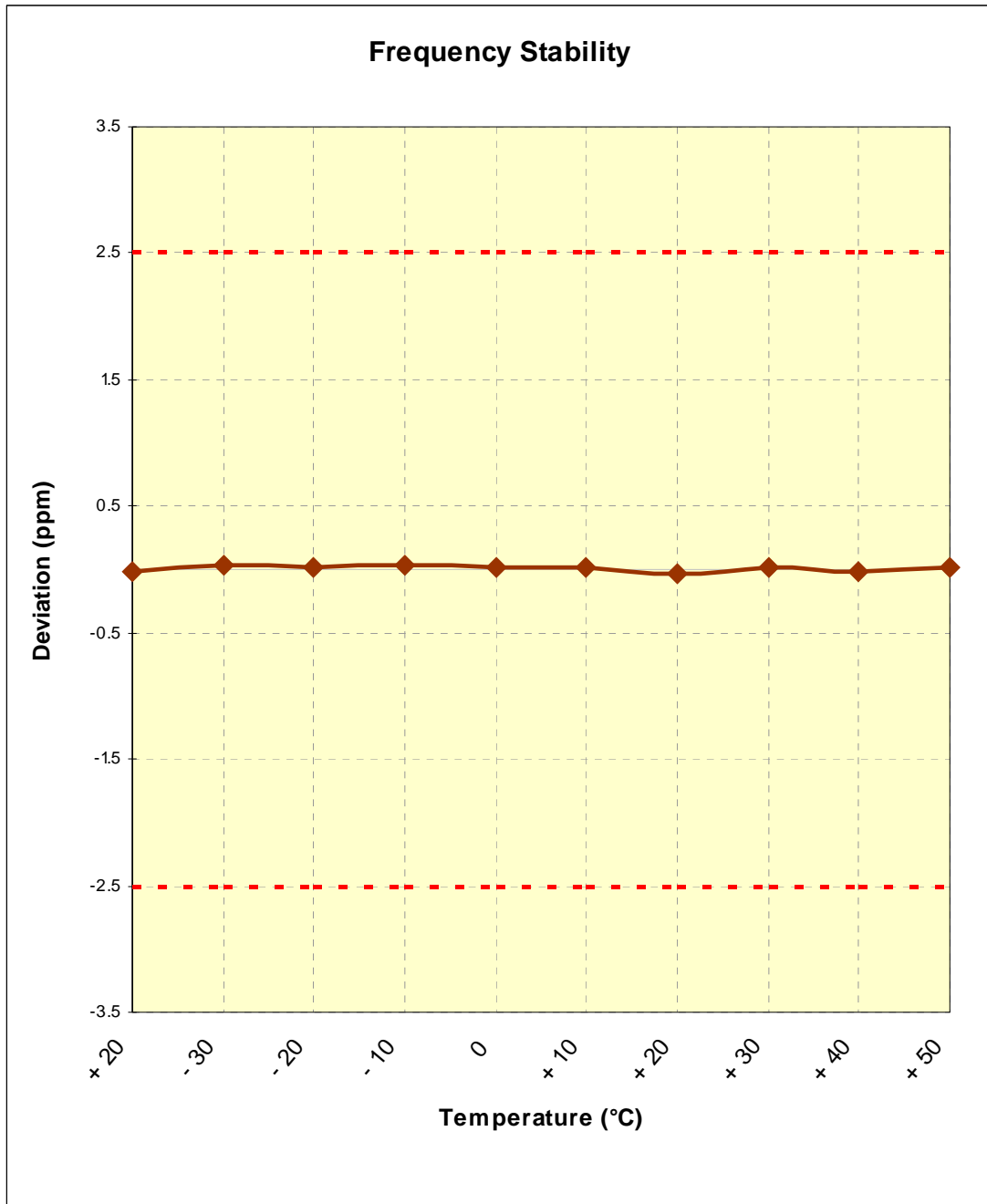
Figure 6-3. Frequency Stability Graph (Cellular CDMA Mode – Ch. 384)
