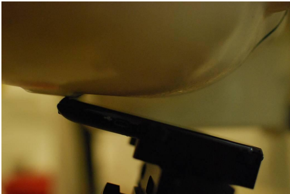
Figure 24-2 SAR Test Setup Photo – Right Tilt
