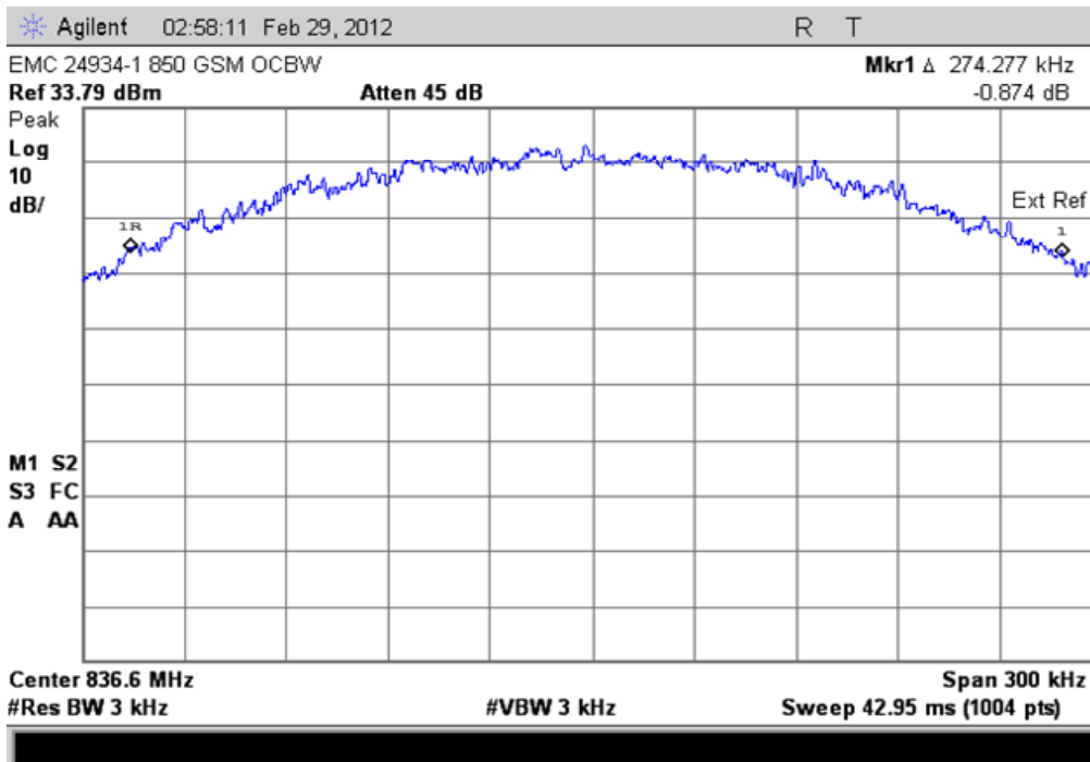
GSM 850 – Reference Level Plot – Channel 190 (836.60 MHz)
