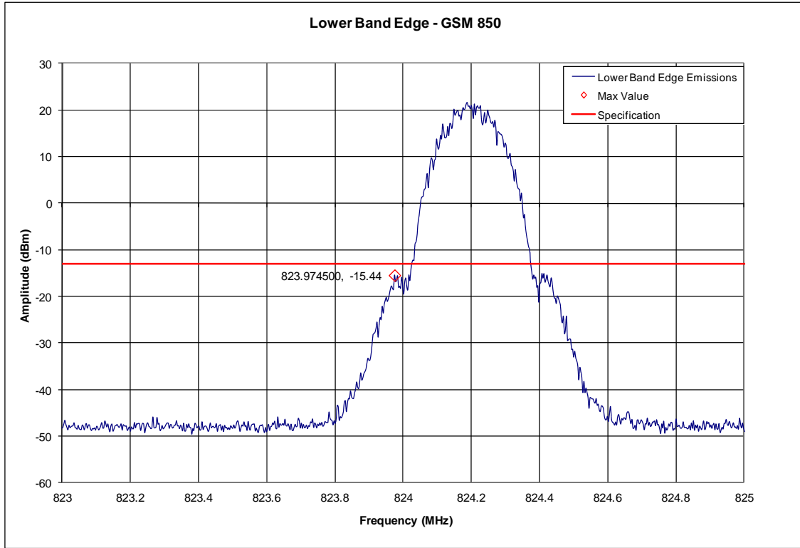
GSM 850 – Lower Band Edge – Channel 128 (824.2 MHz)
