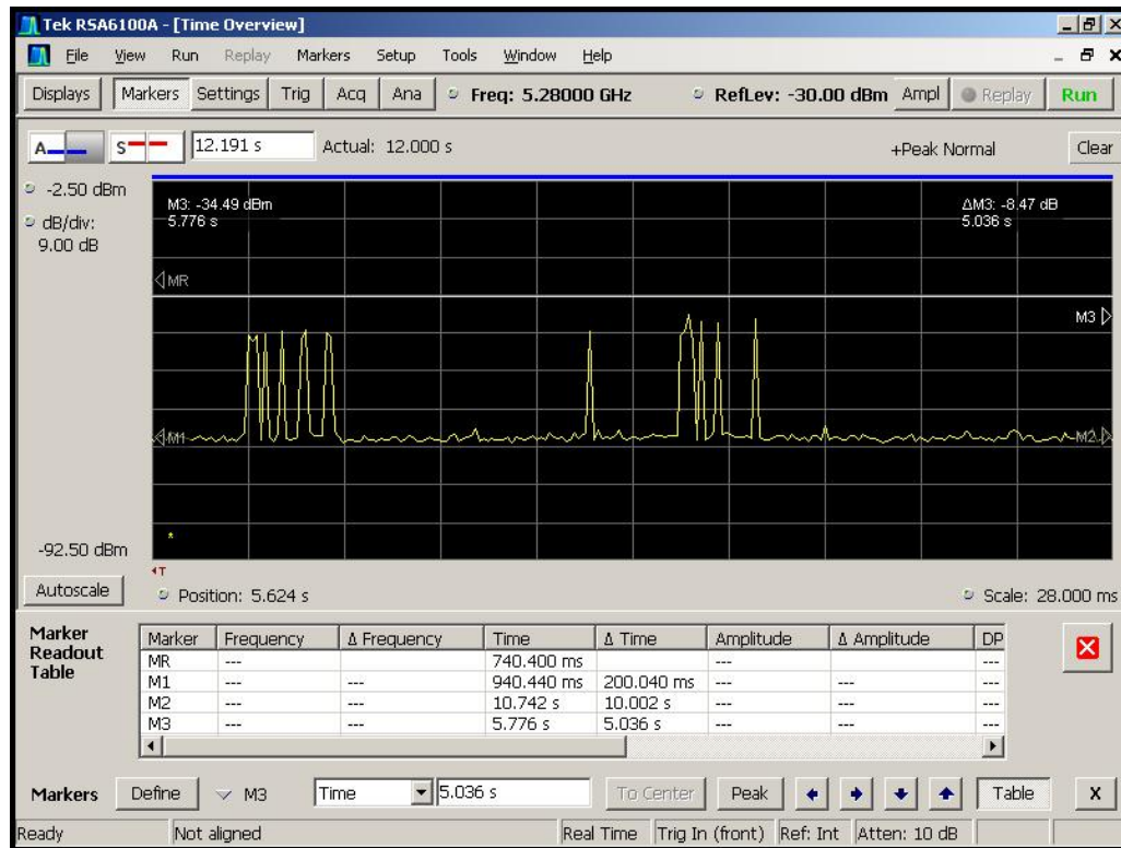
Figure 5-8. Channel Closing Pulses, Aggregate Time After 200ms
