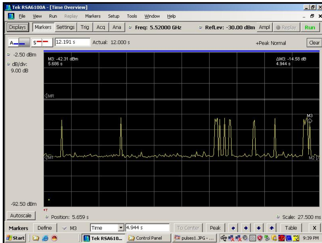
Figure 6-9. Channel Closing Pulses, Aggregate Time After 200ms
