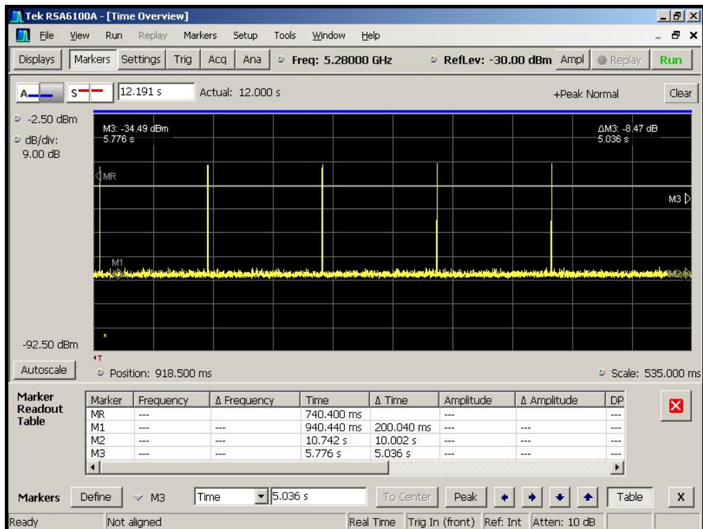
Figure 5-7. Channel Closing Pulses, Aggregate Time After 200ms
