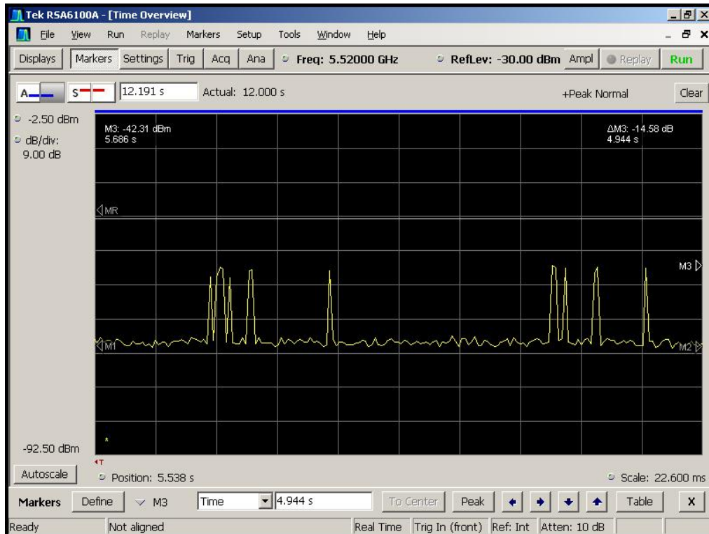
Figure 6-8. Channel Closing Pulses, Aggregate Time After 200ms
