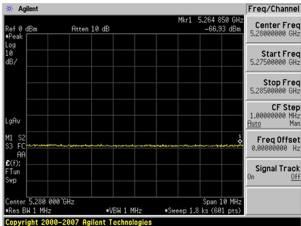
Figure 5-11 Non-occupancy Period - Monitoring live real time spectrum - Elapse time 30 minutes
