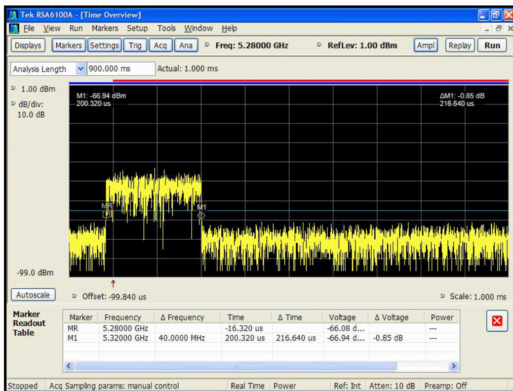
Figure 5-10. Pulse Width After 200ms
