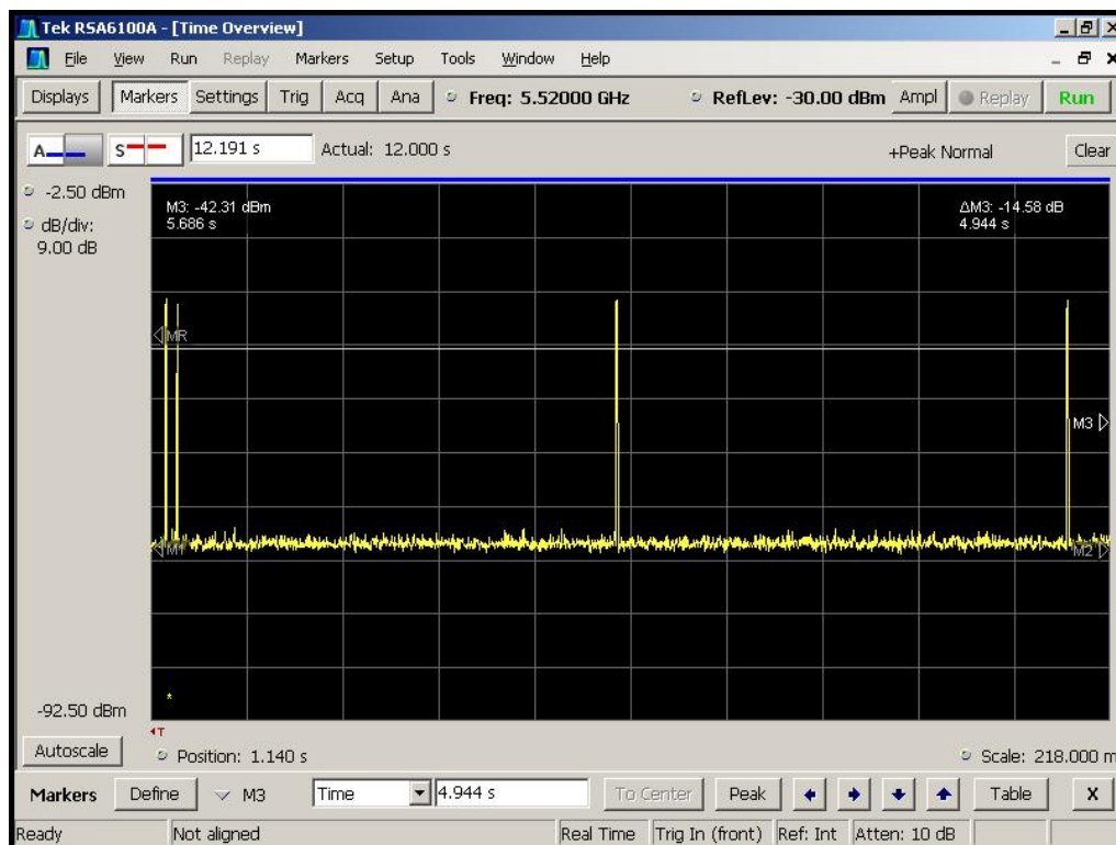
Figure 6-6. Channel Closing Pulses, Aggregate Time After 200ms
