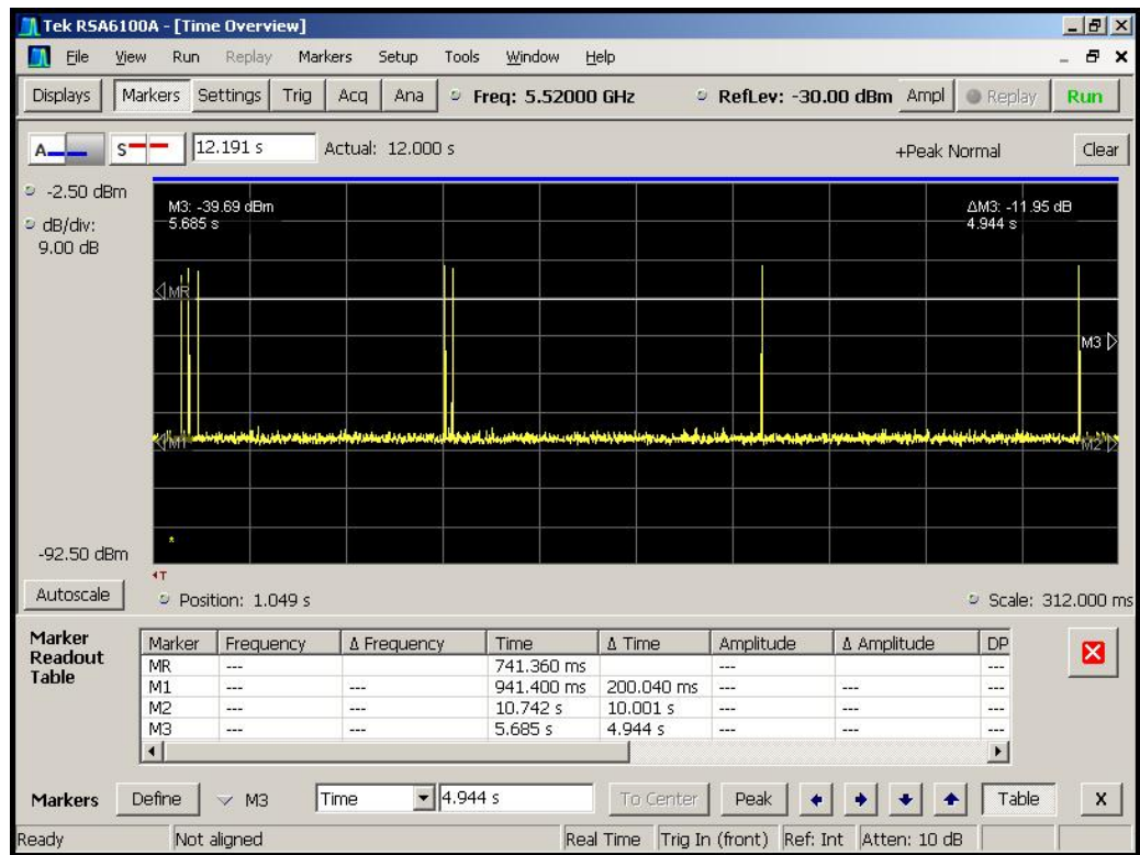
Figure 6-7. Channel Closing Pulses, Aggregate Time After 200ms
