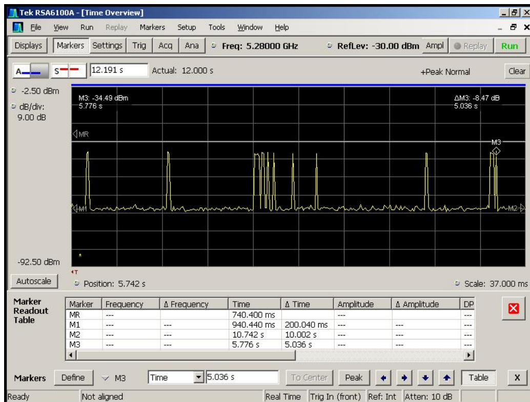
Figure 5-9. Channel Closing Pulses, Aggregate Time After 200ms
