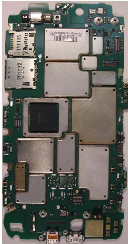
XCVR TOP SIDE W/SHIELDS
