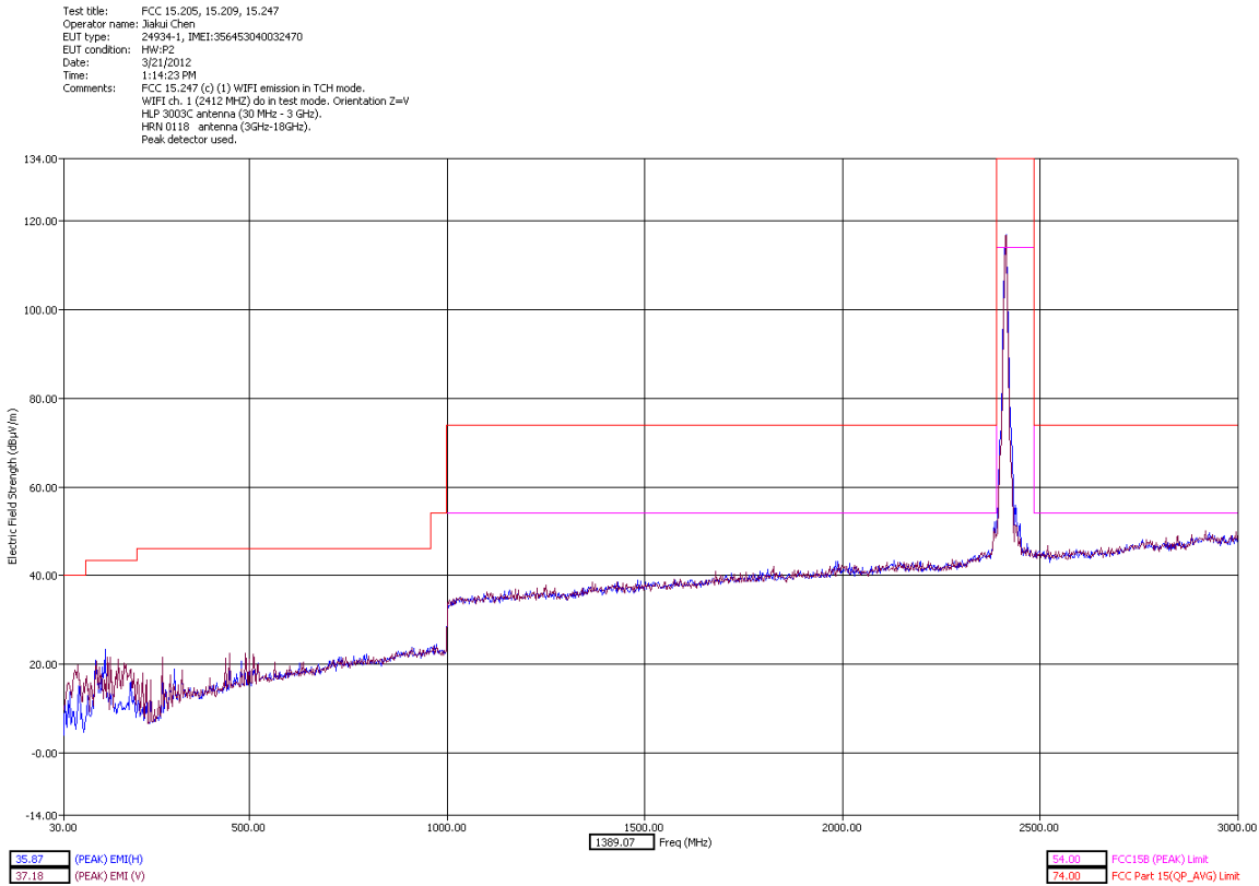
30 MHz – 3 GHz Low Channel Dual Polarization Z
