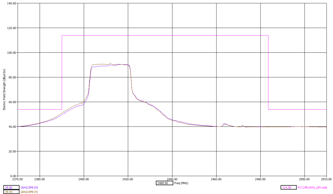
Low Channel Band Edge Z Orientation AVG Detector
