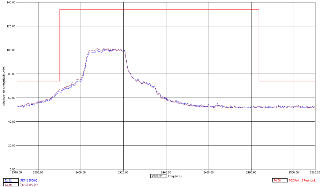
Low Channel Band Edge Z Orientation Peak Detector
