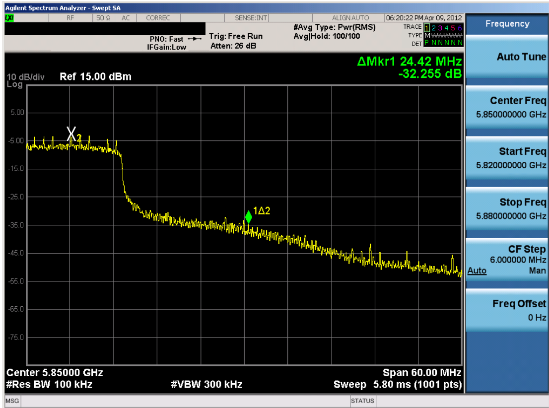
6-24. Band Edge Plot (802.11n (5.8GHz – 40MHz) – Ch. 163)
