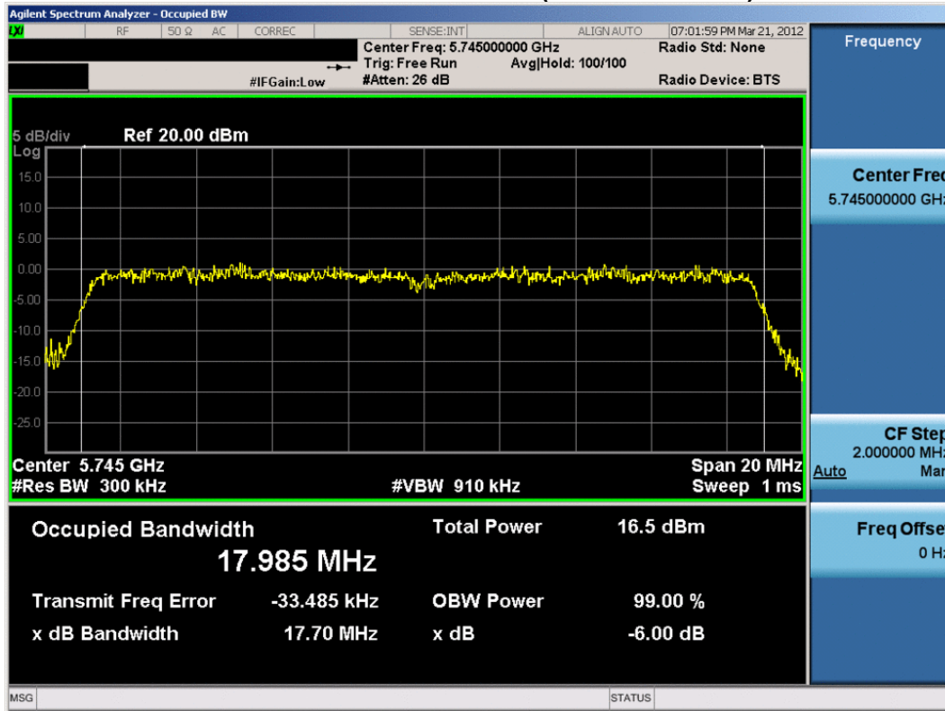
Plot 6-4. 6dB Bandwidth Plot (802.11n (5.8GHz – 20MHz BW) – Ch. 149)
