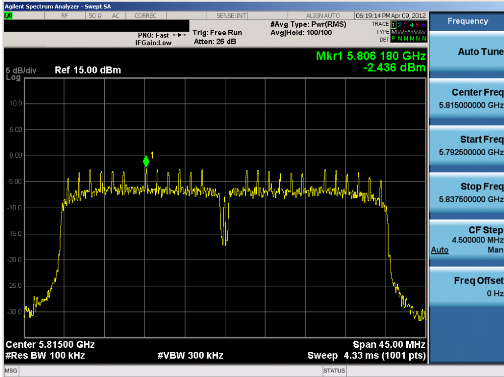
Plot 6-18. Power Spectral Density Plot (802.11n (5.8GHz – 40MHz BW) – Ch. 163)
