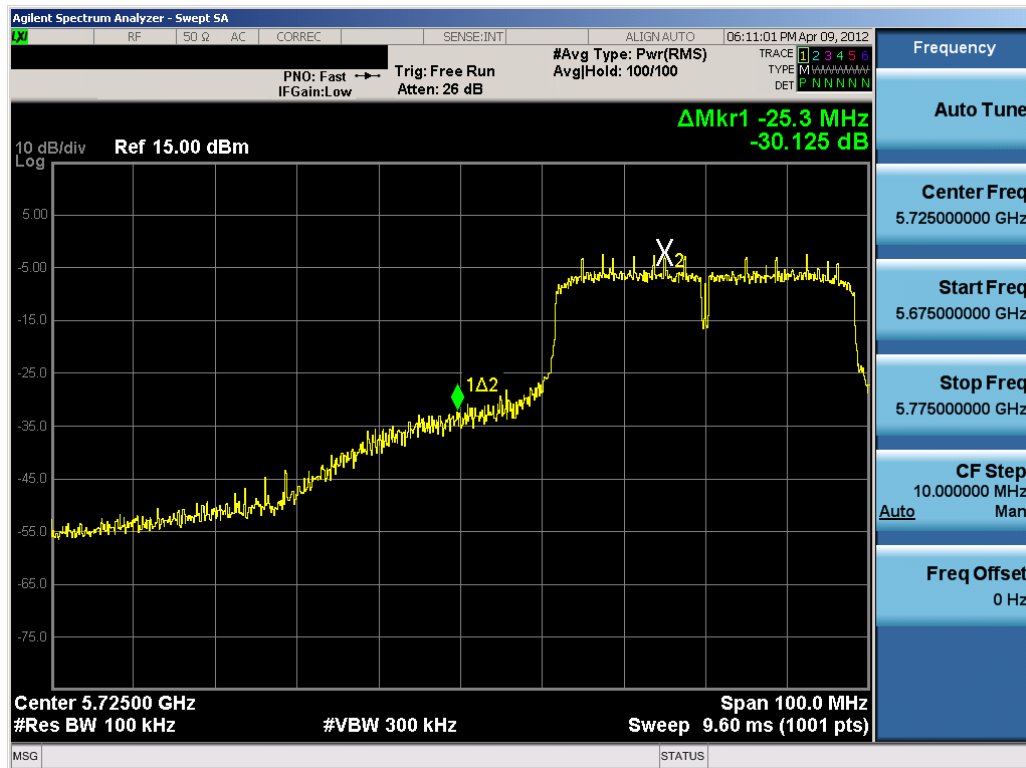
Plot 6-23. Band Edge Plot (802.11n (5.8GHz – 40MHz) – Ch. 151)
