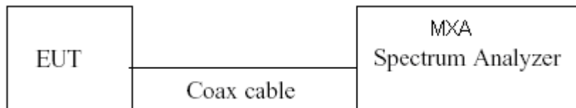
Figure 6-3. Test Instrument & Measurement Setup
