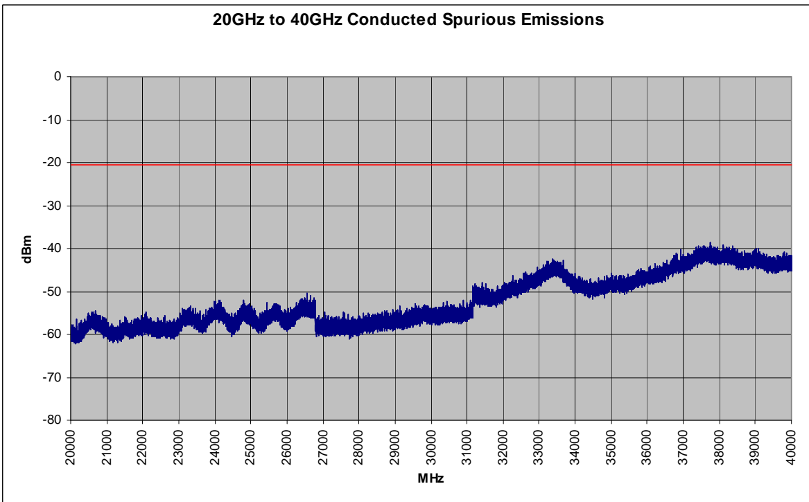
Plot 6-28. Conducted Spurious Plot (802.11a – Ch. 157)
