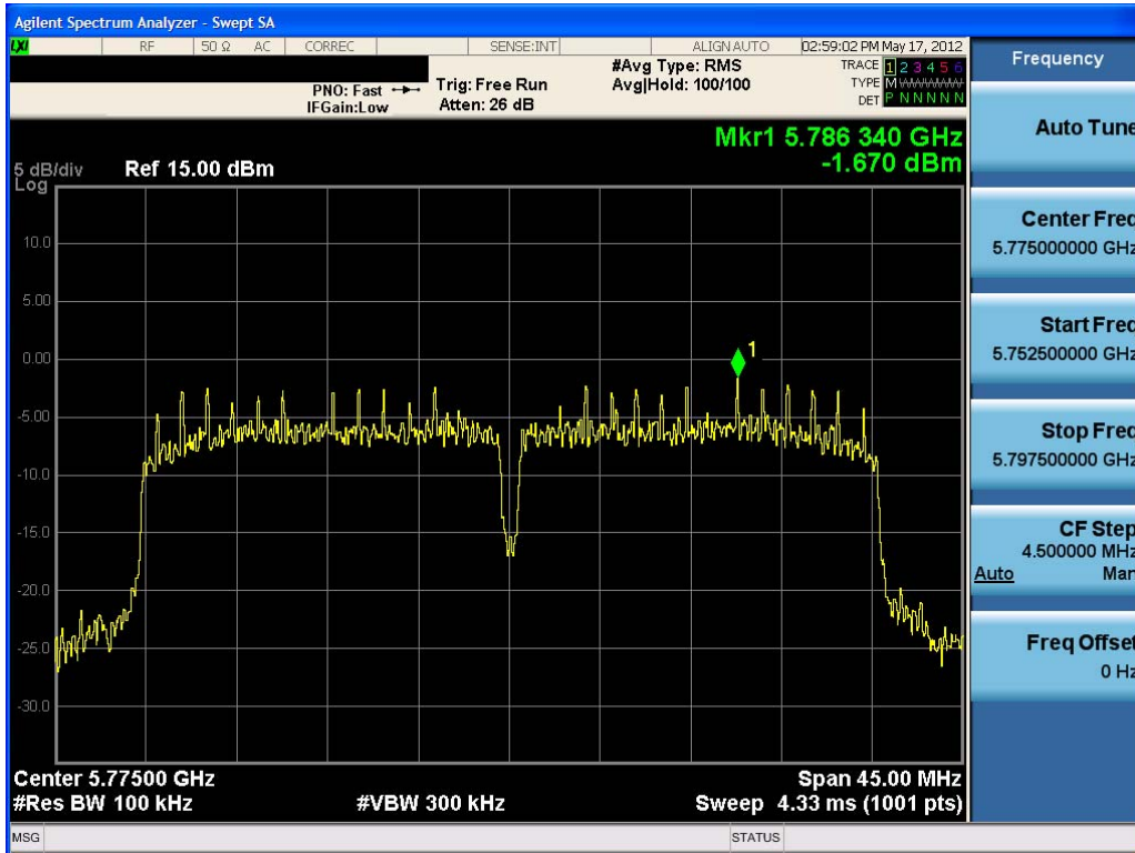
Plot 6-17. Power Spectral Density Plot (802.11n (5.8GHz – 40MHz BW) – Ch. 155)
