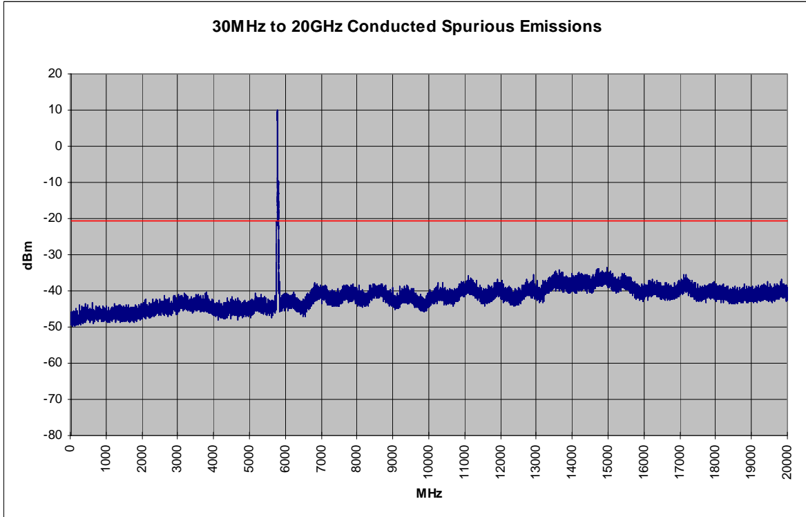
Plot 6-27. Conducted Spurious Plot (802.11a – Ch. 157)
