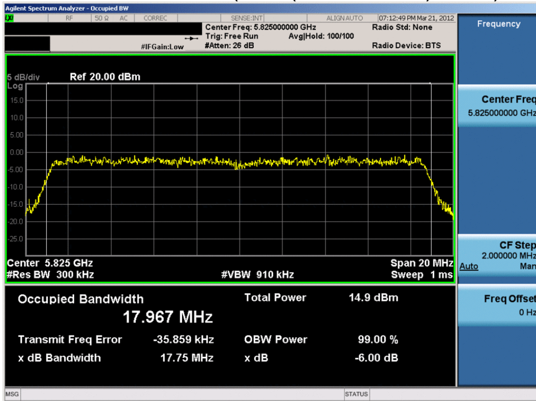
Plot 6-6. 6dB Bandwidth Plot (802.11n (5.8GHz – 20MHz BW) – Ch. 165)
