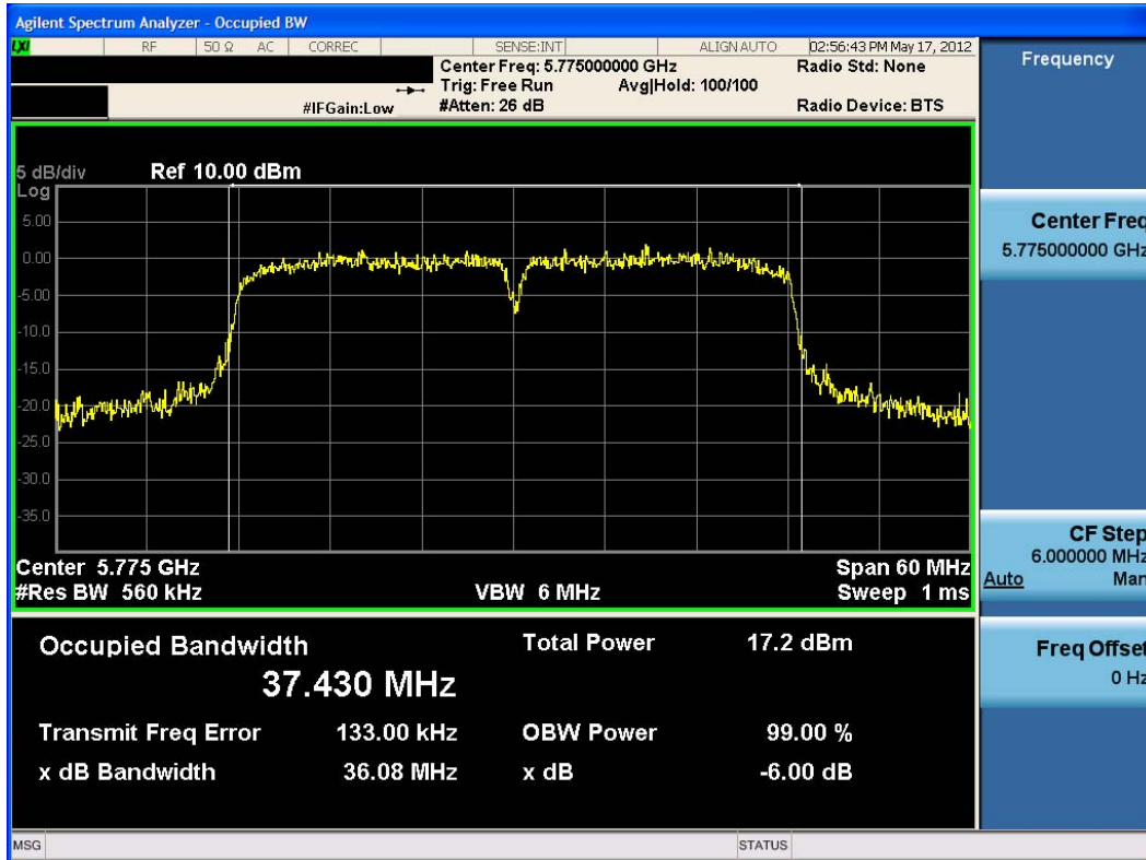
Plot 6-8. 6dB Bandwidth Plot (802.11n (5.8GHz – 40MHz BW) – Ch. 155)
