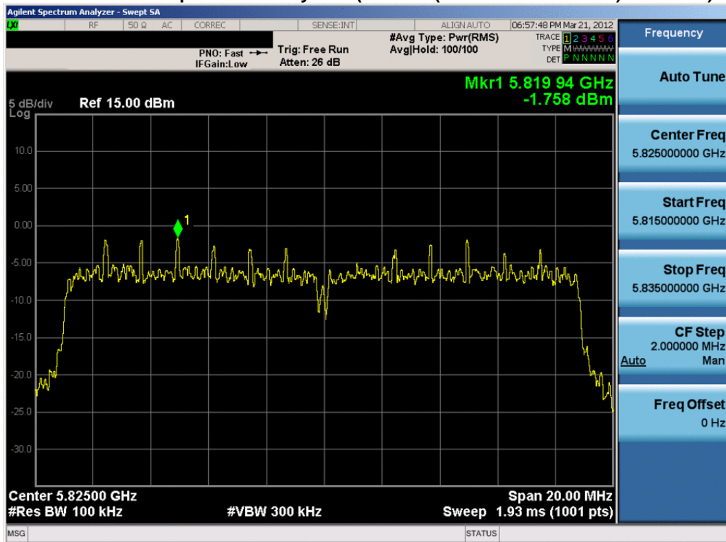
Plot 6-15. Power Spectral Density Plot (802.11n (5.8GHz – 20MHz BW) – Ch. 165)
