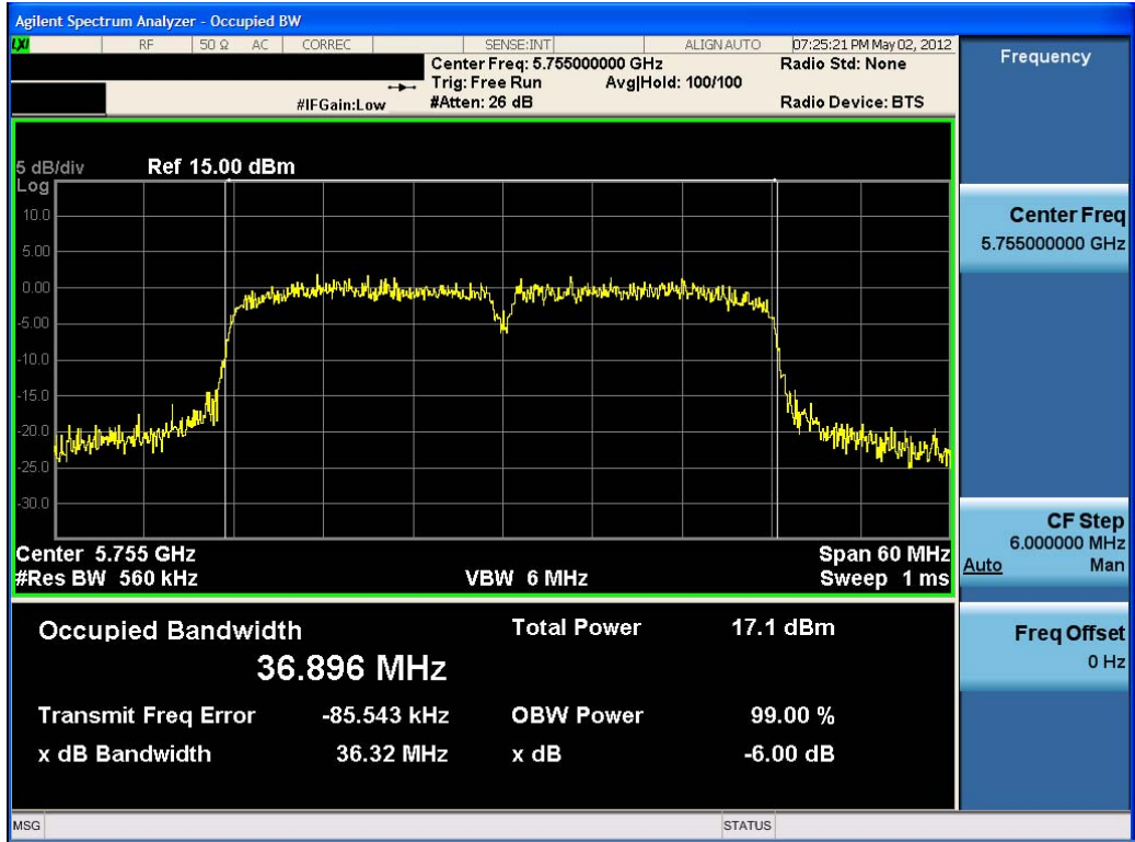
Plot 6-7. 6dB Bandwidth Plot (802.11n (5.8GHz – 40MHz BW) – Ch. 151)
