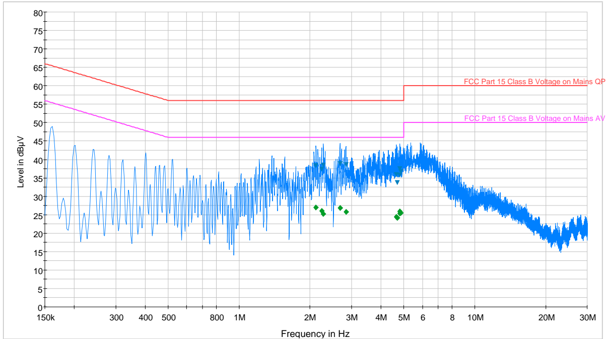
Plot 6-31. Line Conducted Plot with 802.11a
