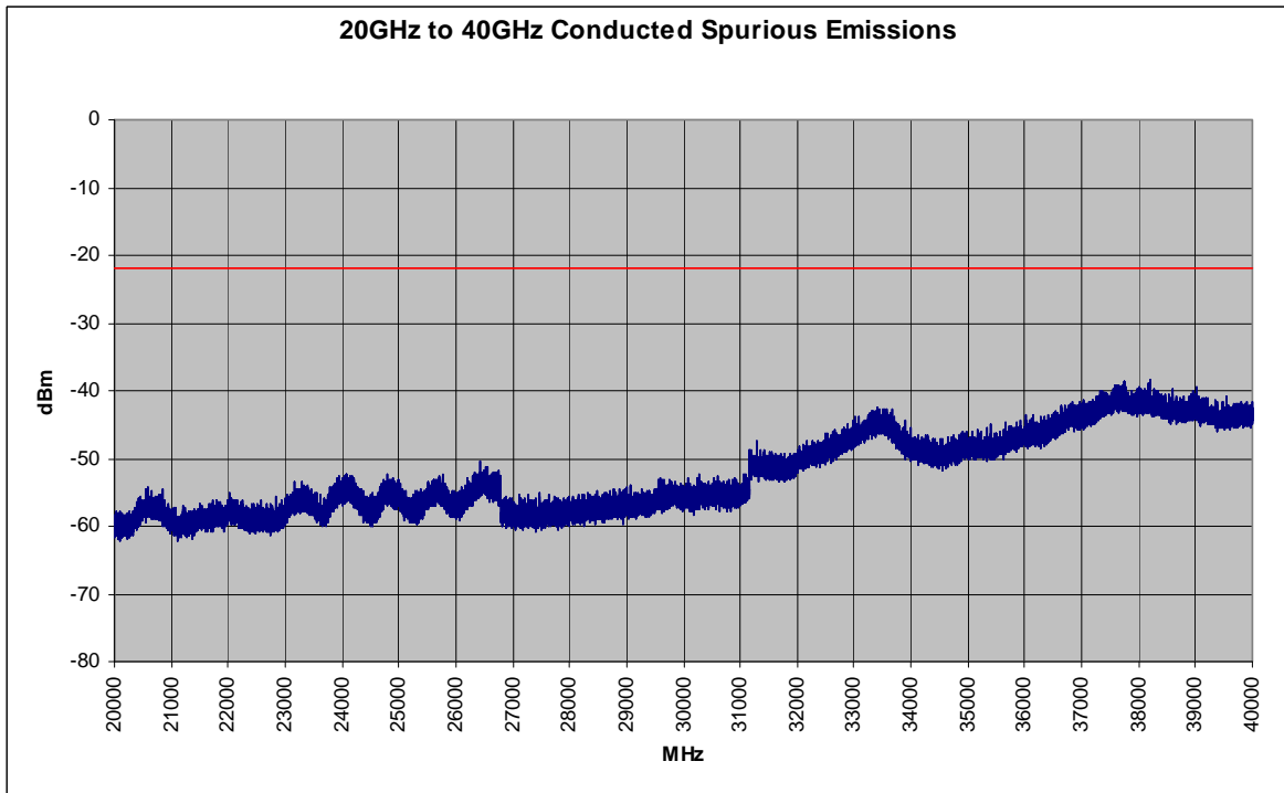
Plot 6-30. Conducted Spurious Plot (802.11a – Ch. 165)
