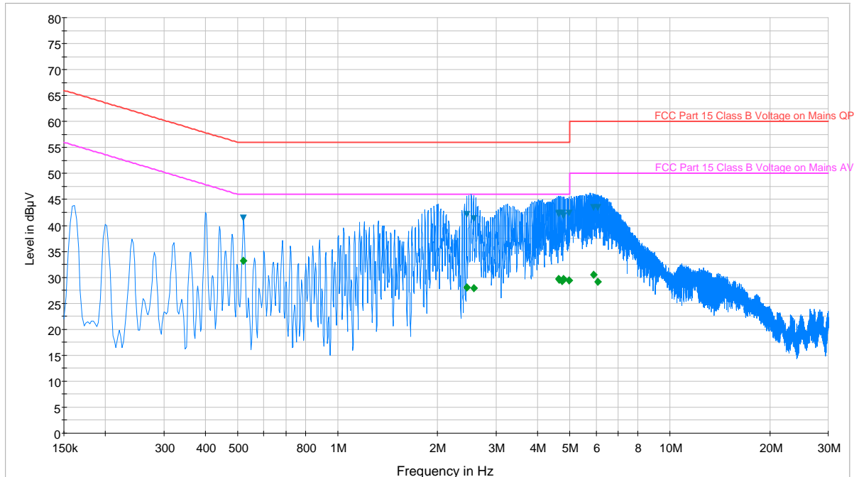
Plot 6-32. Line Conducted Plot with 802.11a
