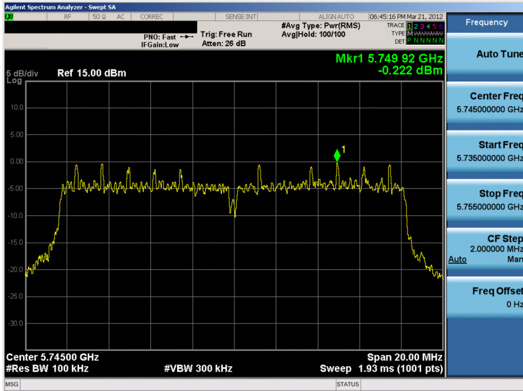
Plot 6-10. Power Spectral Density Plot (802.11a – Ch. 149)
