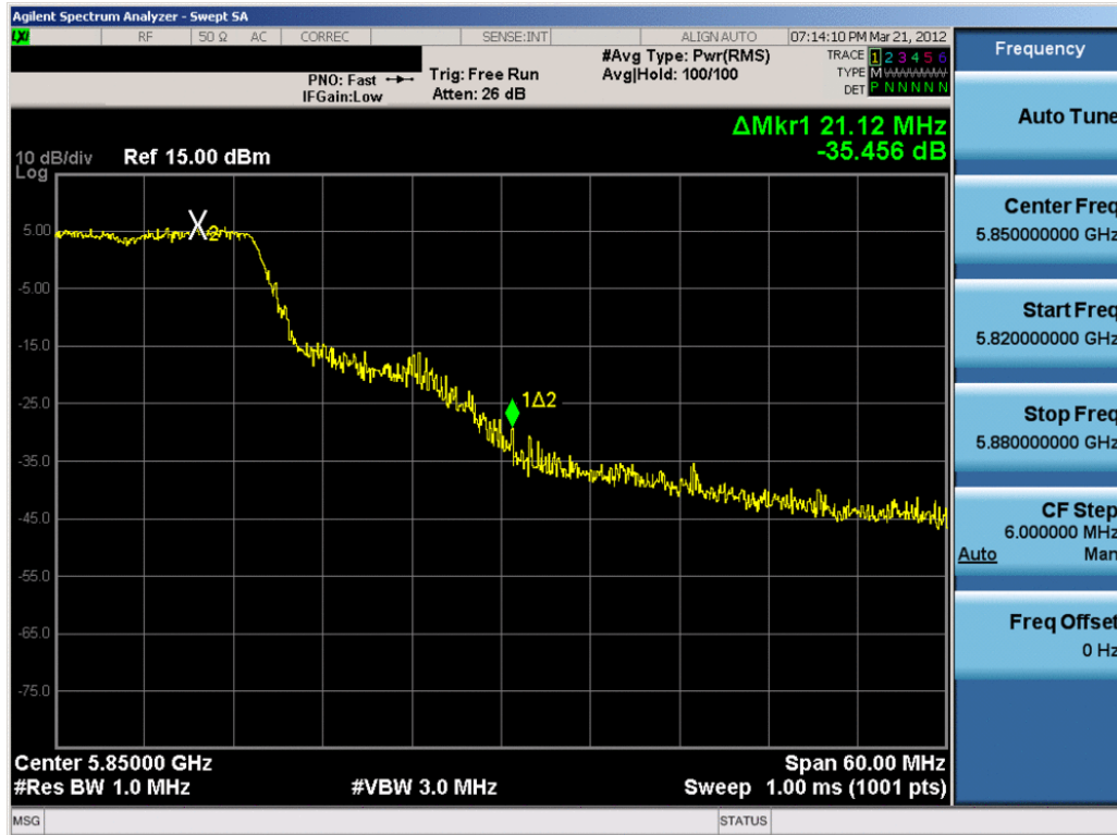
Plot 6-22. Band Edge Plot (802.11n (5.8GHz – 20MHz) – Ch. 165)
