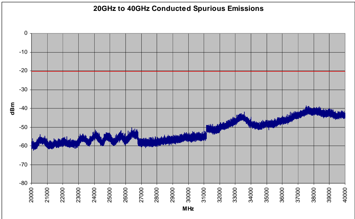
Plot 6-26. Conducted Spurious Plot (802.11a – Ch. 149)
