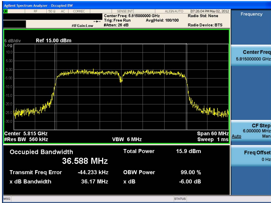
Plot 6-9. 6dB Bandwidth Plot (802.11n (5.8GHz – 40MHz BW) – Ch. 163)
