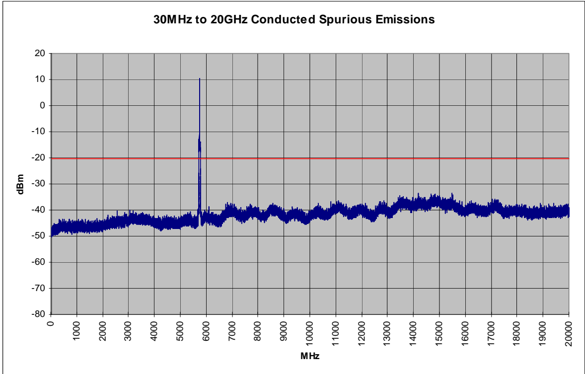
Plot 6-25. Conducted Spurious Plot (802.11a – Ch. 149)
