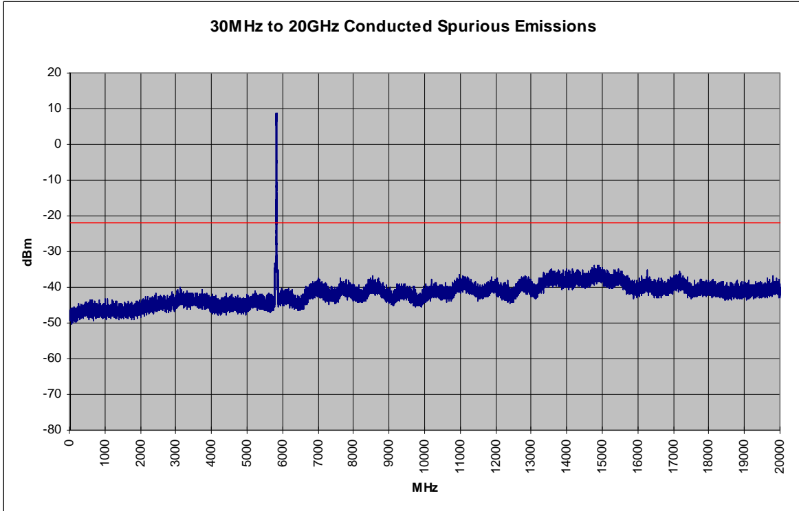
Plot 6-29. Conducted Spurious Plot (802.11a – Ch. 165)
