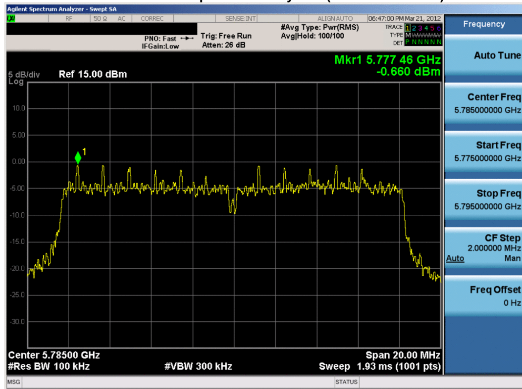
Plot 6-11. Power Spectral Density Plot (802.11a – Ch. 157)
