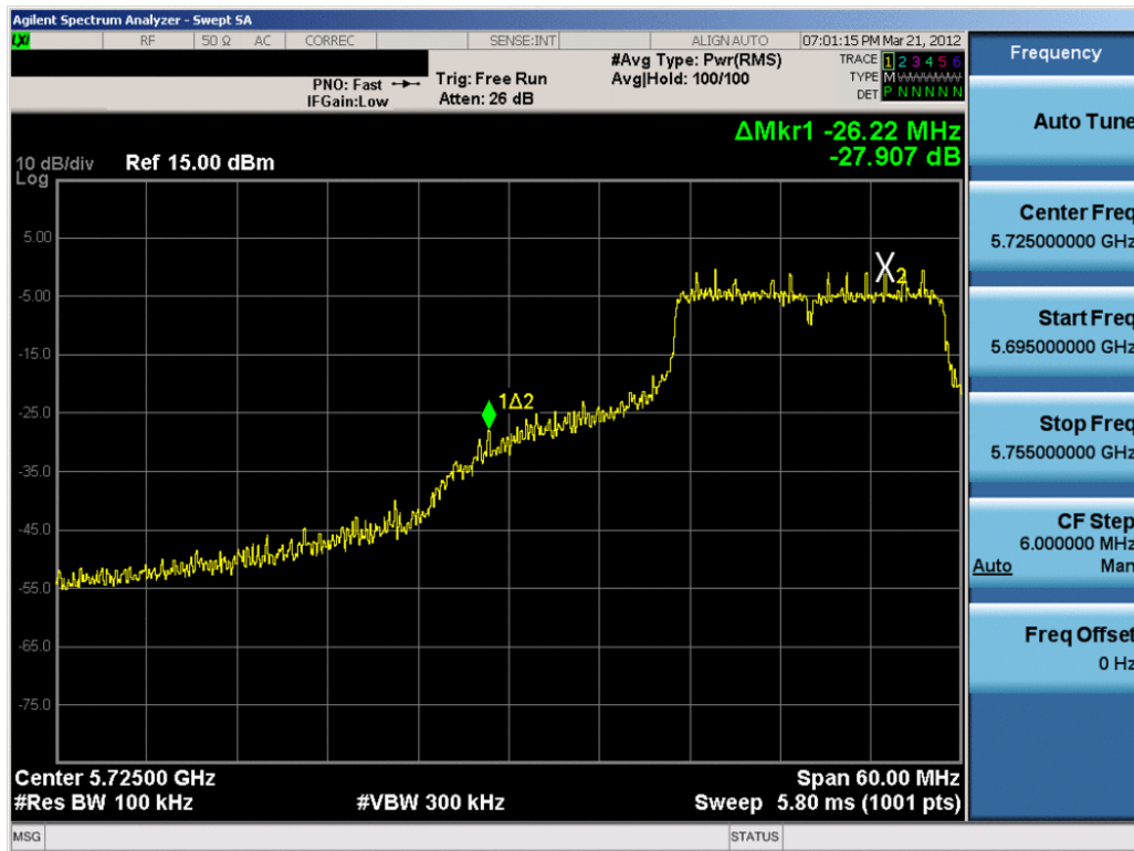
Plot 6-21. Band Edge Plot (802.11n (5.8GHz – 20MHz) – Ch. 149)
