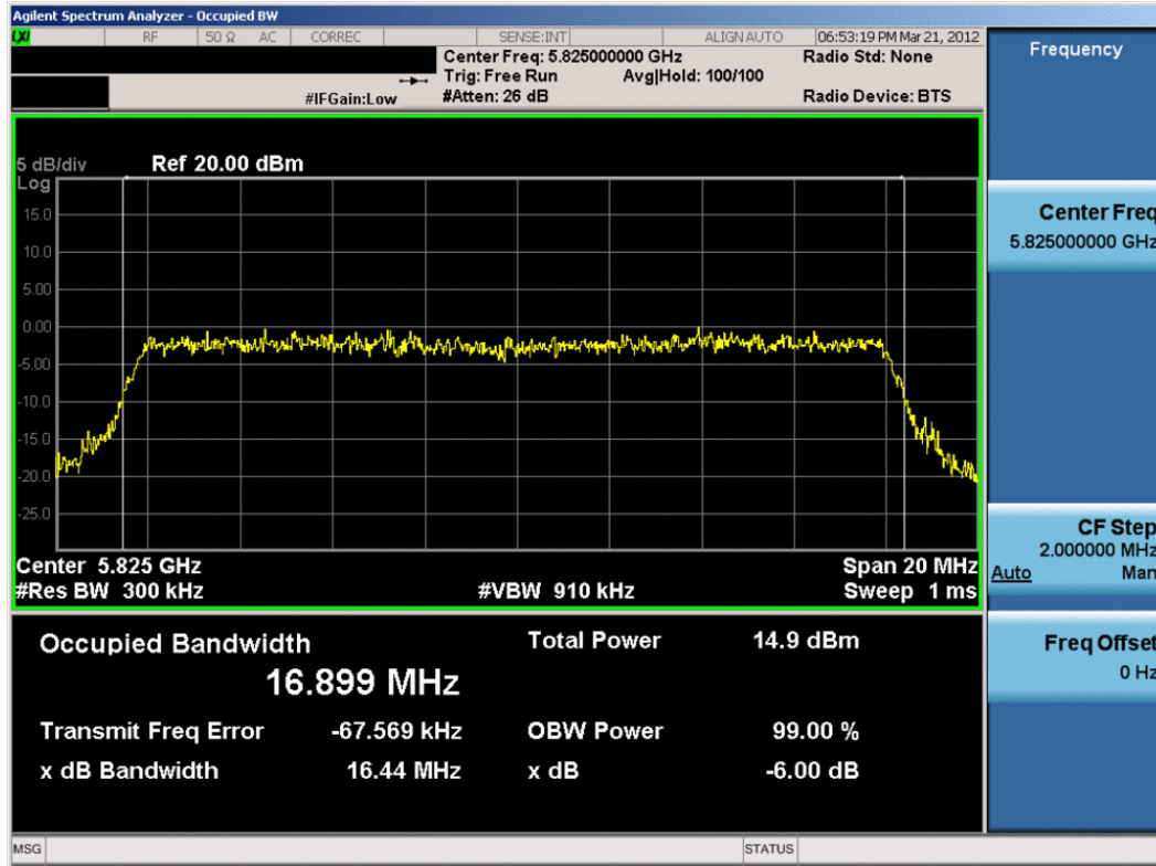
Plot 6-3. 6dB Bandwidth Plot (802.11a – Ch. 165)
