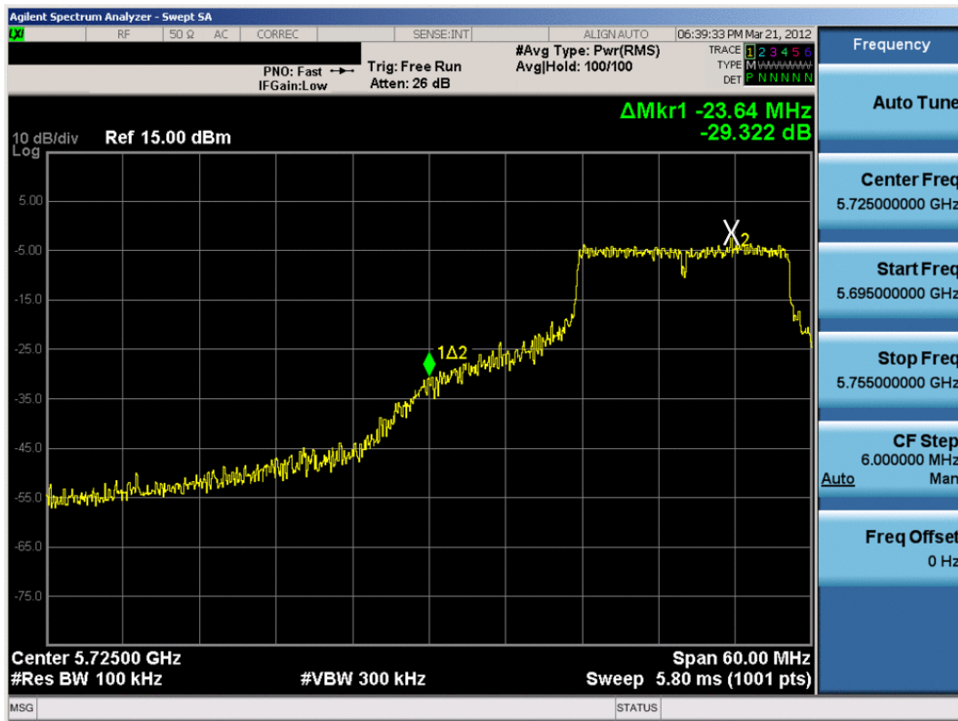
Plot 6-19. Band Edge Plot (802.11a – Ch. 149)
