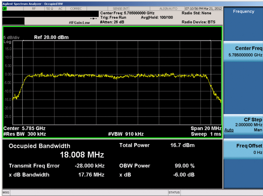
Plot 6-5. 6dB Bandwidth Plot (802.11n (5.8GHz – 20MHz BW) – Ch. 157)
