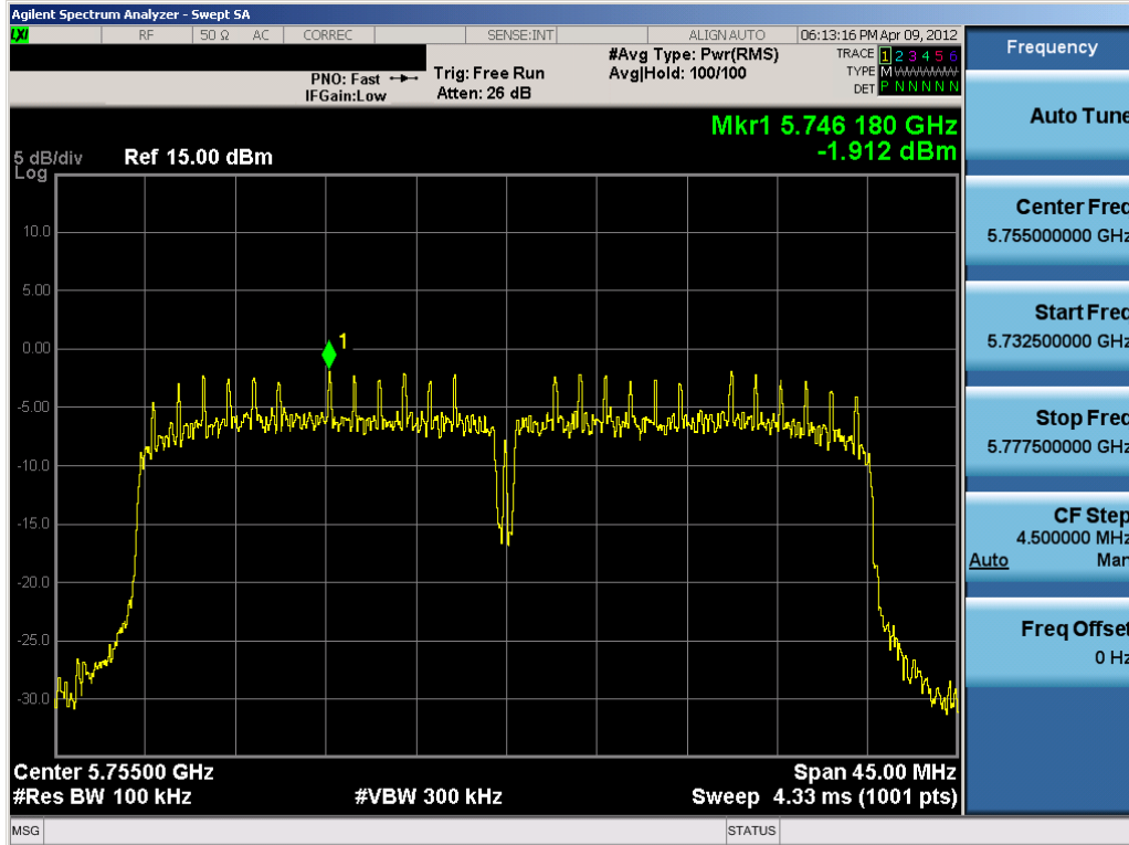
Plot 6-16. Power Spectral Density Plot (802.11n (5.8GHz – 40MHz BW) – Ch. 151)
