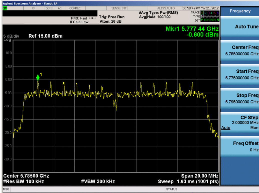
Plot 6-14. Power Spectral Density Plot (802.11n (5.8GHz – 20MHz BW) – Ch. 157)
