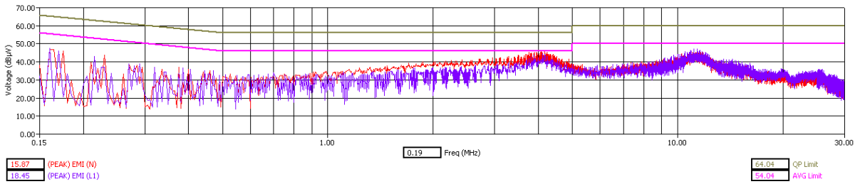
WLAN Channel 11 - Tx Mode - Peak Detector
