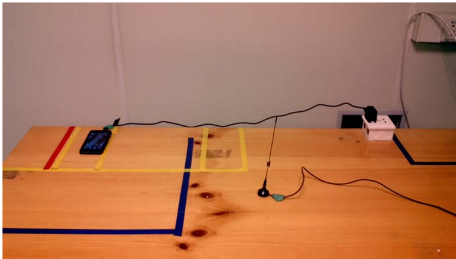
Radiated Emissions
