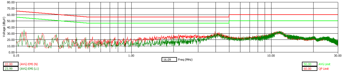
Bluetooth – Hopping - Tx Mode – AVG Detector
