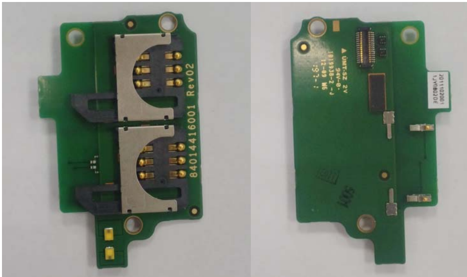
Daughter Board Back
