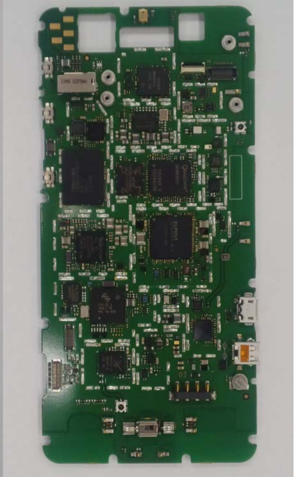
Main Board Bottom Without Shields
