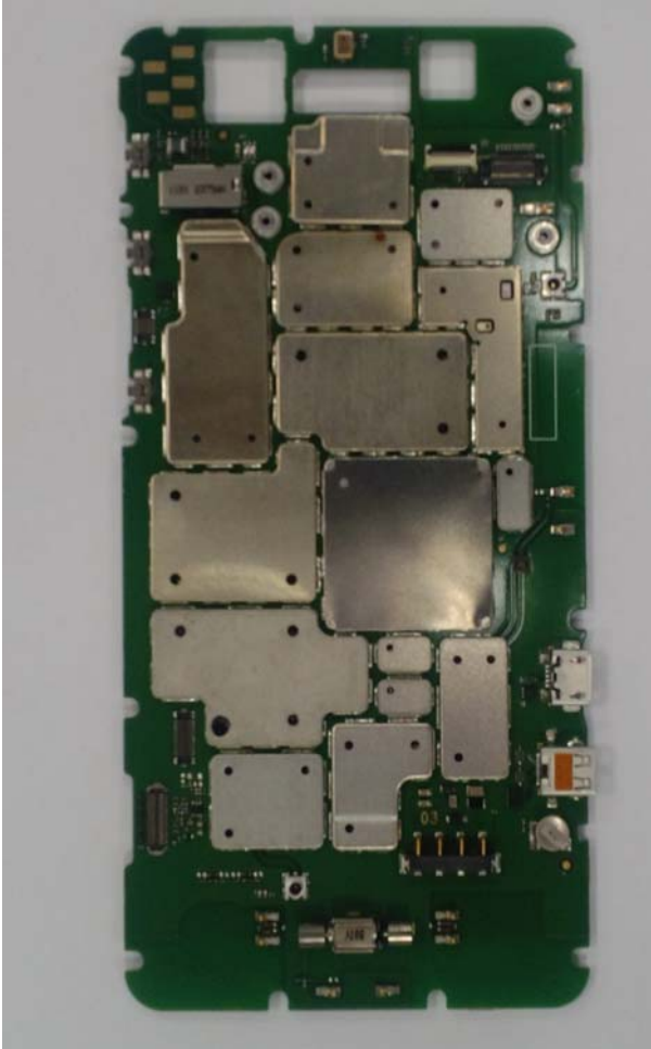
Main Board Bottom With shields
