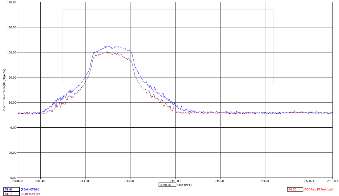
Low Band Edge Y Orientation Peak Detector
