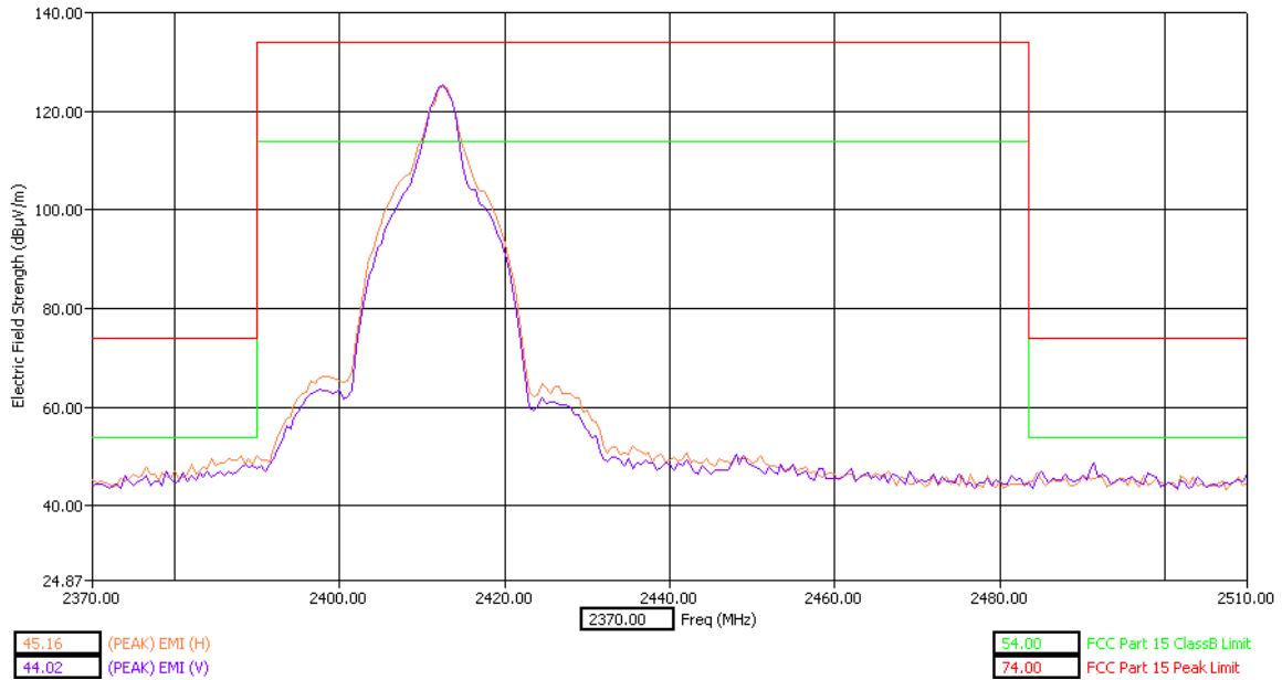
Low Band Edge Y Orientation Peak Detector
