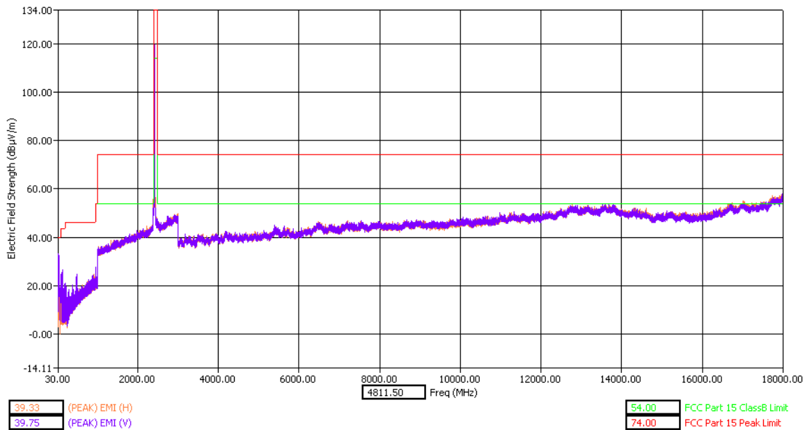
Low Channel Dual Polarization Y
