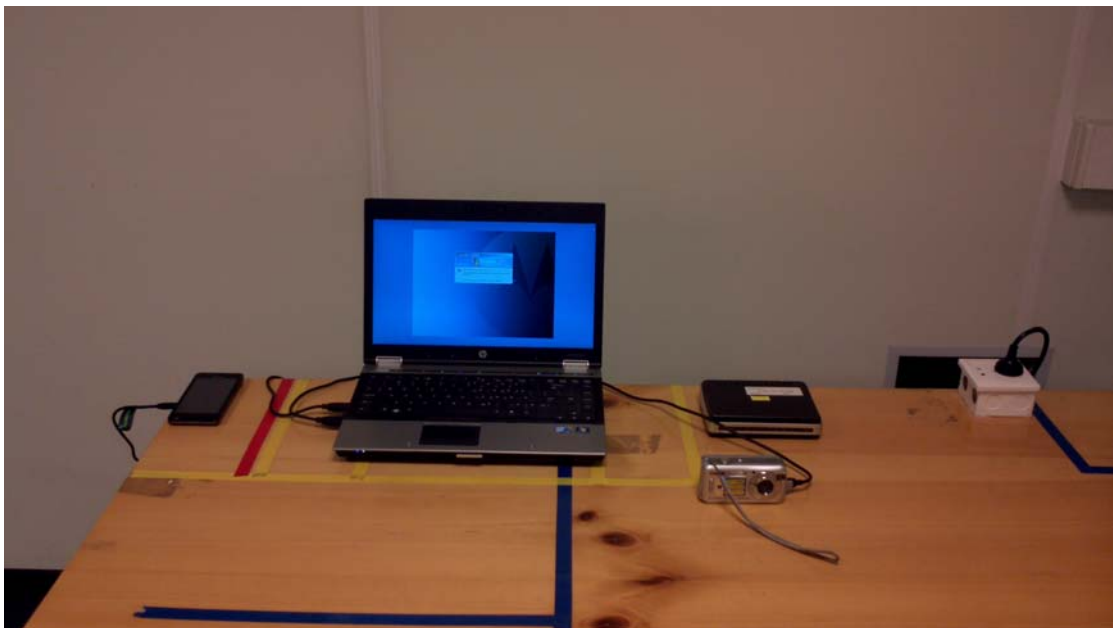
AC Line Conducted Emissions – Computer Peripheral
