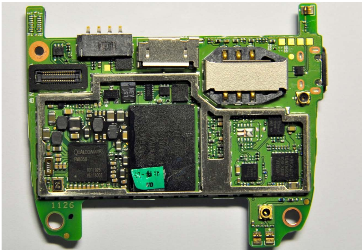
Sub Board-Top (Shielding removed)
