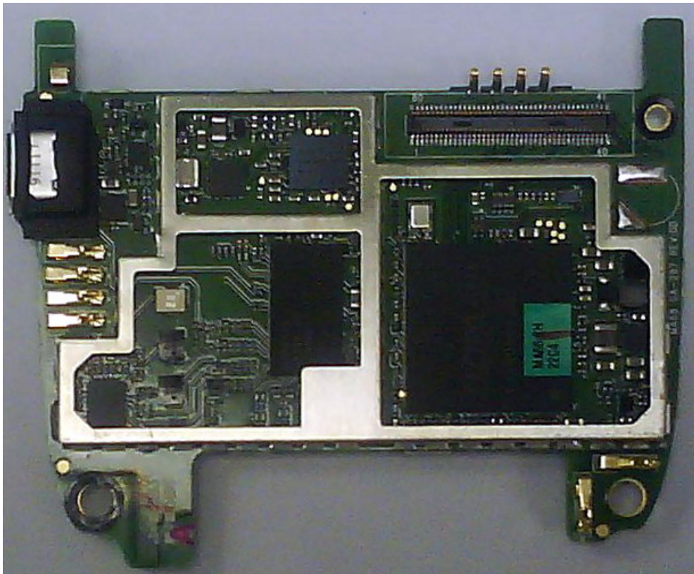
Sub Board-Bottom (Shielding removed)
