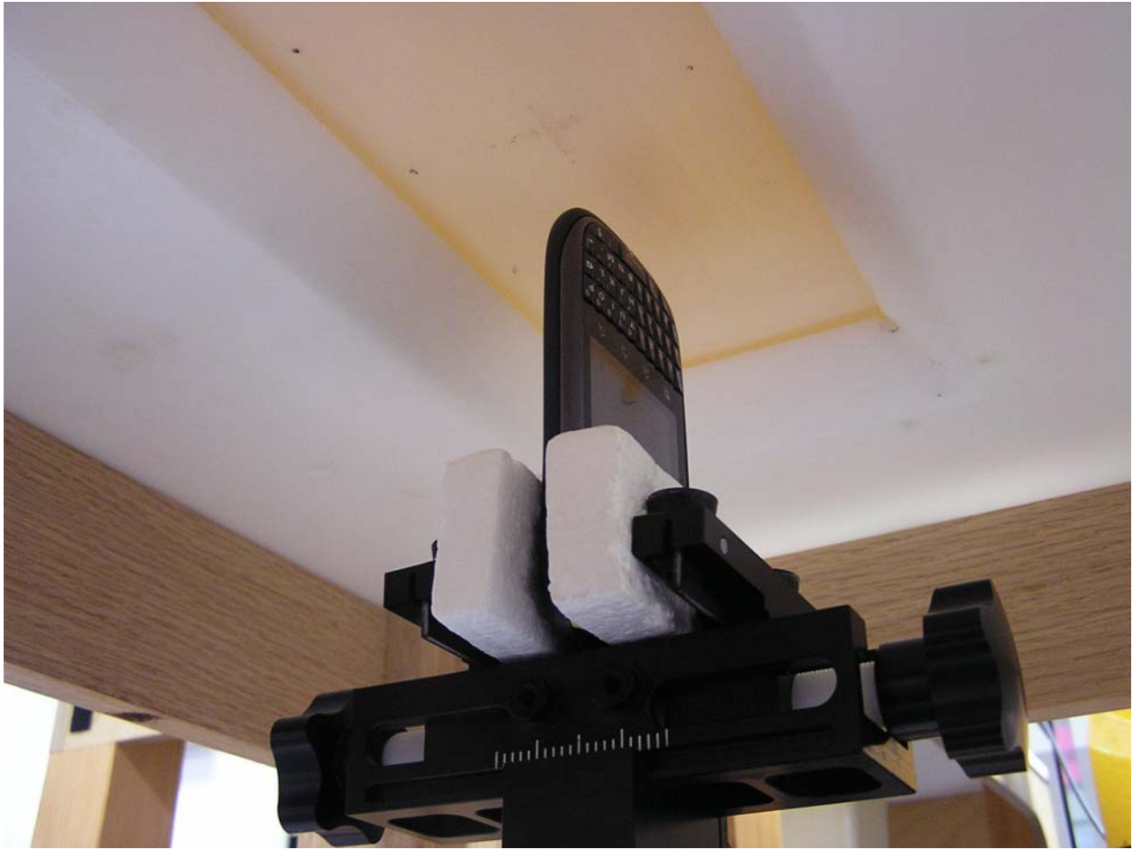
Figure 9: 10mm Separation from Bottom Edge Position
