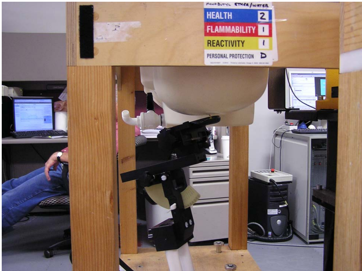
Figure 6: Tilt Position, Top of Head of Phantom
