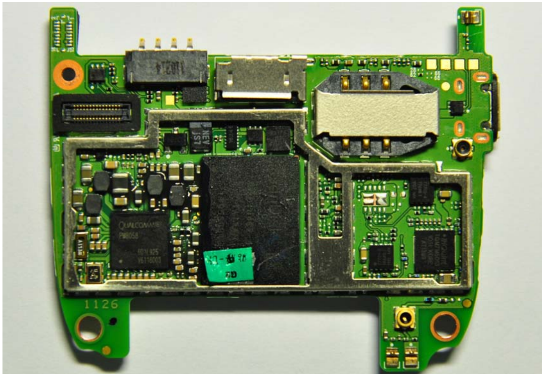
Sub Board-Bottom (Shielding removed)
