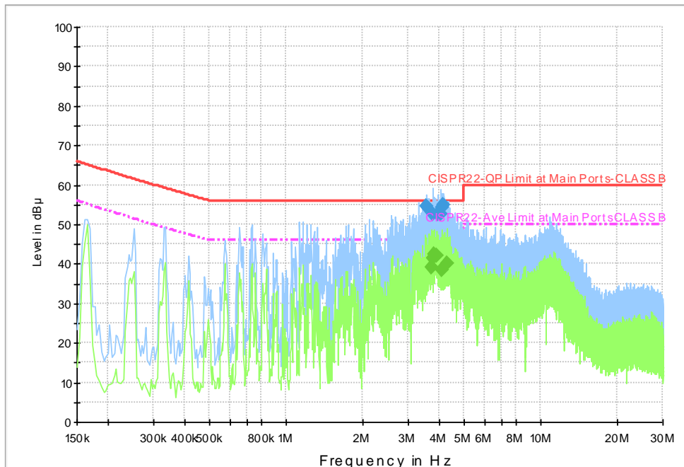
MORLAB-CE-ENV216Auto Test-L
