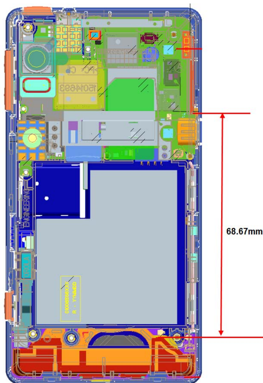
Figure 2: Antenna Separation
