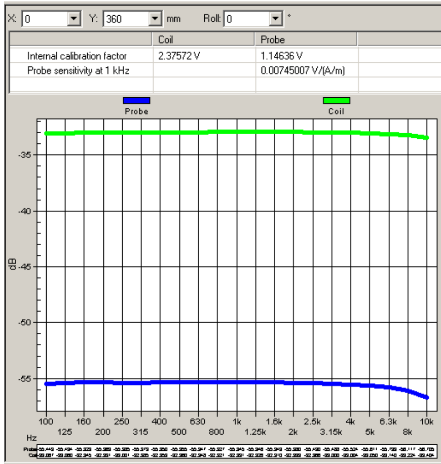
Graph 1: Frequency Response measured in AMCC
