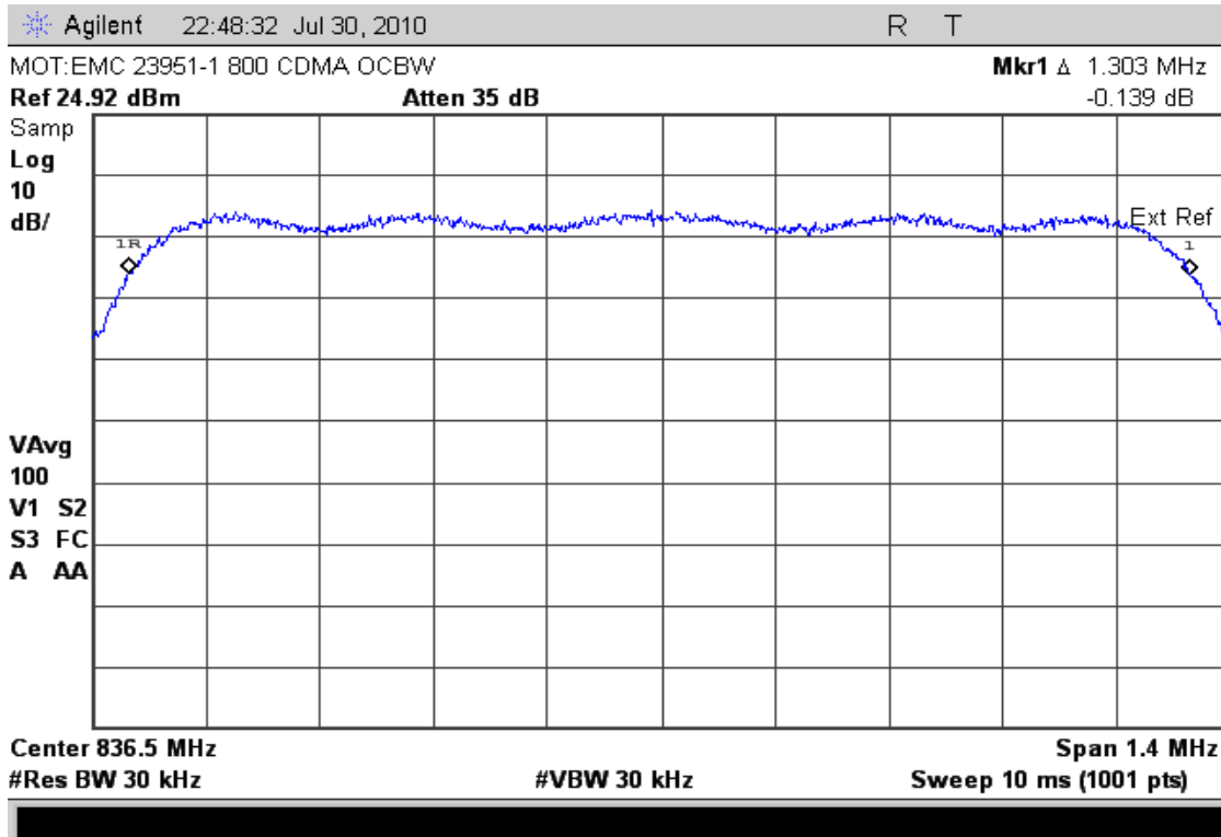
CDMA 800 – Occupied Bandwidth – Channel 384 (836.52MHz)
