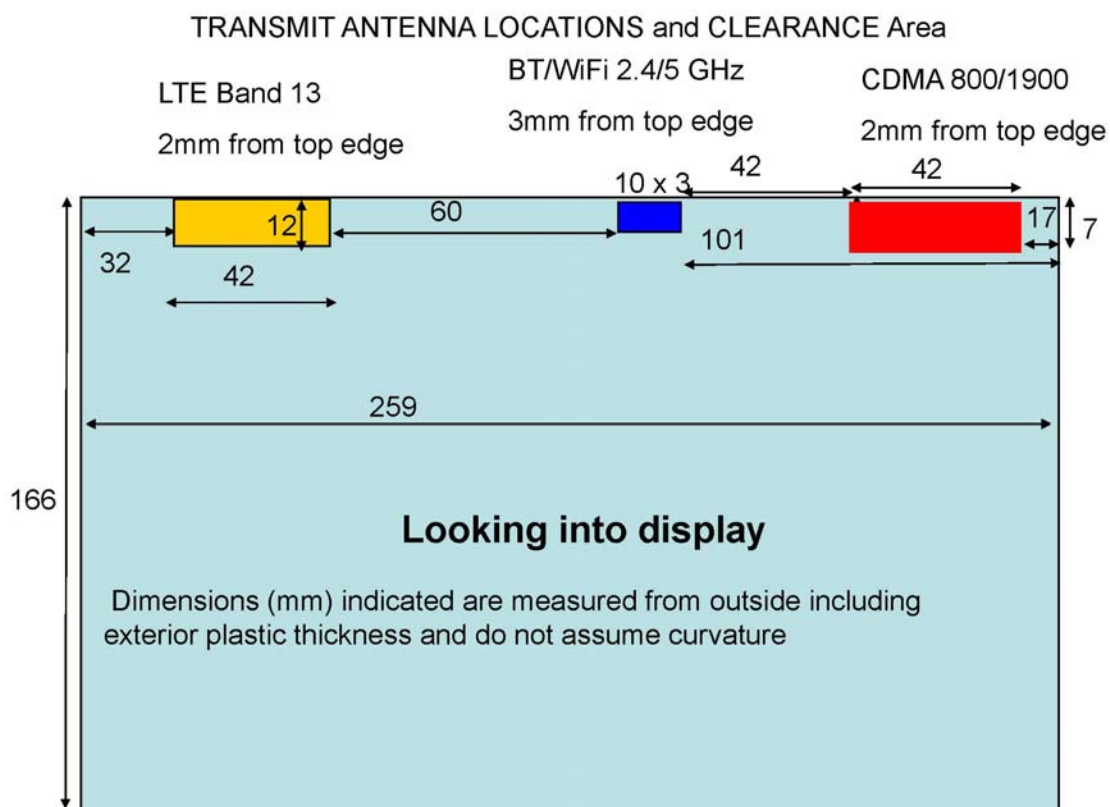
Figure 5: Device Dimensions and Antenna Separation Distances
