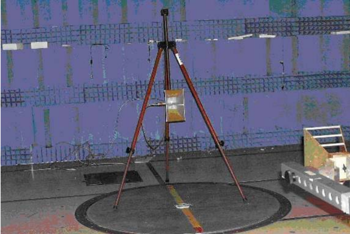
Antenna - Substitution
