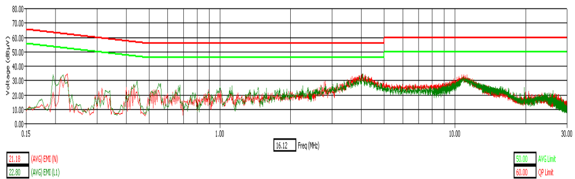
WLAN Channel 161 - Tx Mode - AVG Detector
