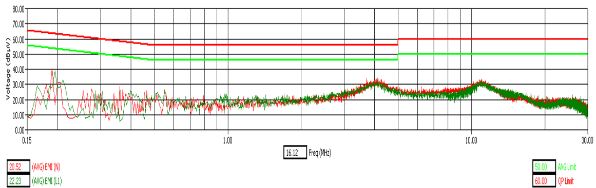
WLAN Channel 157 - Tx Mode - AVG Detector
