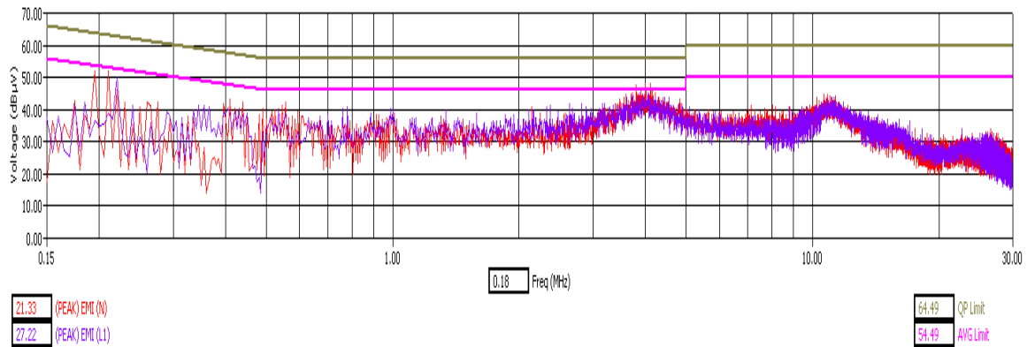
WLAN Channel 149 - Tx Mode -Peak Detector
