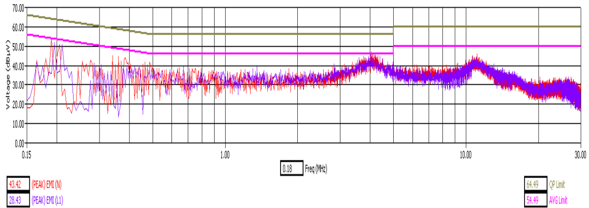
WLAN Channel 157 - Tx Mode - Peak Detector
