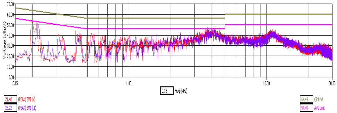
WLAN Channel 157 - Tx Mode - Peak Detector
