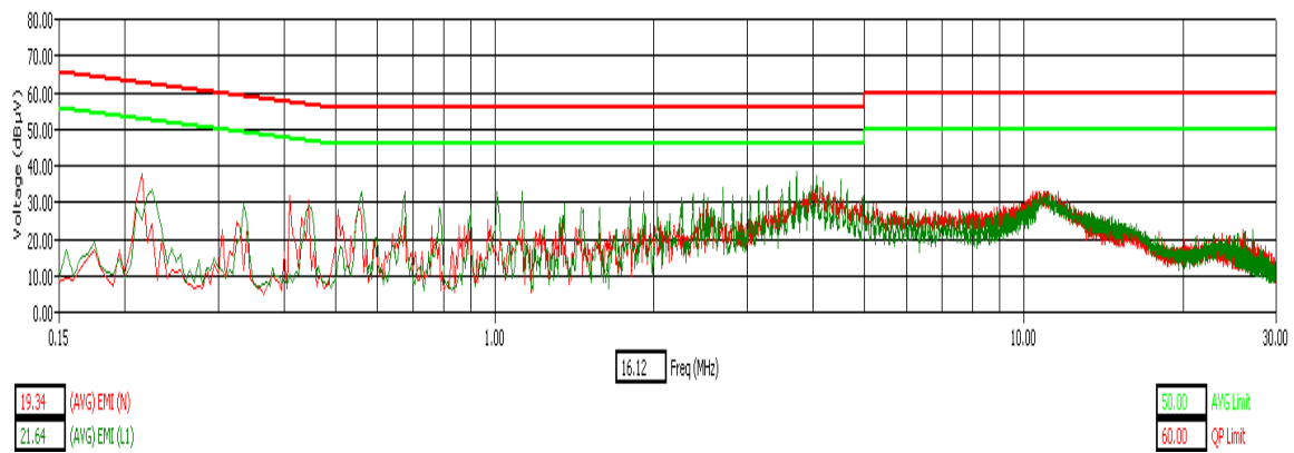
WLAN Channel 161 - Tx Mode - AVG Detector
