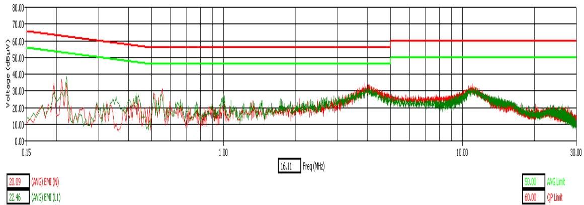
WLAN Channel 149 - Tx Mode - AVG Detector
