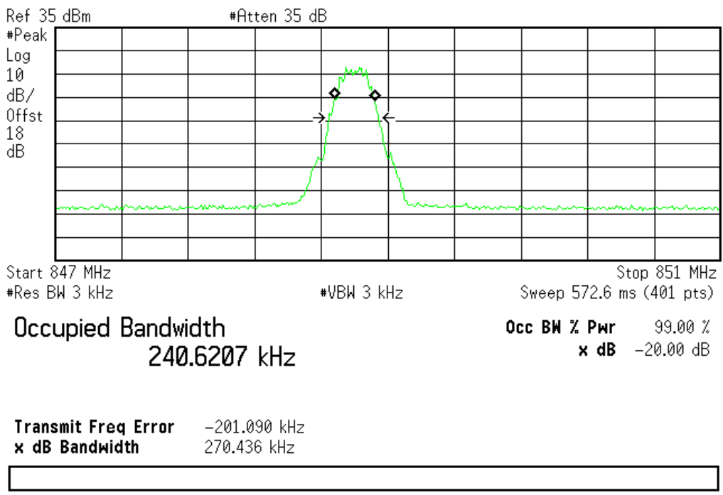
(Plot C3.2: EGPRS 850MHz Channel = 251)
