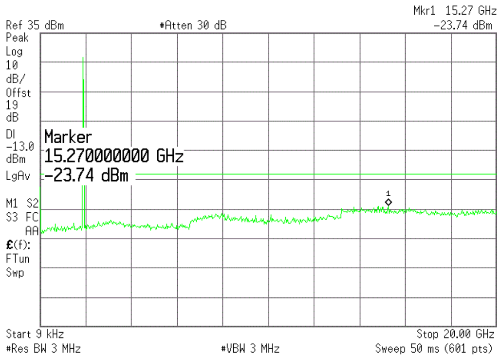
(Plot Q4.:EGPRS 1900MHz Channel = 661, 9KHz to 20GHz)
