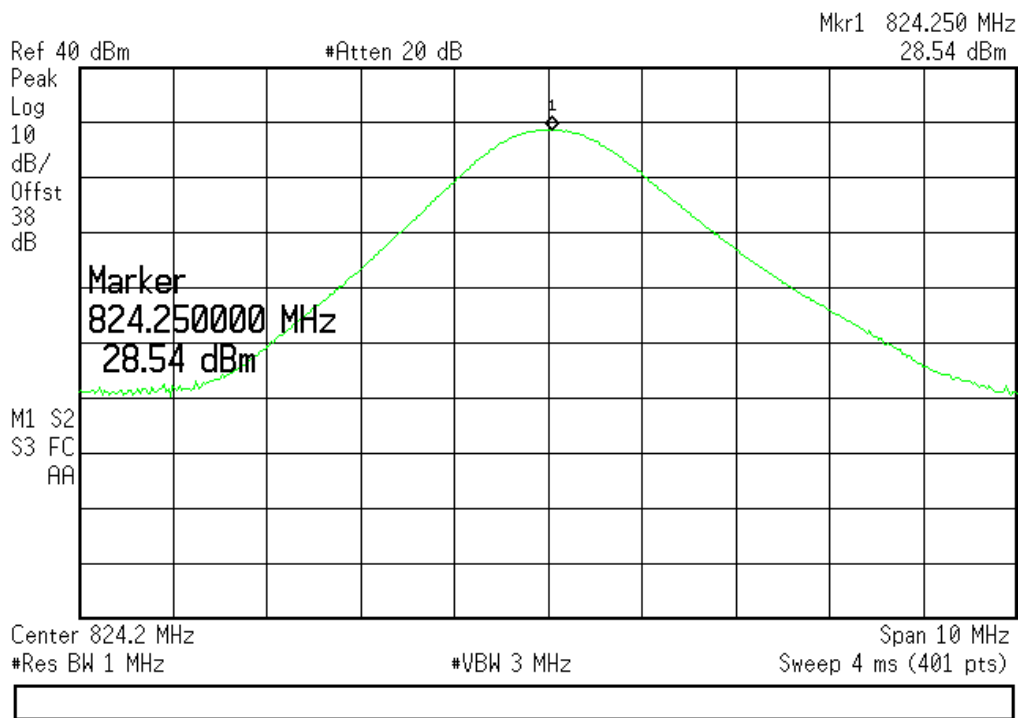
(Plot A6:GSM 850MHz Channel = 128)
