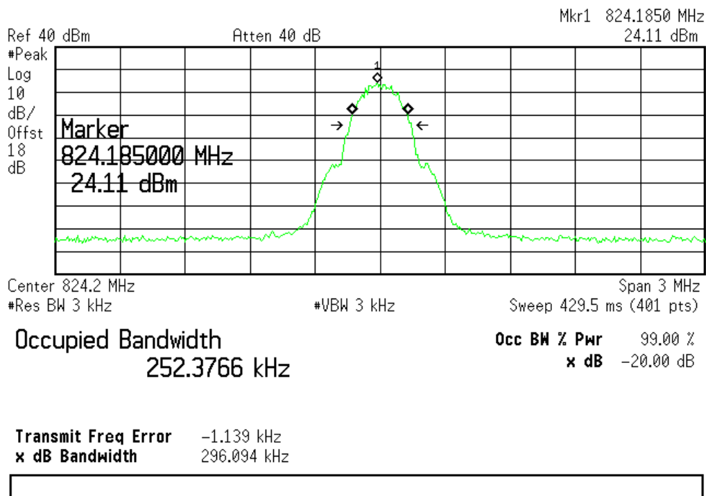
(Plot A3: GSM 850MHz Channel = 128)
