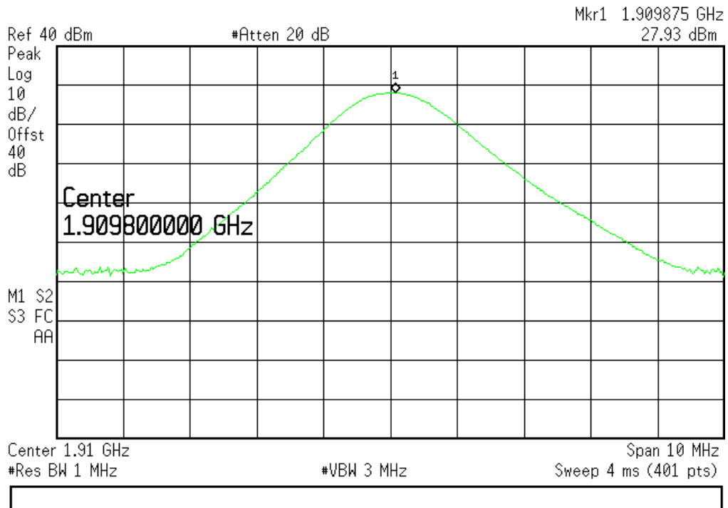
(Plot F6:GSM 1900MHz Channel = 810)
