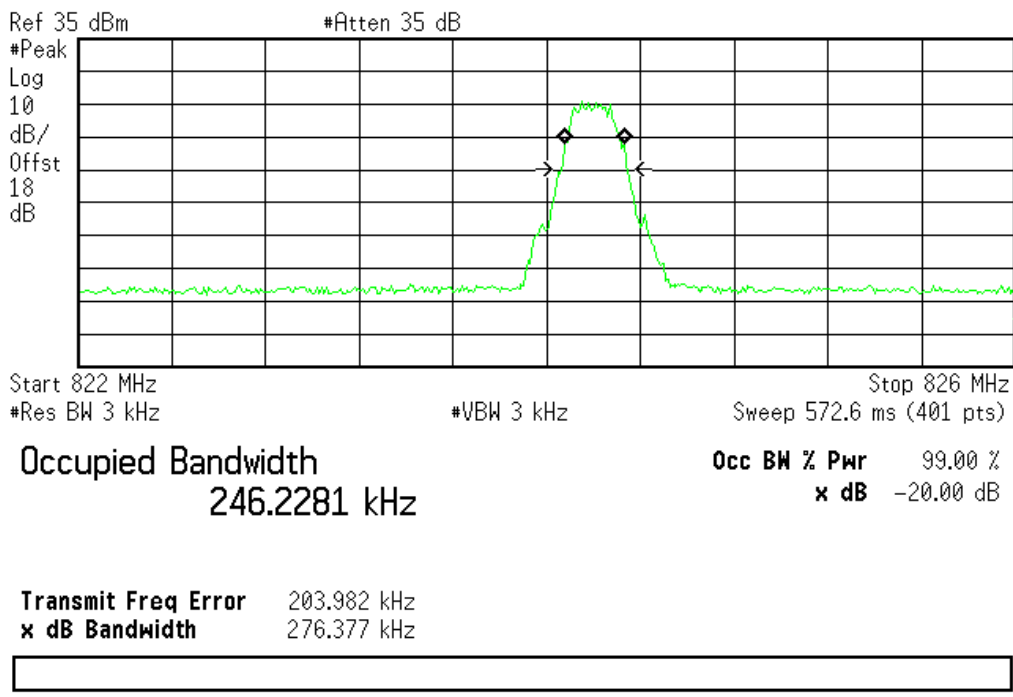
(Plot A3.2: EGPRS 850MHz Channel = 128)
