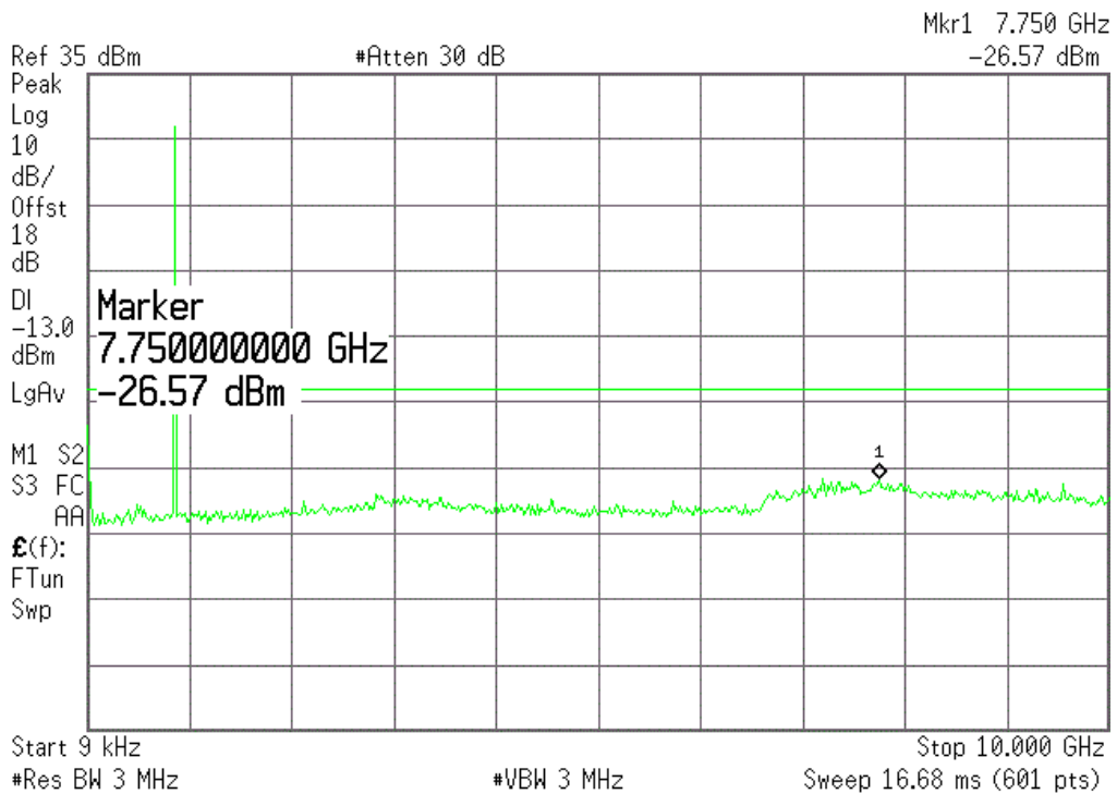
(Plot M4.:EGPRS 850MHz Channel = 128, 9KHz to 10GHz)
