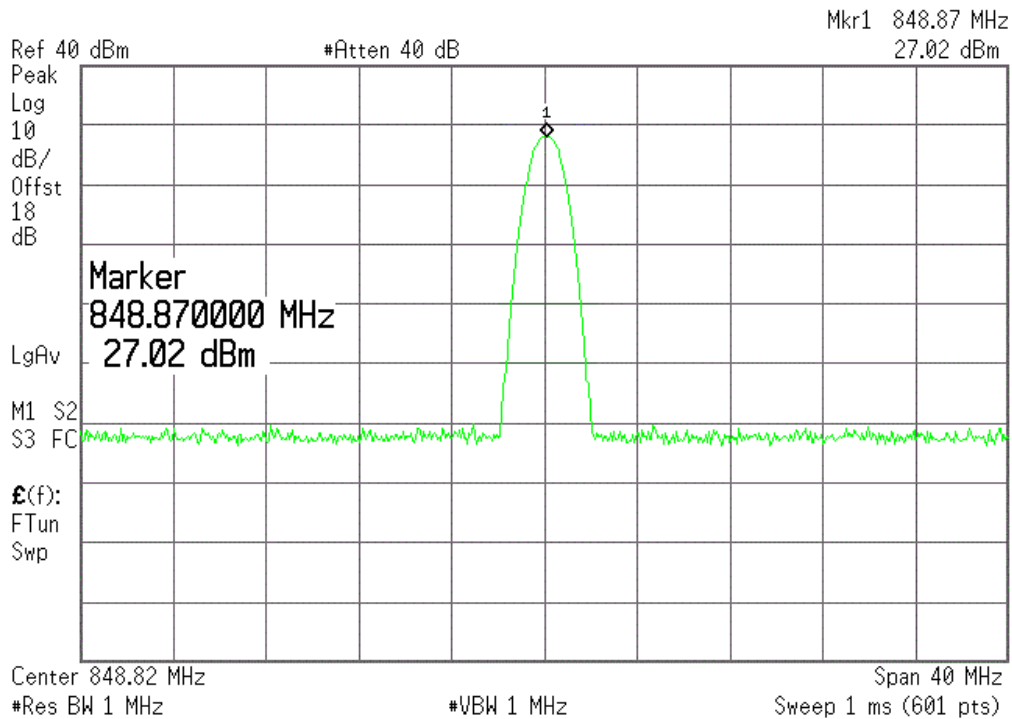
(Plot J1: EGPRS 850MHz Channel = 251)
