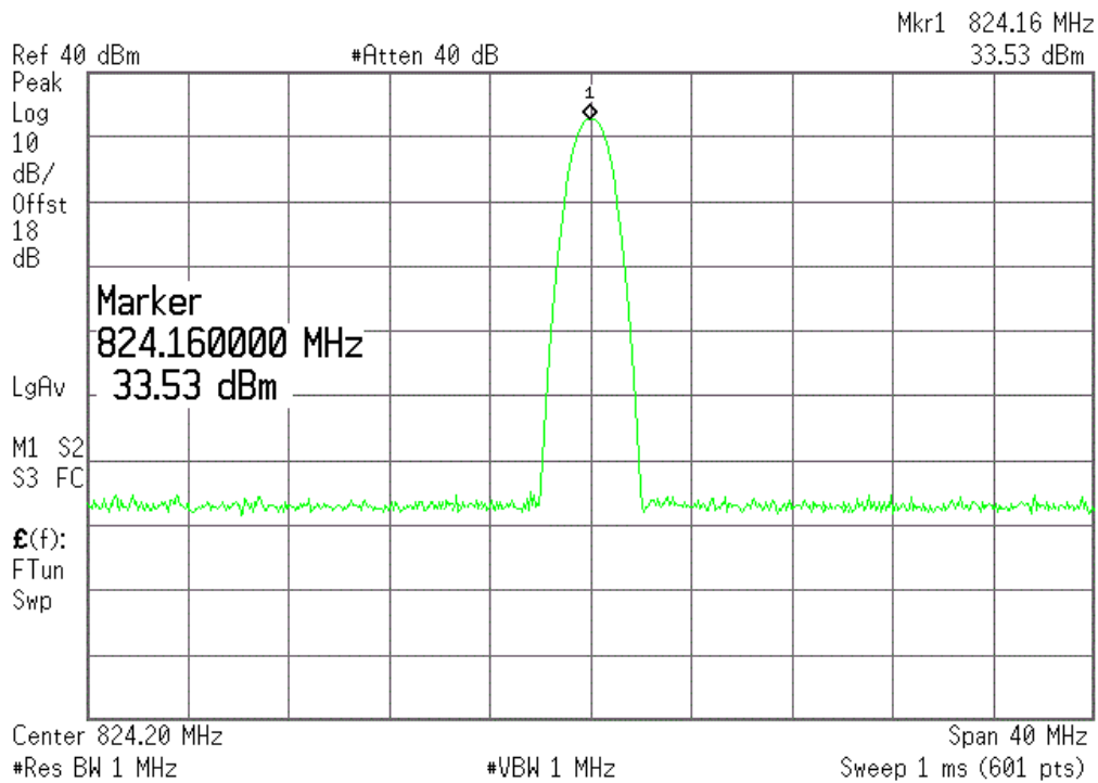
(Plot G2:GPRS 850MHz Channel = 128)
