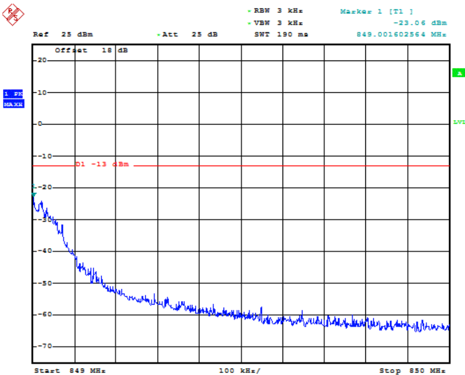
(Plot J5: EGPRS 850MHz Channel = 251)
