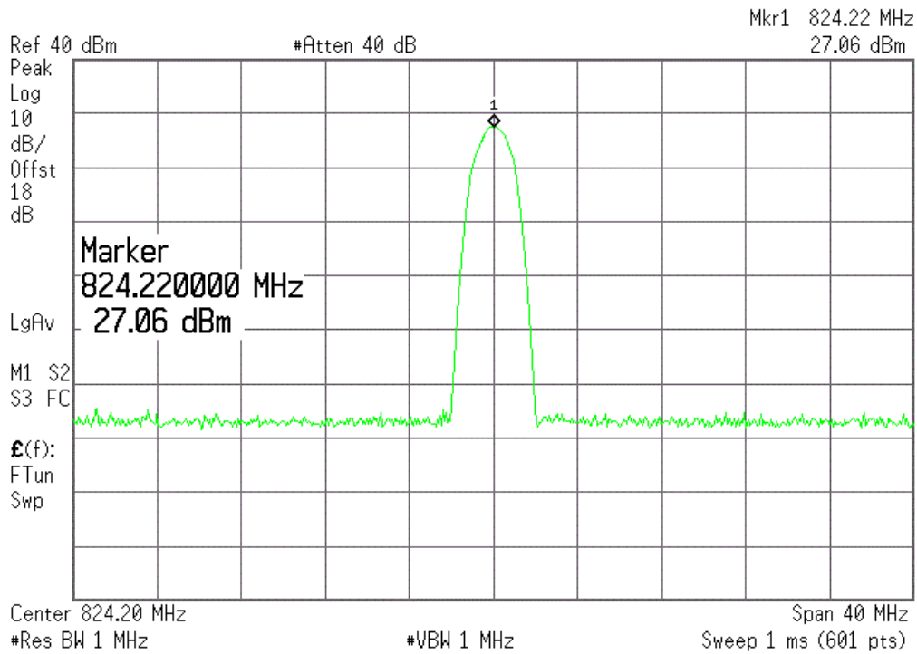
(Plot I1: EGPRS 850MHz Channel = 128)
