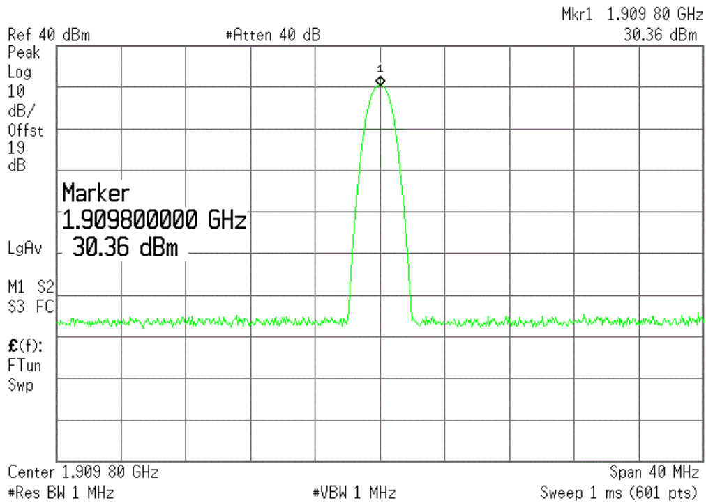
(Plot L2: GPRS 1900MHz Channel = 810)
