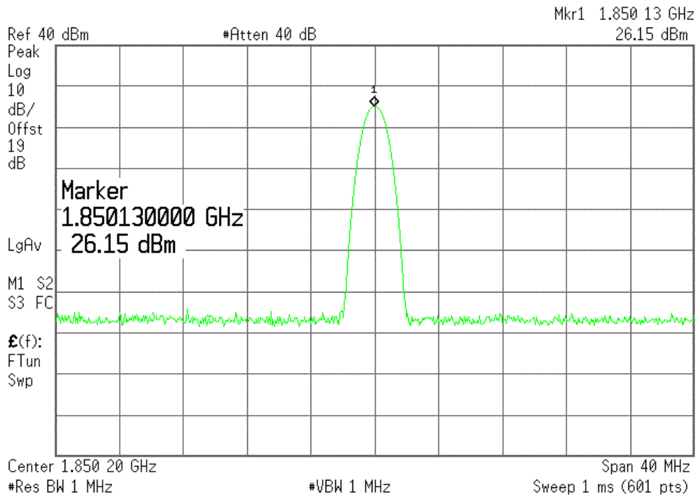
(Plot K1: EGPRS 1900MHz Channel = 512)
