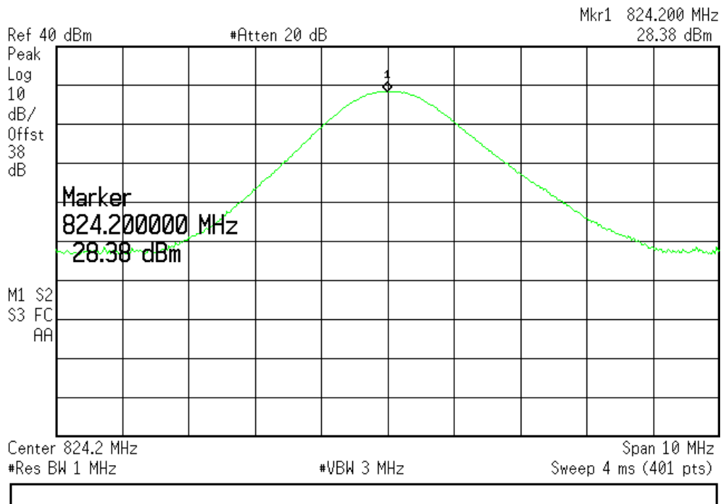
(Plot A6.1:GPRS 850MHz Channel = 128)
