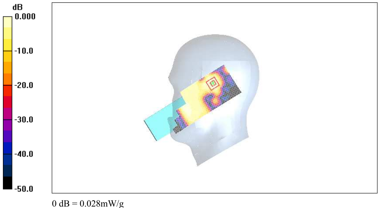
Fig.30 2450MHz CH1
