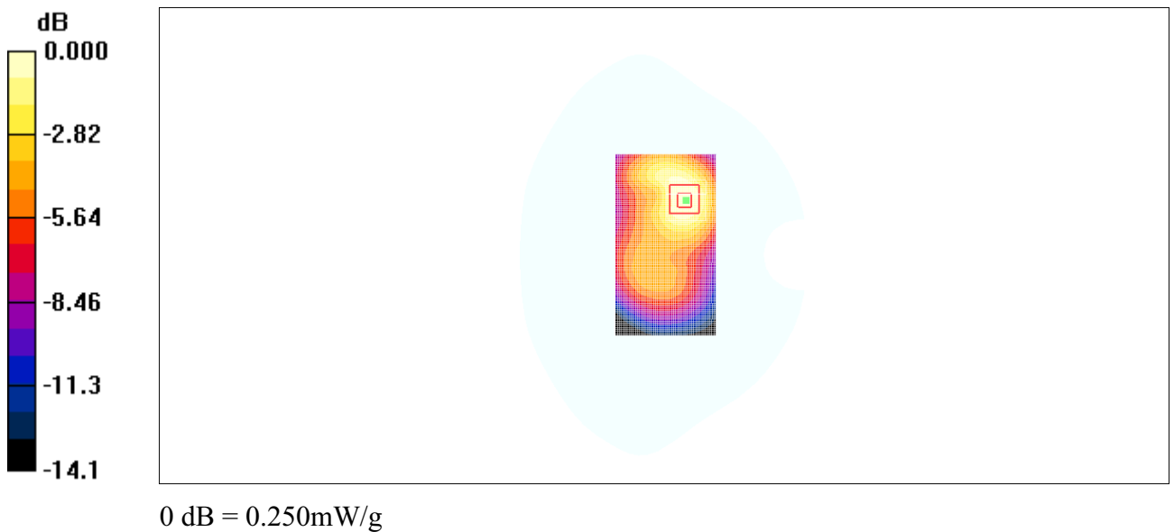
Fig. 25 1900 MHz CH512
