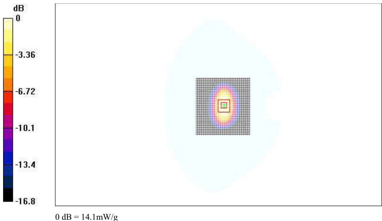
Fig.36 validation 2450MHz 250mW
