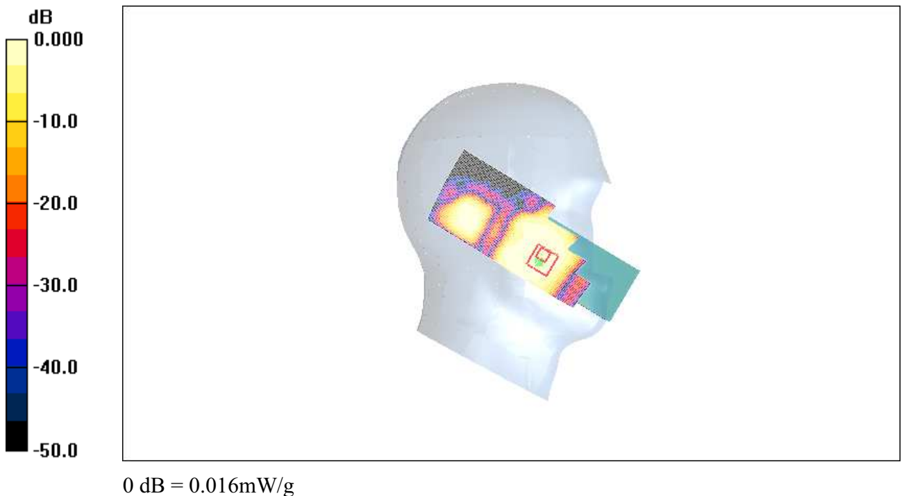
Fig.28 2450MHz CH1
