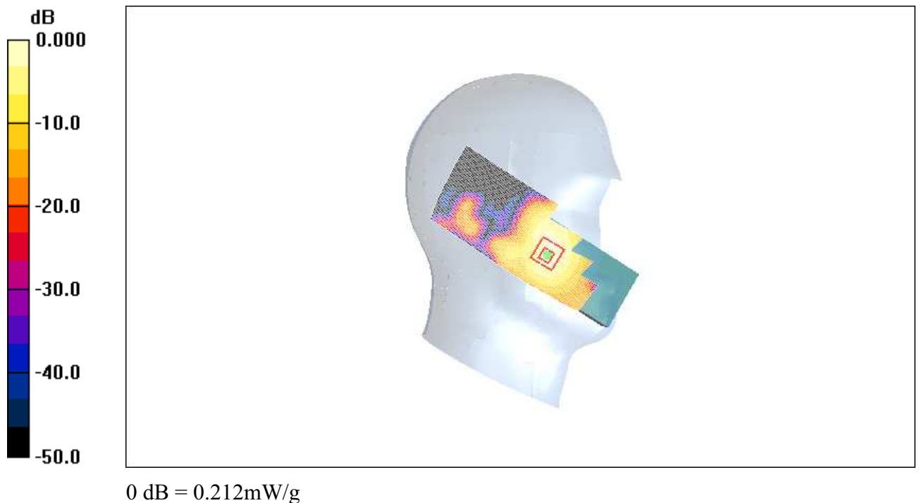
Fig.27 2450MHz CH1
