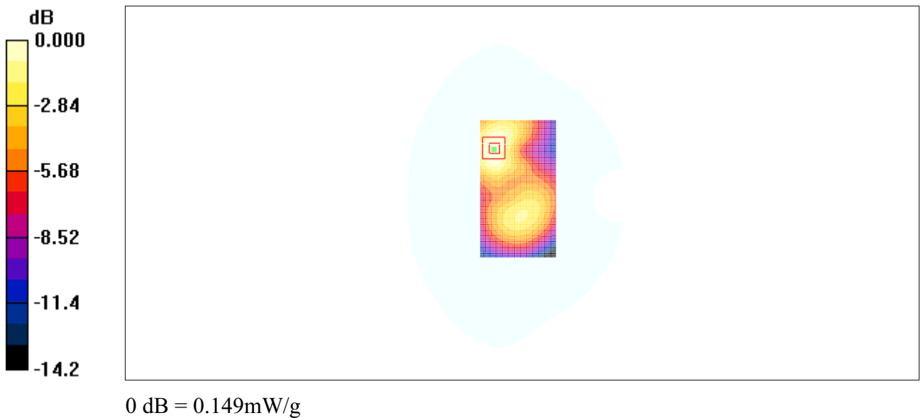
Fig. 26 1900 MHz CH512
