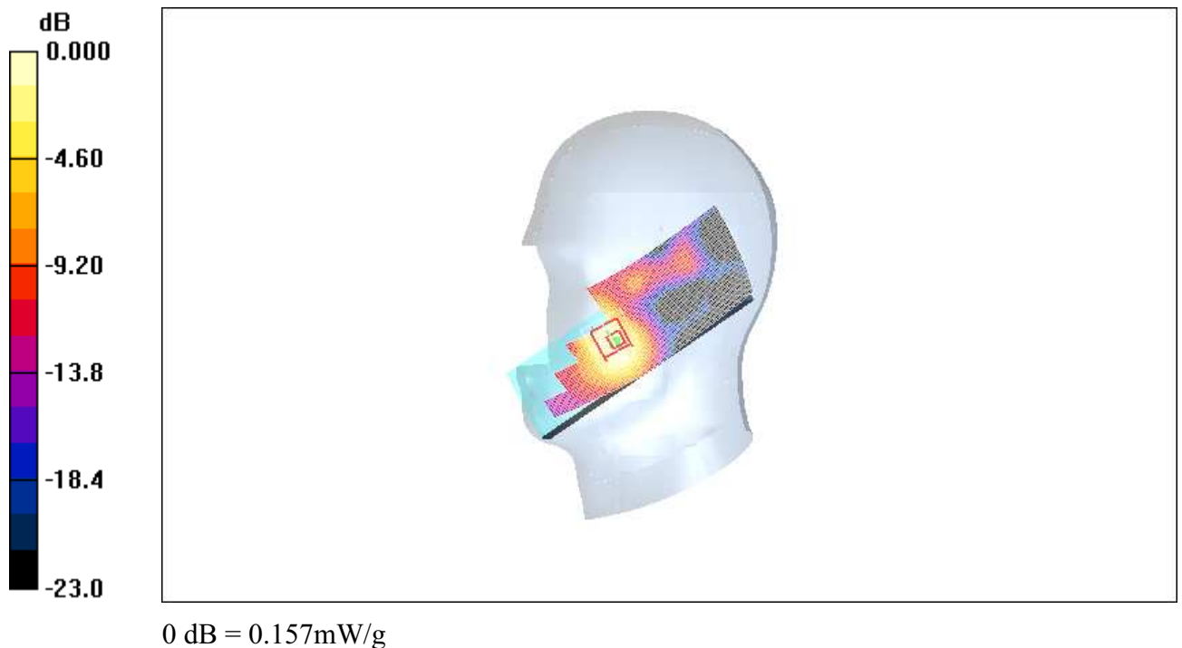
Fig.29 2450MHz CH1
