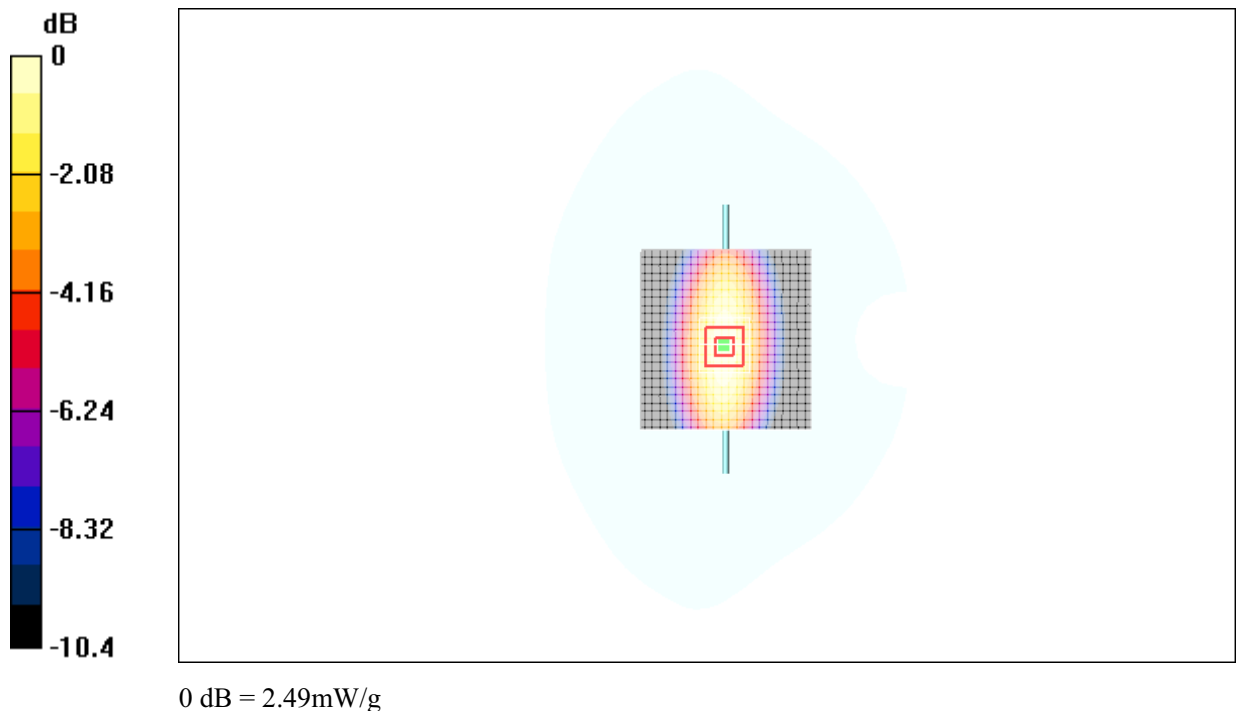
Fig.33 validation 835MHz 250mW
