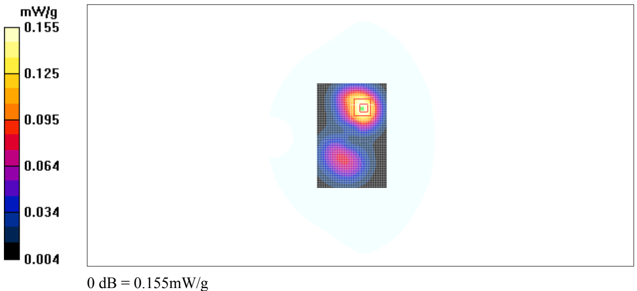
Fig. 12 1900 MHz CH512
