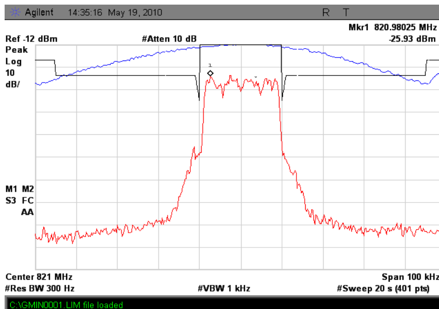
Figure 6a.2.1-2. iDEN 800 MHz Band, Quad-QPSK, Minimum Power, Emission Mask G
