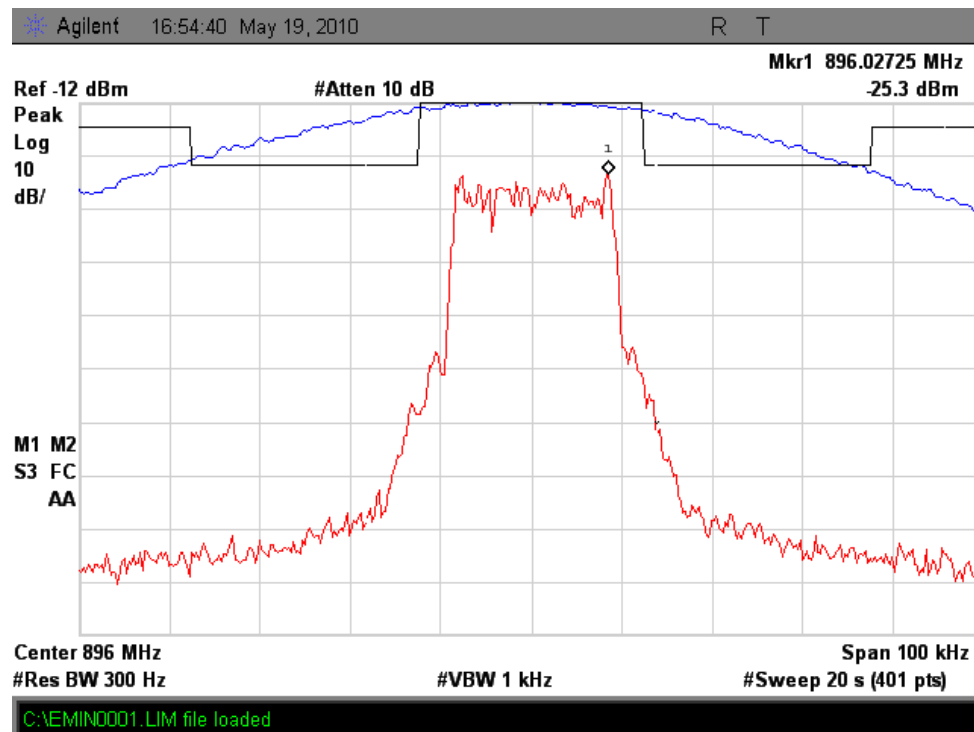
Figure 6a.2.2-12. iDEN 900 MHz Band, Quad-64QAM, Minimum Power, EA Emission Mask
