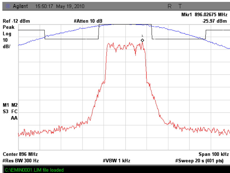
Figure 6a.2.2-8. iDEN 900 MHz Band, Quad-16QAM, Minimum Power, EA Emission Mask
