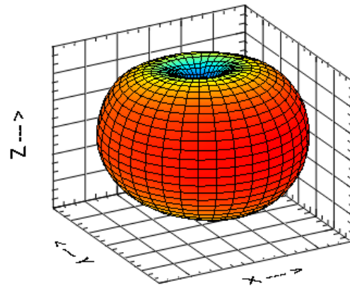
Figure 6a.6-2 Antenna pattern in the 900 MHz SMR frequency band.
