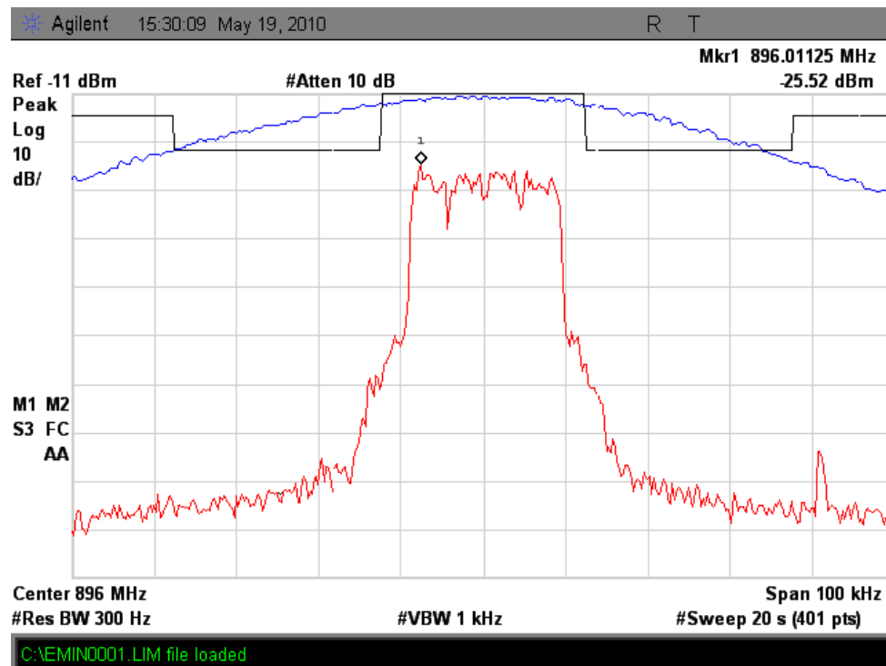
Figure 6a.2.2-4. iDEN 900 MHz Band, Quad-QPSK, Minimum Power, EA Emission Mask
