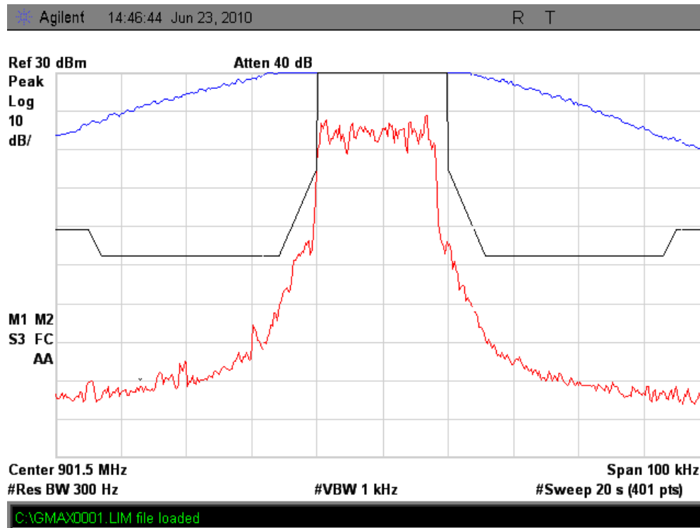
Figure 6b.2.1-3 iDEN NBPCS Band, Occupied Bandwidth, Quad-64QAM, Maximum Power.
