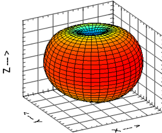
Figure 6a.6-5 Antenna pattern in the 900 MHz NBPCS frequency band.
