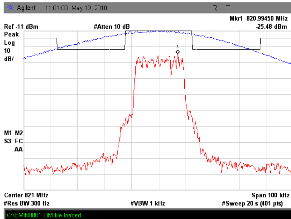
Figure 6a.2.1-8. iDEN 800 MHz Band, Quad-16QAM, Minimum Power, EA Emission Mask
