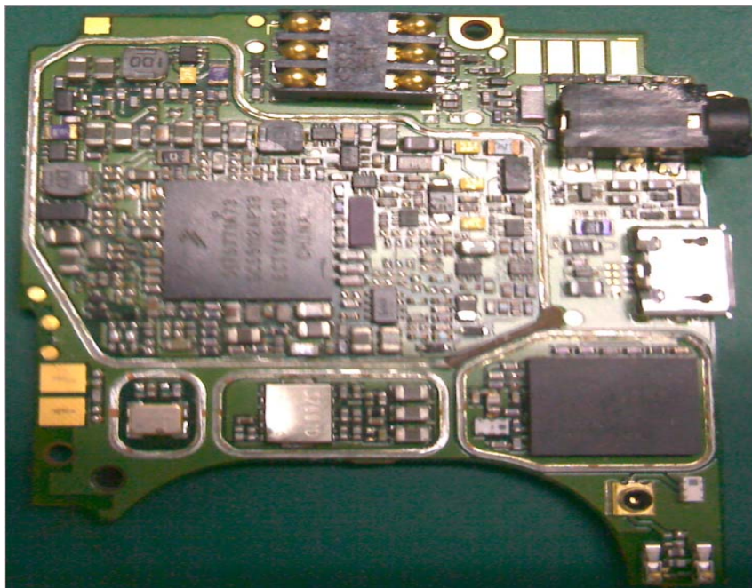
Photograph 9-3: Front side view of radio product PC Board; shields removed.
