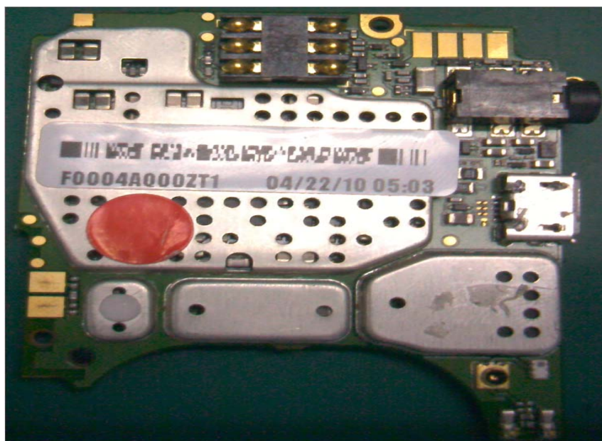
Photograph 9-2: Rear side view of radio product PC Board; shields in place.
