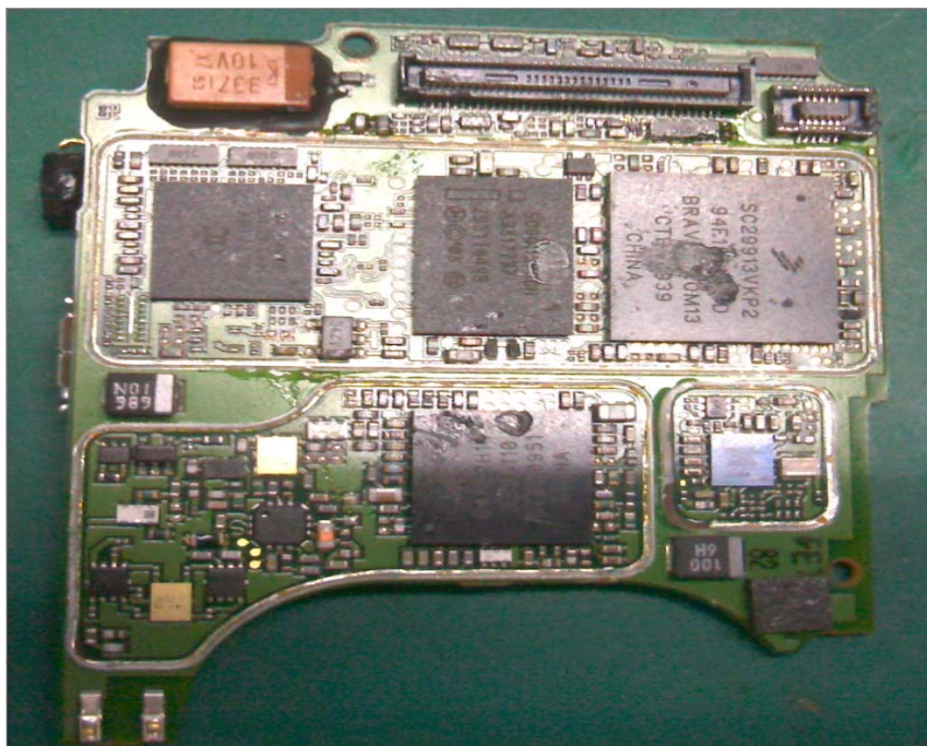
Photograph 9-4: Rear side view of radio product PC Board; shields removed.
