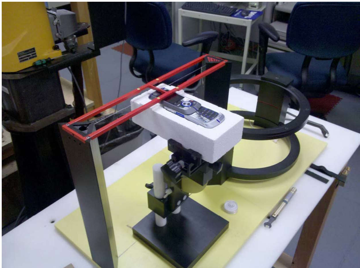
Figure 4. Positioning and Measurement for RF Emissions
