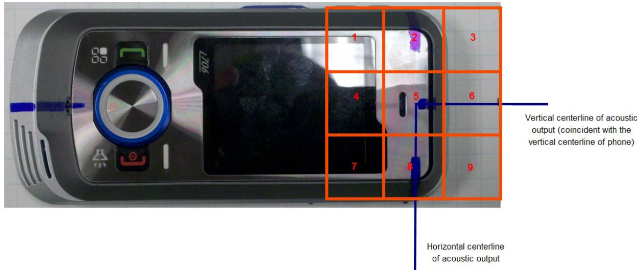
Figure 3. Phone Front - Orientation and Measurement Plane for RF Emissions Testing
