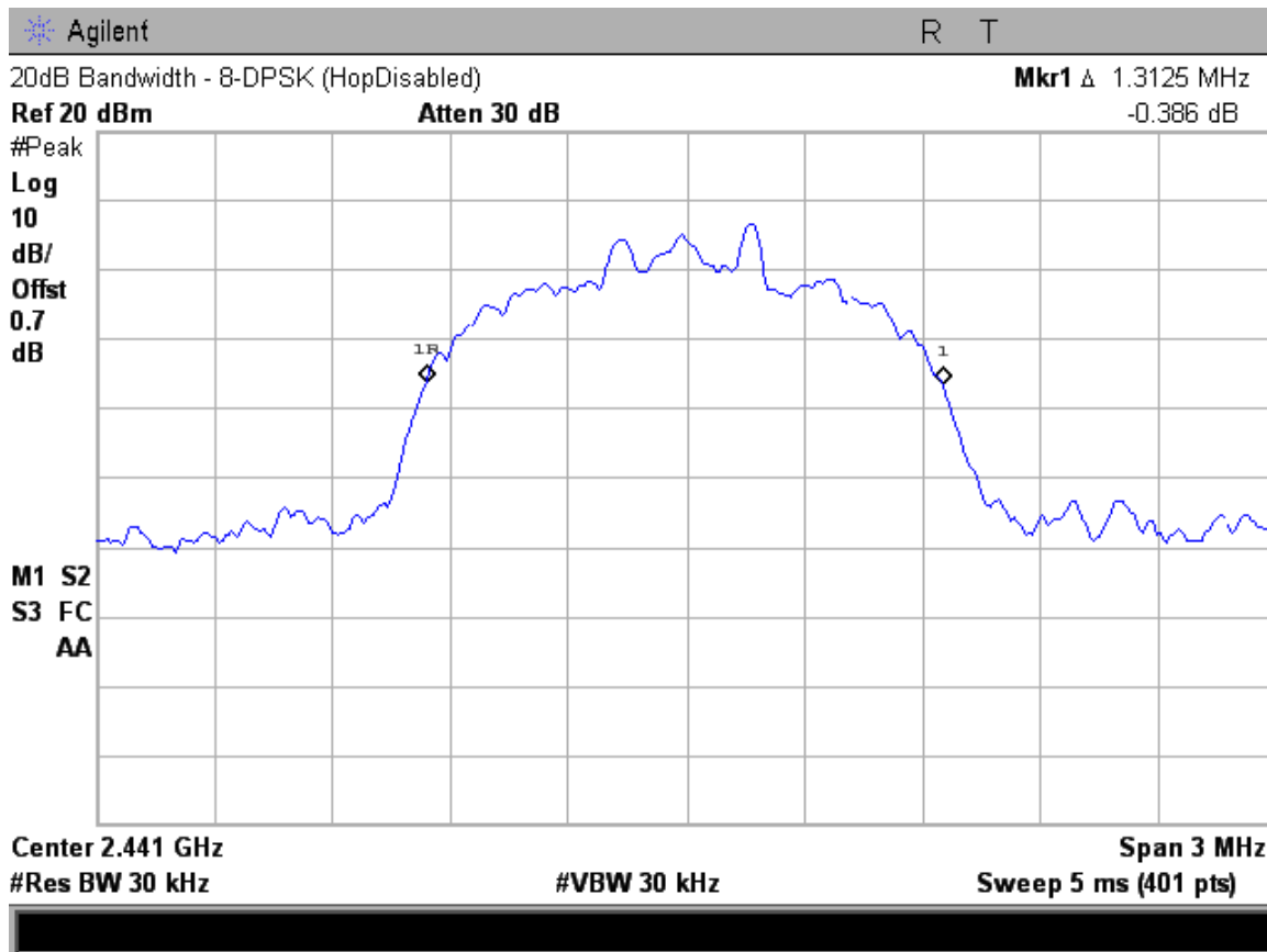
Figure 6c.2-3: Plot of 20 dB bandwidth (8-DPSK Modulation)
