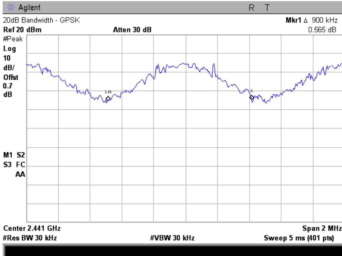
Figure 6c.2-1: Plot of 20 dB bandwidth (GFSK Modulation)
