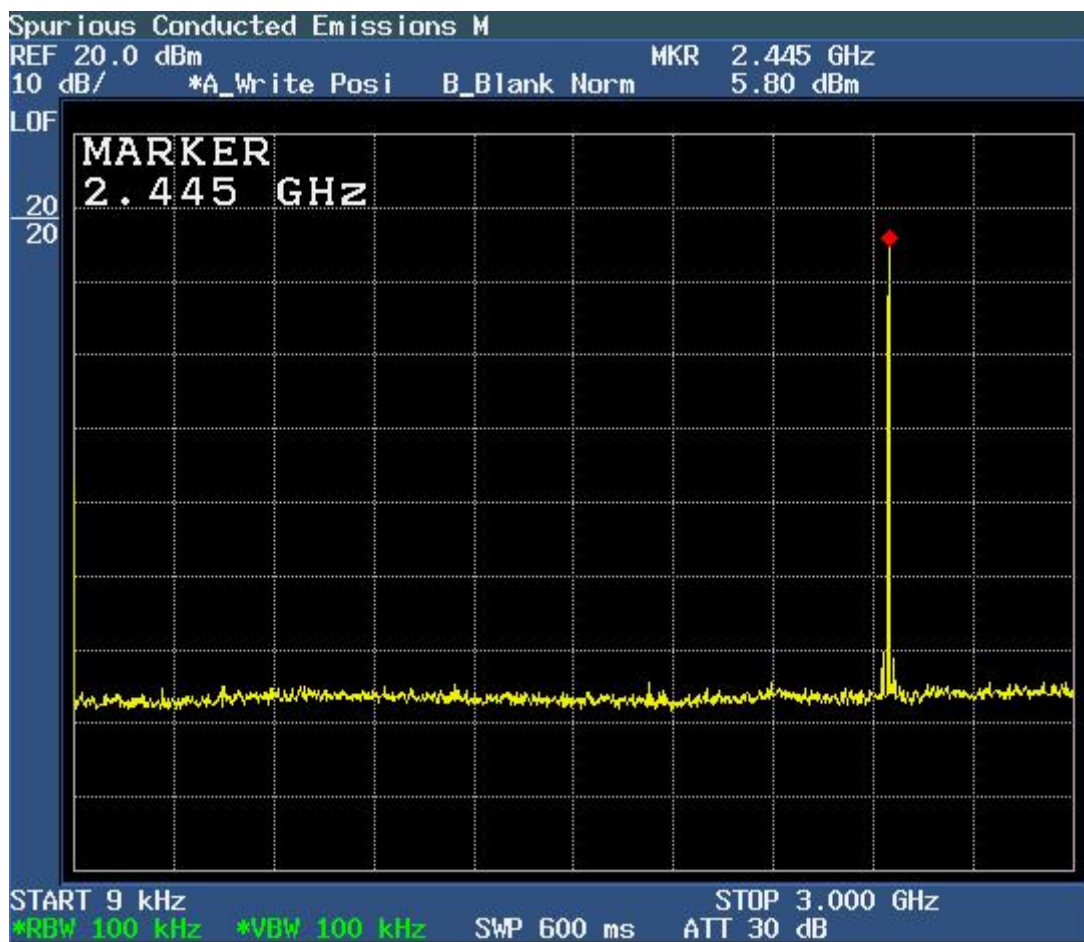
Figure 6c.8-4: Plot of spurious conducted emissions 9.0 kHz – 3.0 GHz (Mid Channel Enabled)
