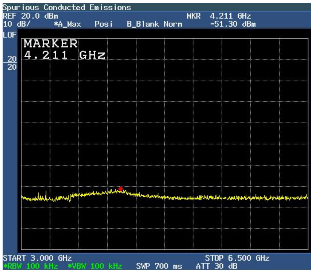
Figure 6c.8-11: Plot of spurious conducted emissions 3.0 GHz – 6.5 GHz (Hopping Enabled).
