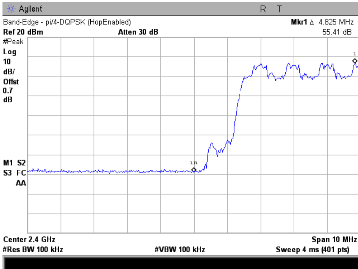
Figure 6c.6-7: Plot of lower band-edge conducted emissions with hopping enabled (Pi/4 DPSK Modulation).
