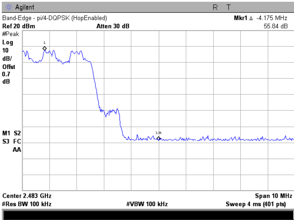
Figure 6c.6-8: Plot of upper band-edge conducted emissions with hopping enabled (Pi/4 DPSK Modulation).
