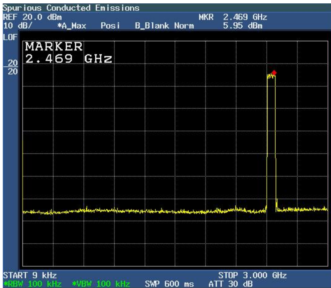
Figure 6c.8-10: Plot of spurious conducted emissions 9.0 kHz – 3.0 GHz (Hopping Enabled).
