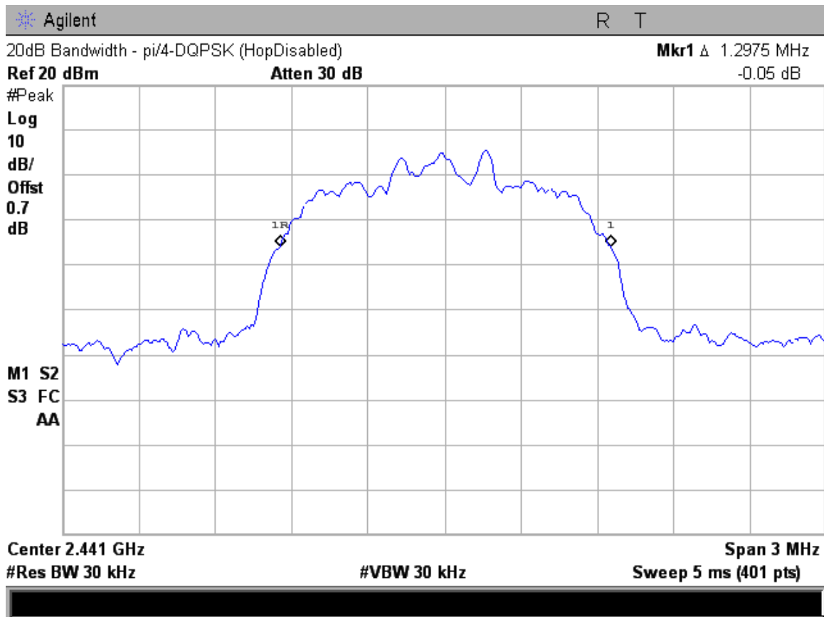
Figure 6c.2-2: Plot of 20 dB bandwidth (P/4 DPSK Modulation)
