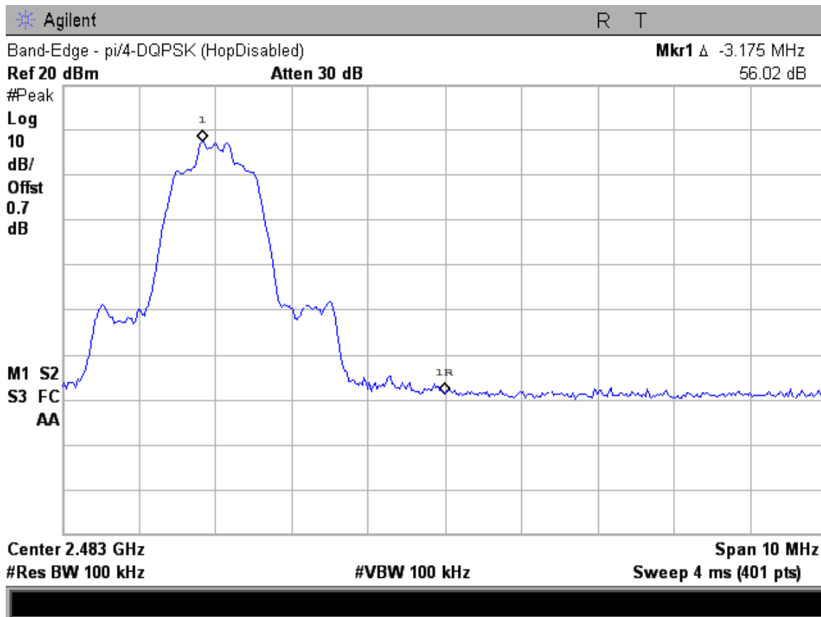
Figure 6c.6-6: Plot of upper band-edge conducted emissions with hopping disabled (Pi/4 DPSK Modulation).
