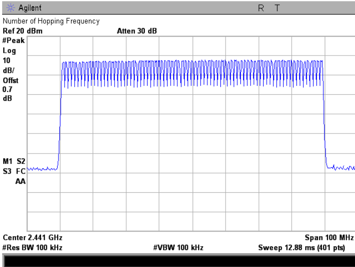
Figure 6c.3-1: Plot of number of Bluetooth hopping frequencies
