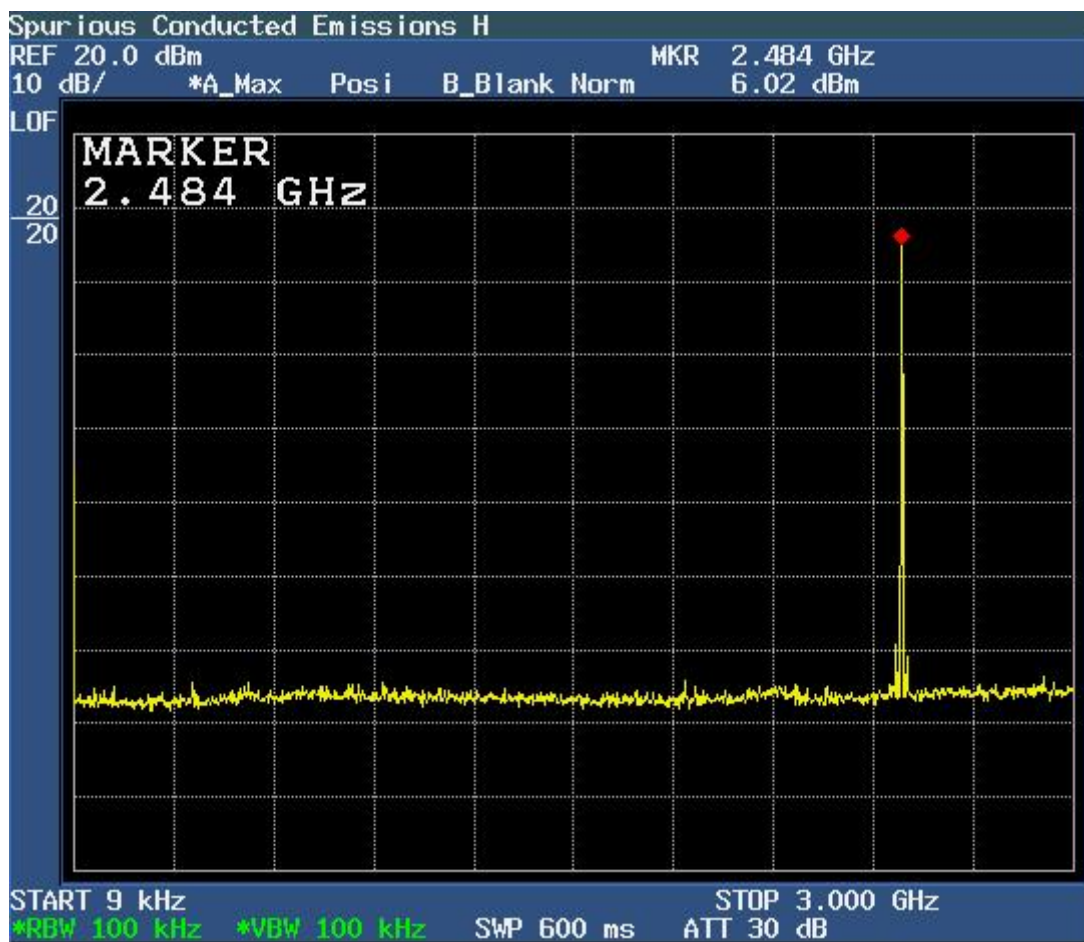
Figure 6c.8-7: Plot of spurious conducted emissions 9.0 kHz – 3.0 GHz (High Channel Enabled)
