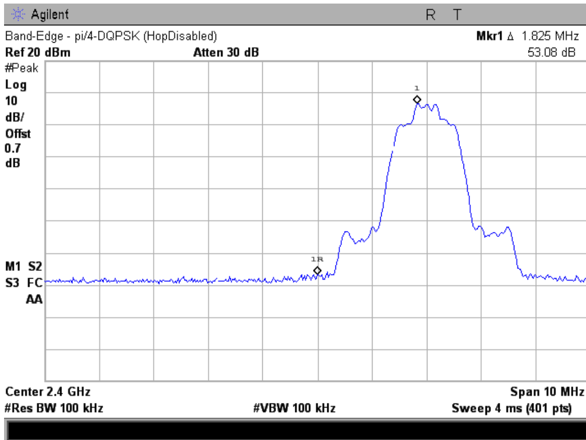
Figure 6c.6-5: Plot of lower band-edge conducted emissions with hopping disabled (Pi/4 DPSK Modulation).
