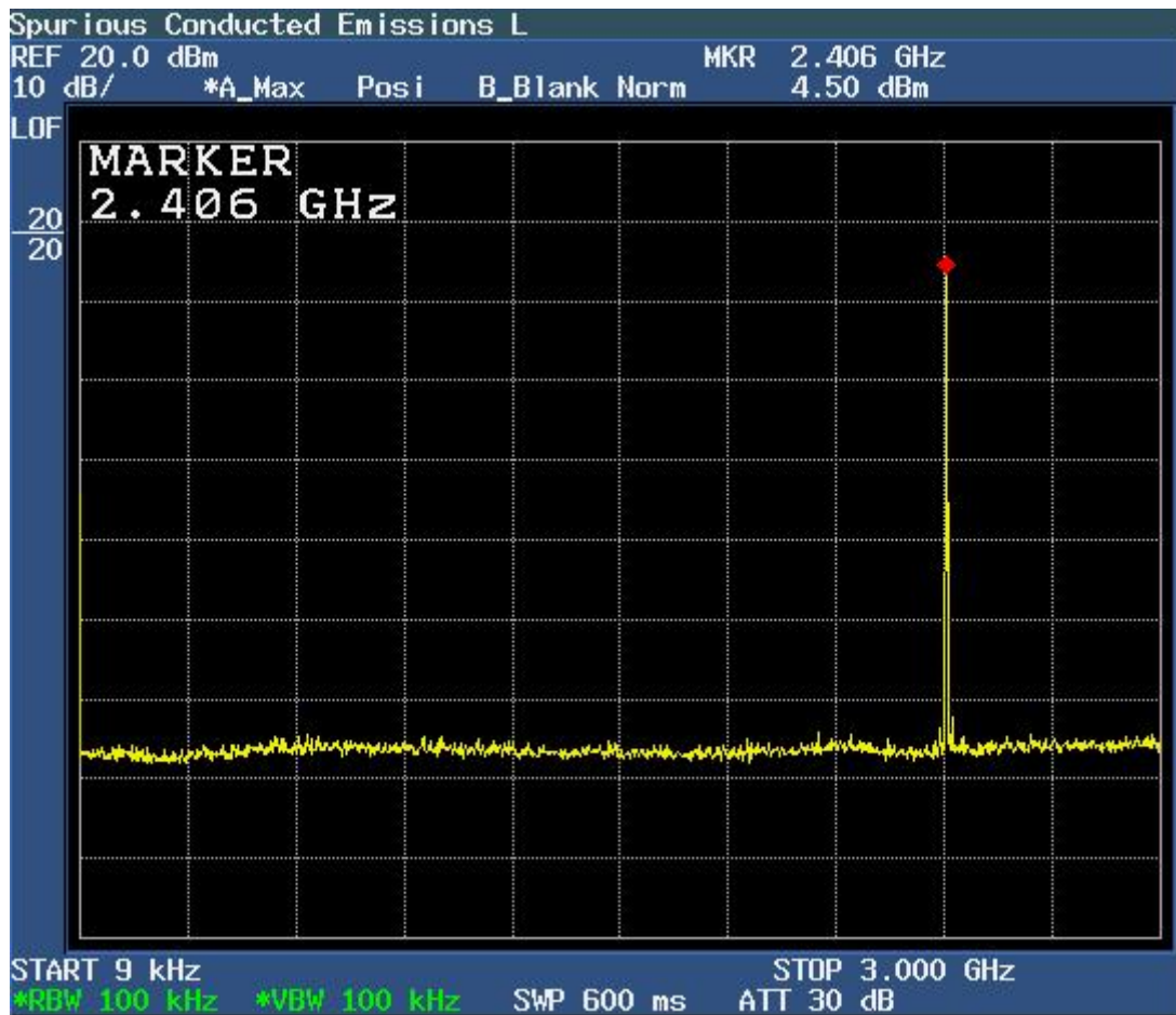
Figure 6c.8-1: Plot of spurious conducted emissions 9.0 kHz – 3.0 GHz (Low Channel Enabled)
