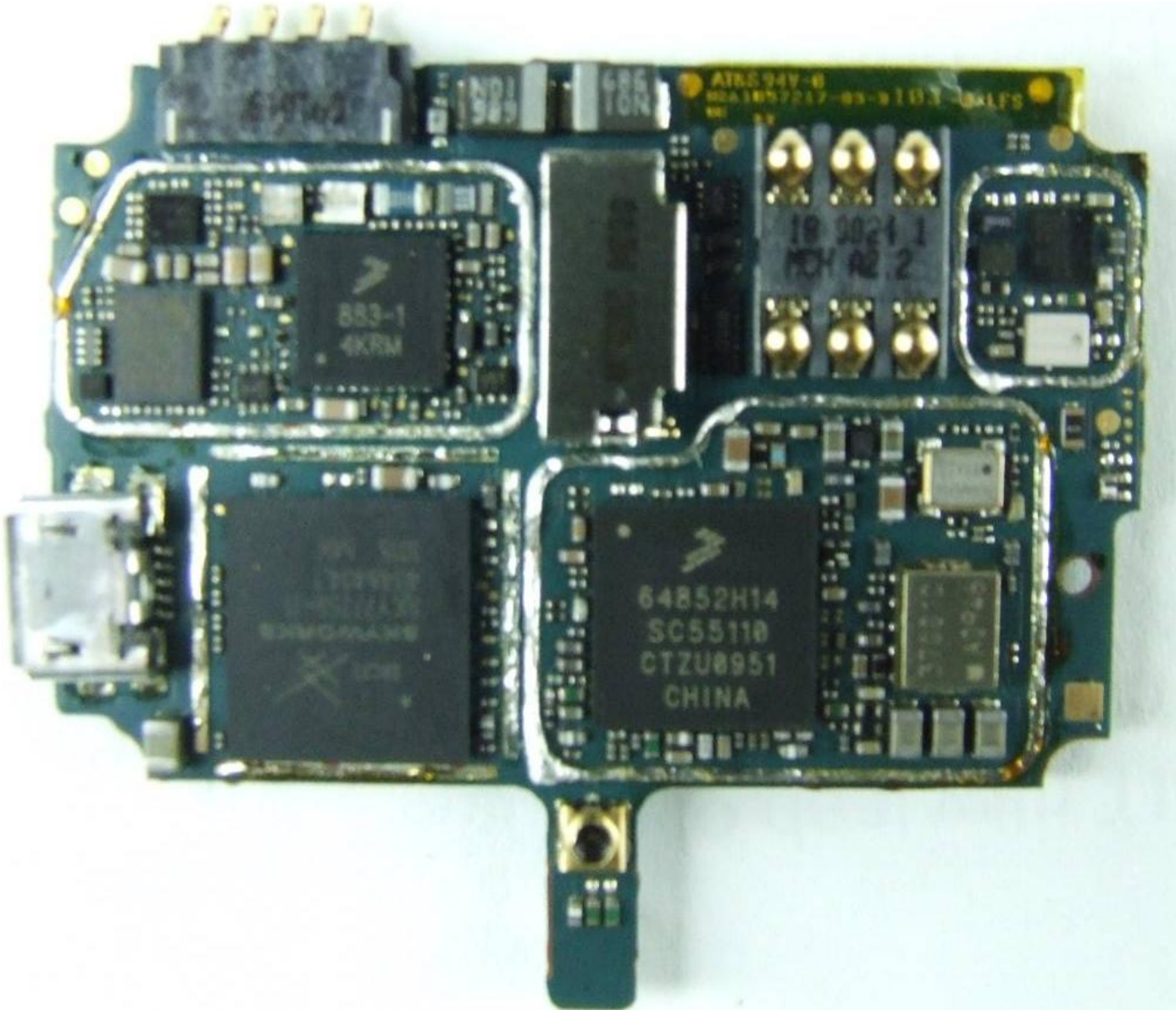
Photograph 9-4: Rear side view of radio product PC Board, Shields Removed.
