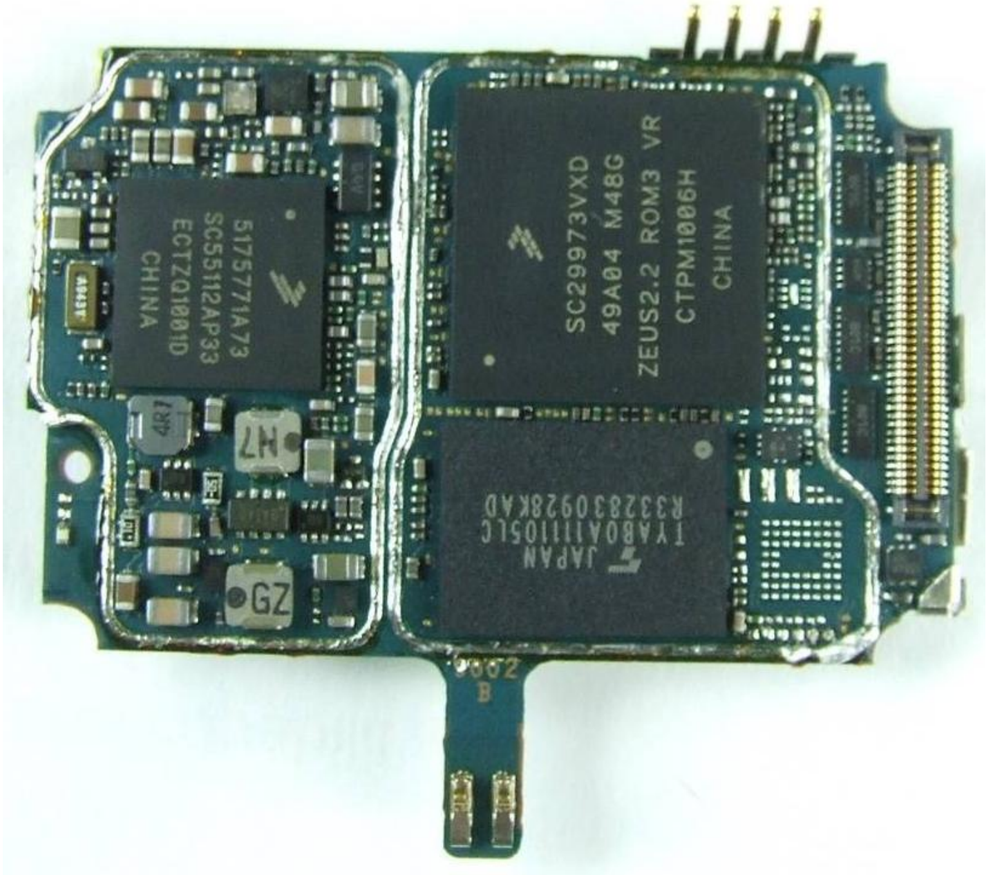
Photograph 9-2: Front side view of radio product PC Board, Shields Removed.
