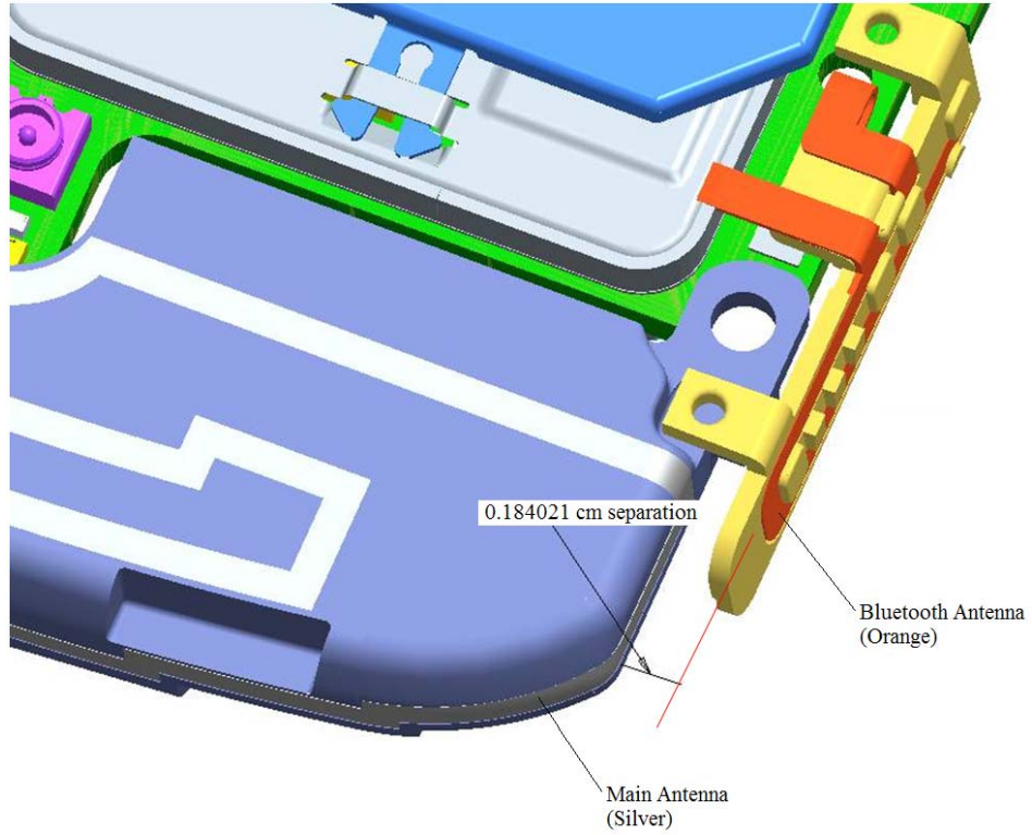
Figure 3: Antenna Separation Distances
