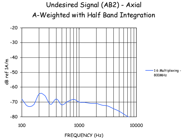
Figure 9-2-2: 800 MHz Undesired Signal (1:6)
