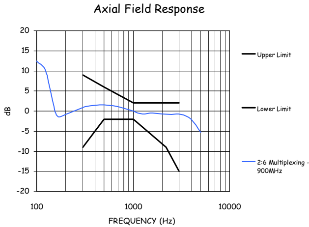
Figure 9-1-3: 900 MHz Measured Frequency Response (2:6)
