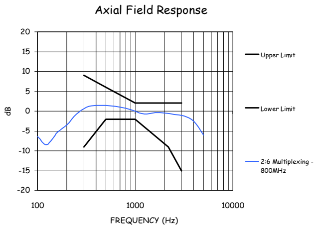
Figure 9-1-1: 800 MHz Measured Frequency Response (2:6)
