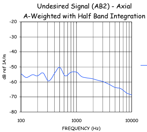
Figure 9-4-1: 900 MHz Undesired Signal (2:6)
