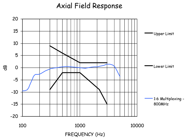
Figure 9-1-2: 800 MHz Measured Frequency Response (1:6)
