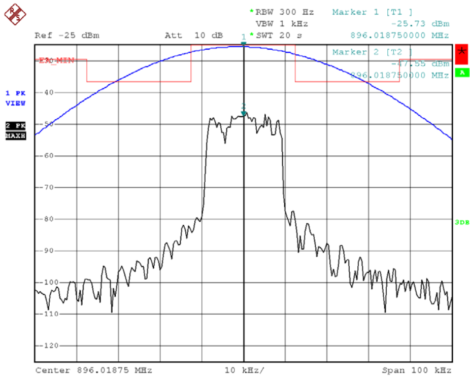
Figure 6a-2.2.8. iDEN 900 MHz Band, QAM16, Minimum Power, EA Emission Mask
