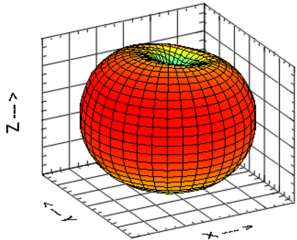
Figure 6a.6-2 Antenna pattern in the 900 MHz SMR frequency band (Flip Open).
