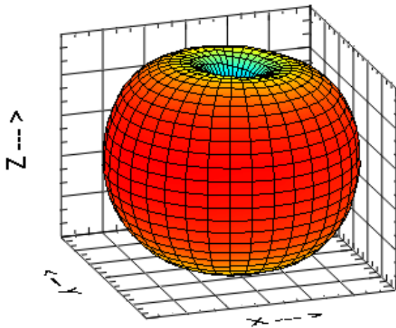
Figure 6a.6-1 Antenna pattern in the 800 MHz SMR frequency band (Flip Open).
