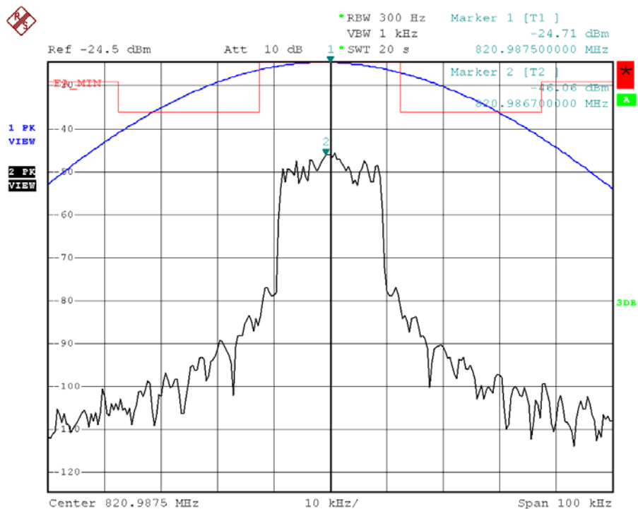
Figure 6a-2.1.12. iDEN 800 MHz Band, QAM64, Minimum Power, EA Emission Mask
