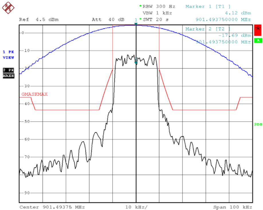
Figure 6b.2.1-3. iDEN NBPCS Band, Occupied Bandwidth, Quad-64QAM, Maximum Power.
