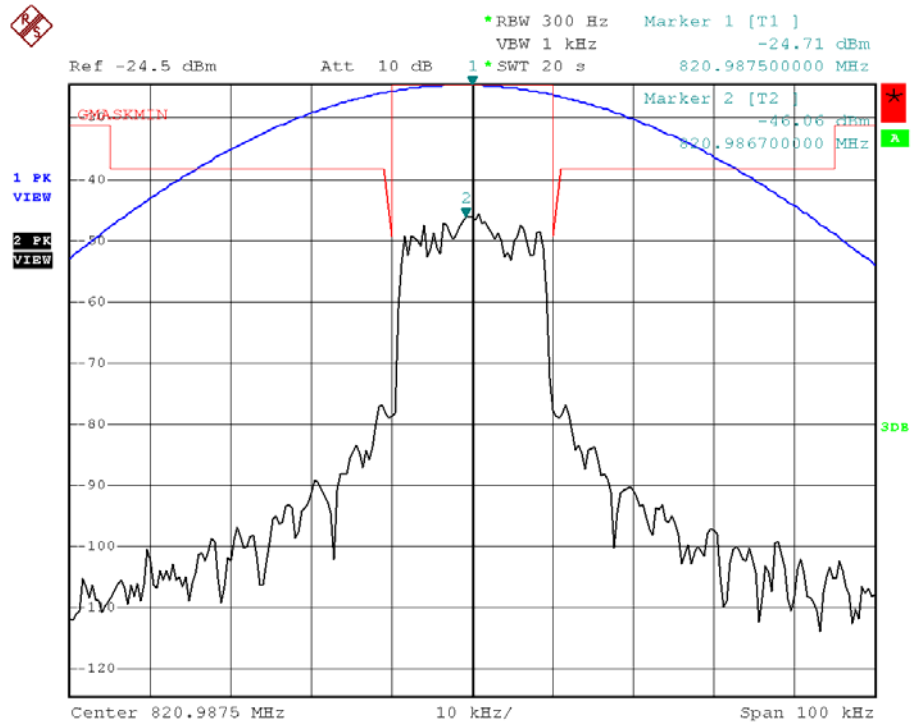
Figure 6a-2.1.10. iDEN 800 MHz Band, QAM64, Minimum Power, Emission Mask G
