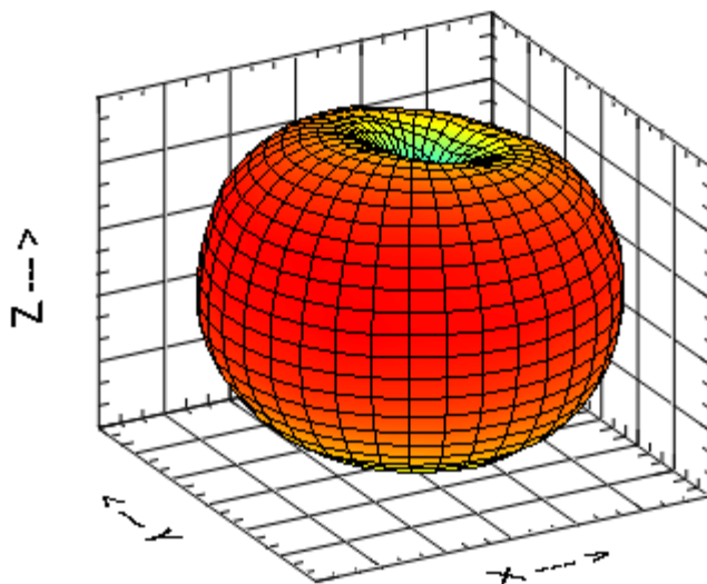
Figure 6a.6-5 Antenna pattern in the 900 MHz NBPCS frequency band (Flip Open).
