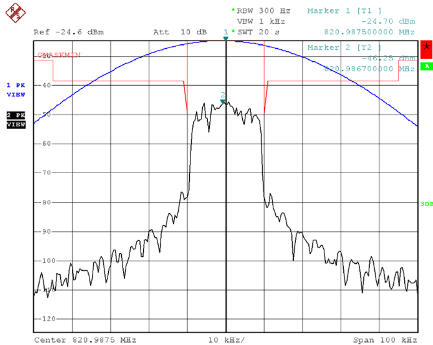
Figure 6a-2.1.6. iDEN 800 MHz Band, QAM16, Minimum Power, Emission Mask G
