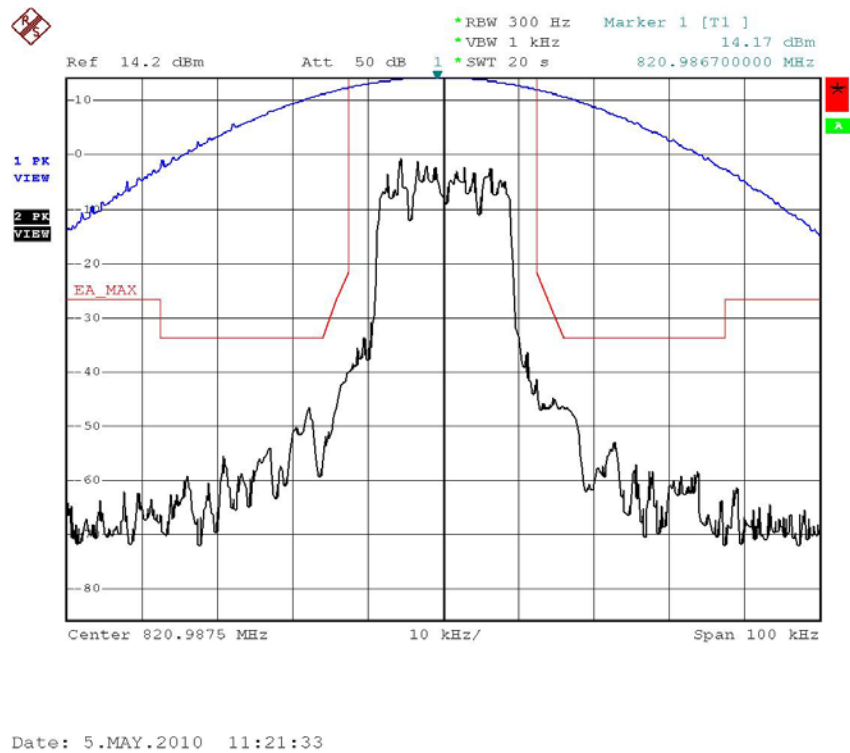
Figure 6a.2.1-7. iDEN 800 MHz Band, Quad-16QAM, Maximum Power, EA Emission Mask
