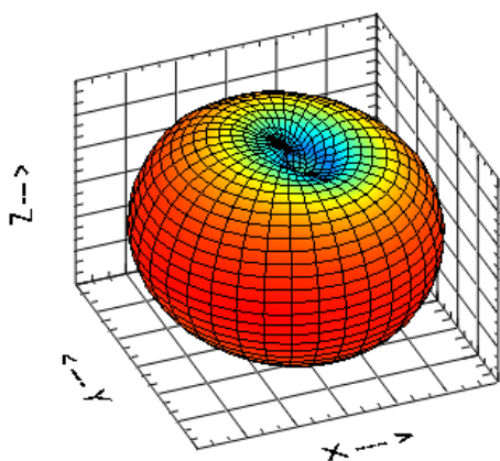
Figure 6a.6-1 Antenna pattern in the 800 MHz SMR frequency band (Slider Open).
