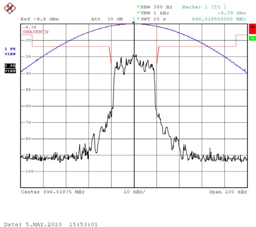
Figure 6a.2.2-6. iDEN 900 MHz Band, Quad-16QAM, Minimum Power, Emission Mask G
