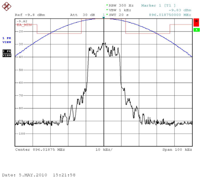
Figure 6a.2.2-4. iDEN 900 MHz Band, Quad-QPSK, Minimum Power, EA Emission Mask
