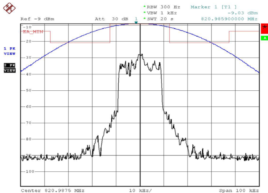
Figure 6a.2.1-11. iDEN 800 MHz Band, Quad-64QAM, Maximum Power, EA Emission Mask
