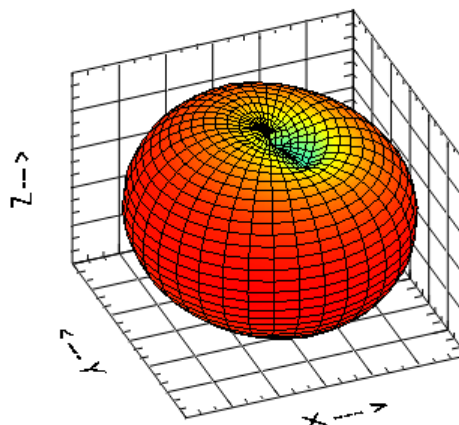
Figure 6a.6-4 Antenna pattern in the 900 MHz SMR frequency band (Slider Closed).
