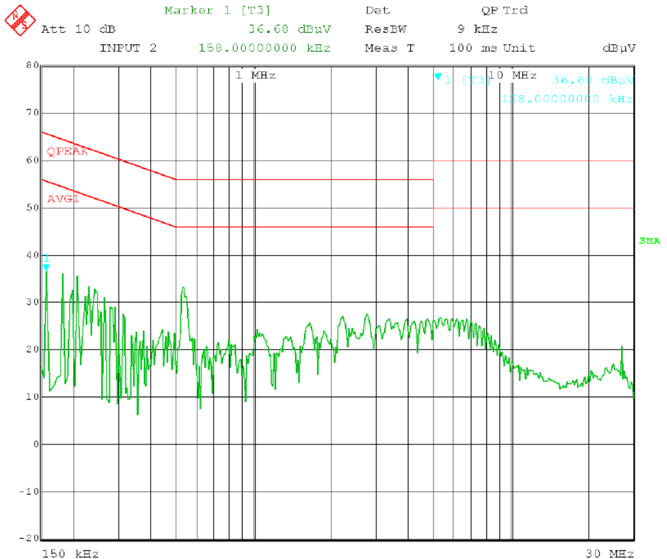
Figure 6a.4-6: iDEN NBPCS Band Neutral Line Spurious Voltage with a Peak Detector (901.49375 MHz).
