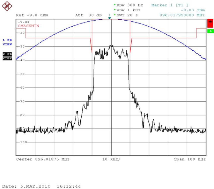
Figure 6a.2.2-10. iDEN 900 MHz Band, Quad-64QAM, Minimum Power, Emission Mask G
