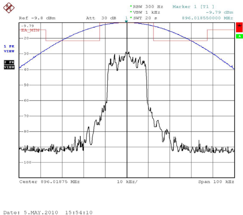
Figure 6a.2.2-8. iDEN 900 MHz Band, Quad-16QAM, Minimum Power, EA Emission Mask
