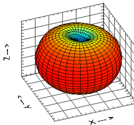
Figure 6a.6-2 Antenna pattern in the 800 MHz SMR frequency band (Slider Closed).
