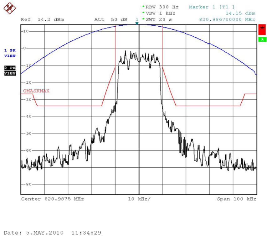
Figure 6a.2.1-5. iDEN 800 MHz Band, Quad-16QAM, Maximum Power, Emission Mask G
