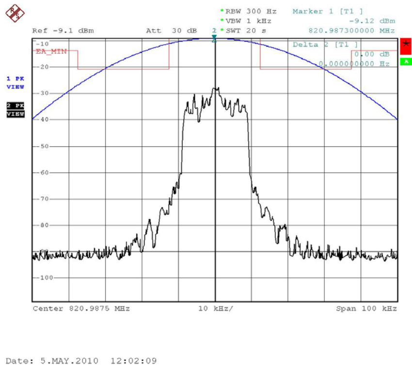
Figure 6a.2.1-8. iDEN 800 MHz Band, Quad-16QAM, Minimum Power, EA Emission Mask
