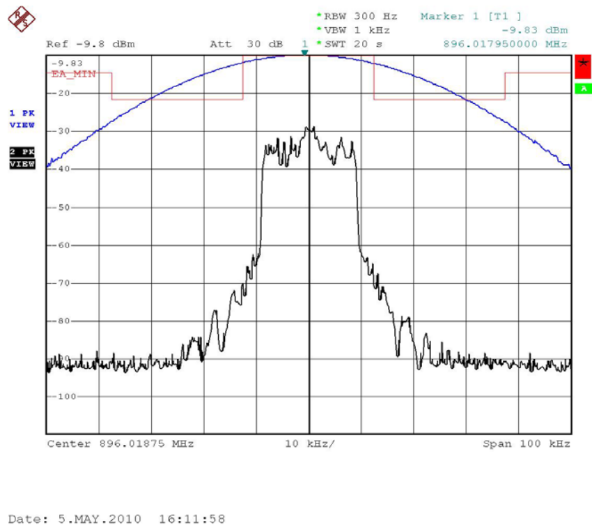
Figure 6a.2.2-12. iDEN 900 MHz Band, Quad-64QAM, Minimum Power, EA Emission Mask
