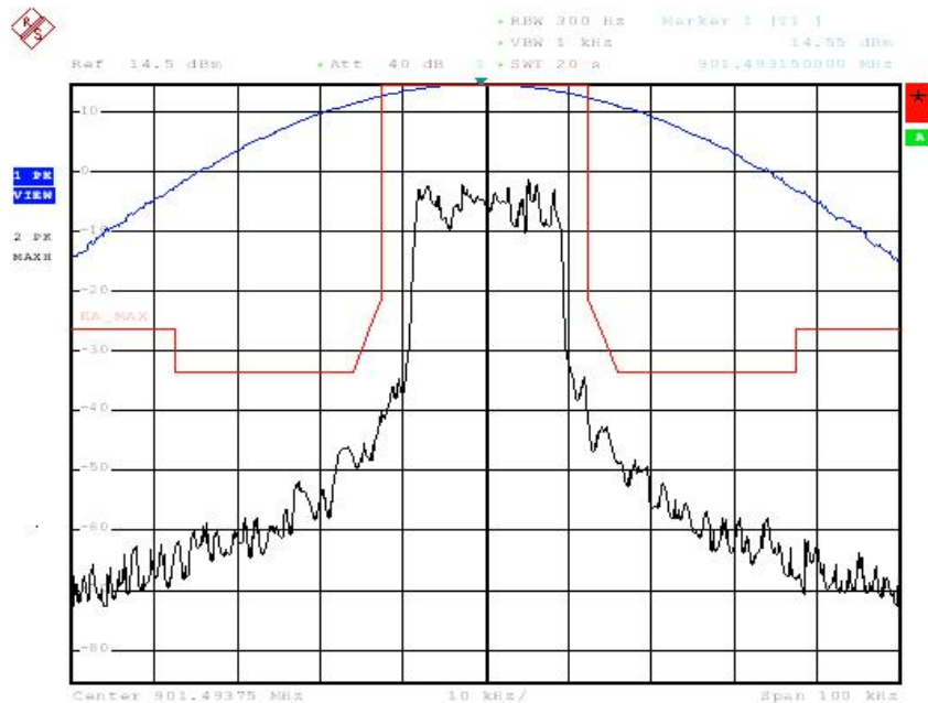
Figure 6b.2.1-2. iDEN NBPCS Band, Occupied Bandwidth, Quad-16QAM, Maximum Power.
