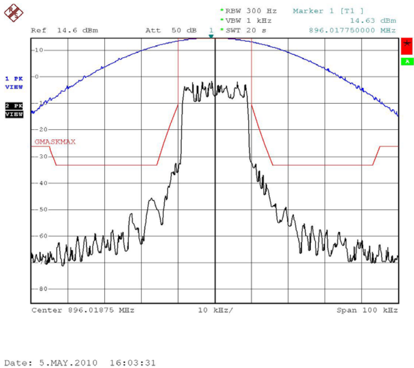
Figure 6a.2.2-9. iDEN 900 MHz Band, Quad-64QAM, Maximum Power, Emission Mask G
