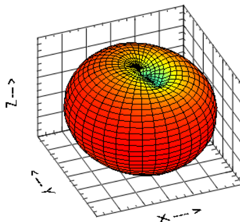
Figure 6a.6-6 Antenna pattern in the 900 MHz NBPCS frequency band (Slider Closed).
