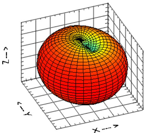
Figure 6a.6-5 Antenna pattern in the 900 MHz NBPCS frequency band (Slider Open).
