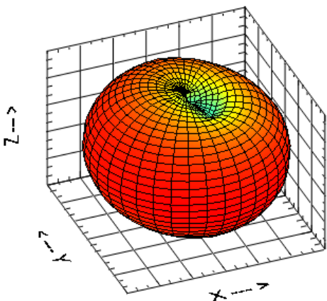
Figure 6a.6-3 Antenna pattern in the 900 MHz SMR frequency band (Slider Open).
