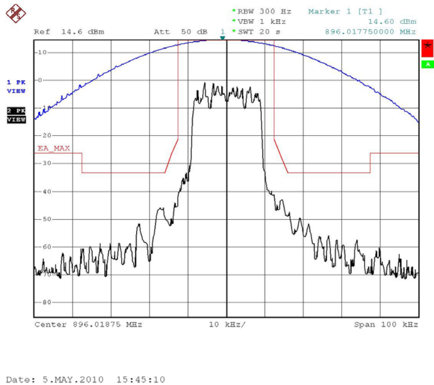
Figure 6a.2.2-7. iDEN 900 MHz Band, Quad-16QAM, Maximum Power, EA Emission Mask
