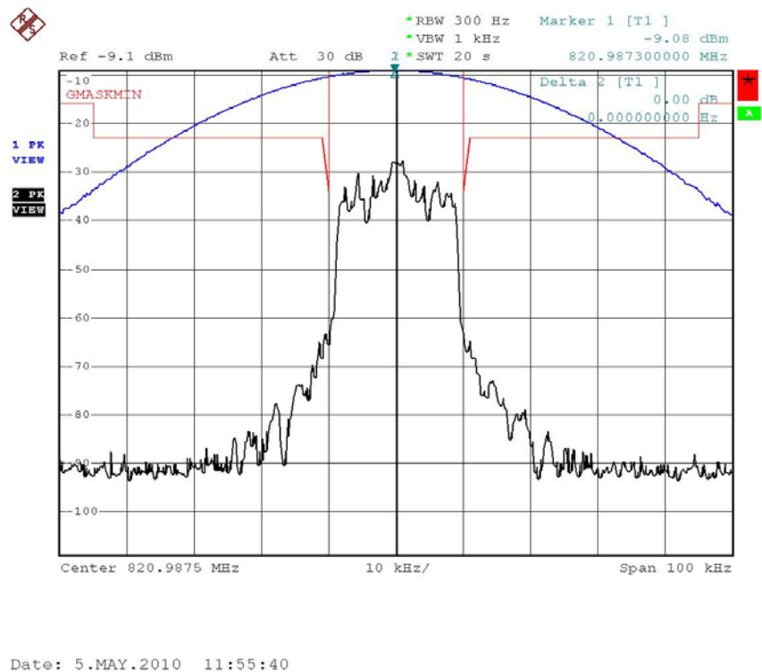
Figure 6a.2.1-6. iDEN 800 MHz Band, Quad-16QAM, Minimum Power, Emission Mask G
