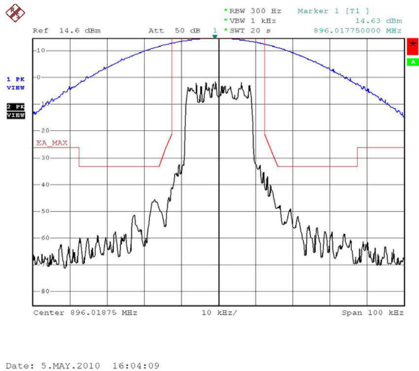
Figure 6a.2.2-11. iDEN 900 MHz Band, Quad-64QAM, Maximum Power, EA Emission Mask
