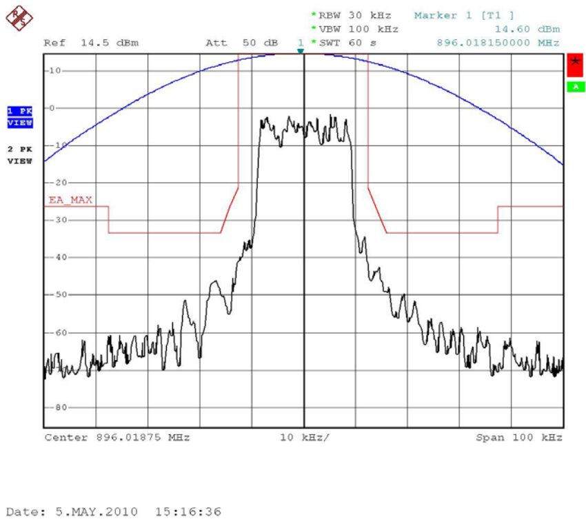
Figure 6a.2.2-3. iDEN 900 MHz Band, Quad-QPSK, Maximum Power, EA Emission Mask
