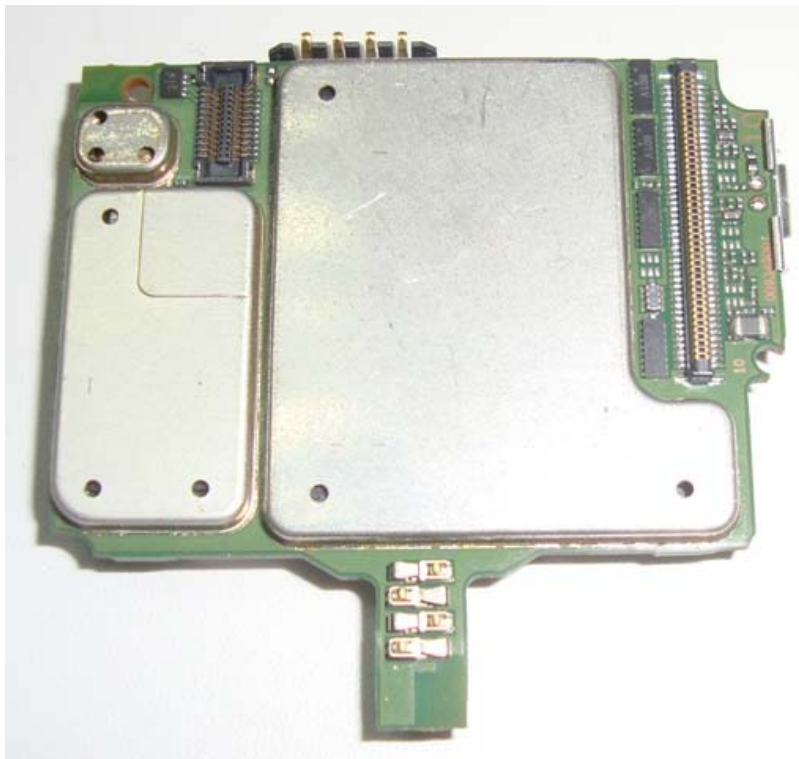
Photograph 9-3: Back side view of radio product PC Board. Shields in Place.
