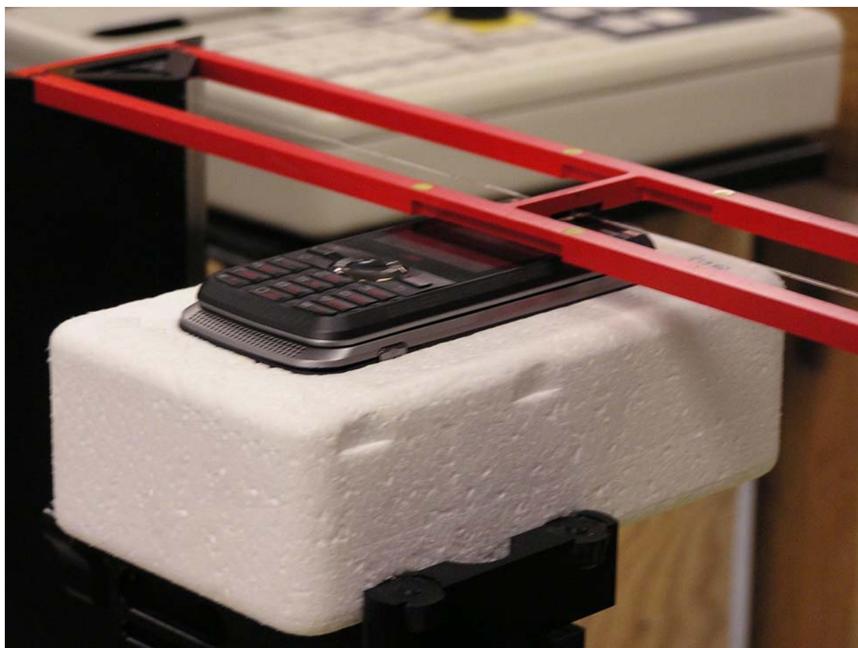
Figure 5. Positioning and Measurement for RF Emissions
