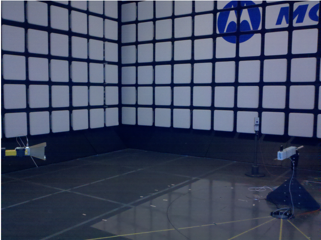
Radiated Emissions
