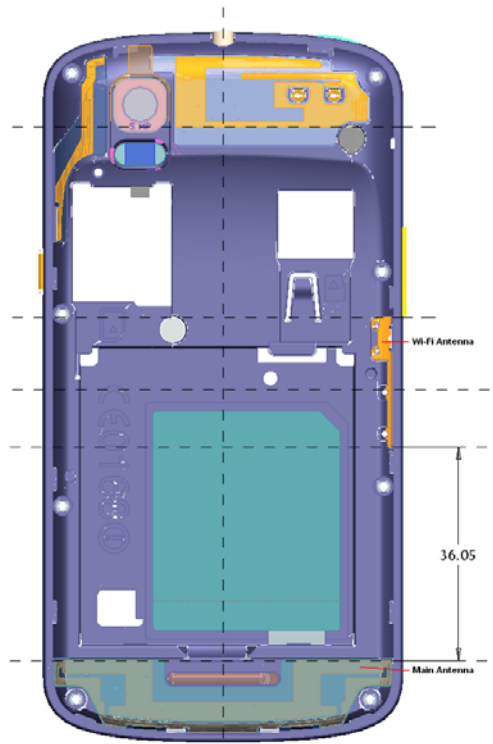
Figure 2: Antenna Separation
