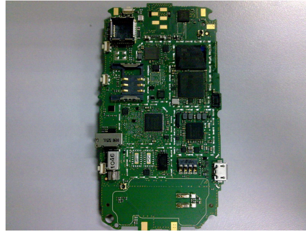
Main Board bottom Without Shields
