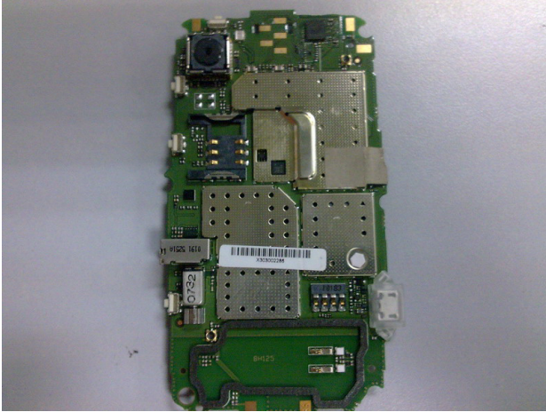
Main Board bottom With Shields
