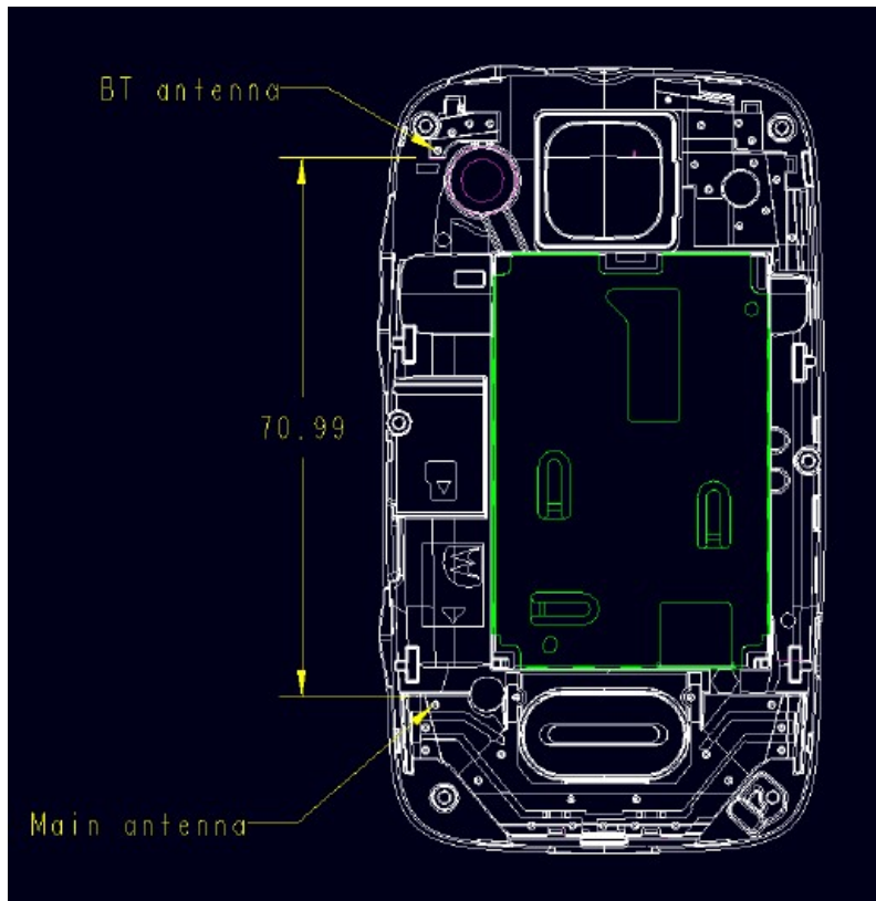
Figure 6: Antenna Separation Distance
