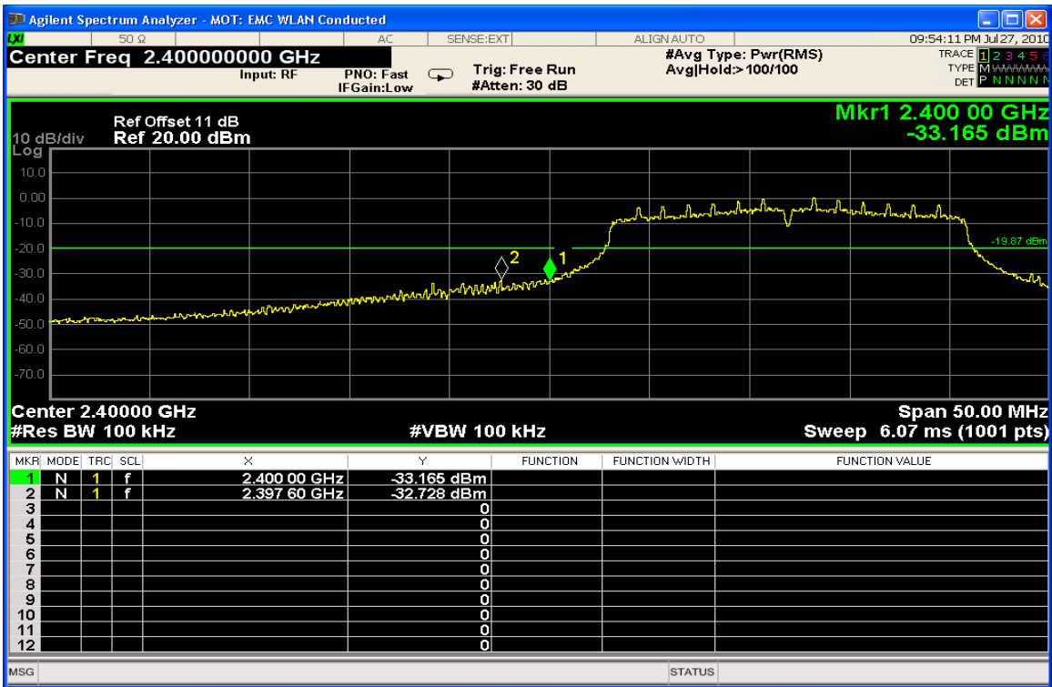
Channel 1 @ 6.5 Mbps – Lower Band Edge
