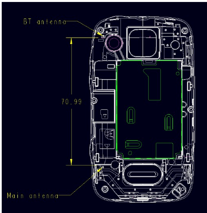
Figure 6: Antenna Separation Distance
