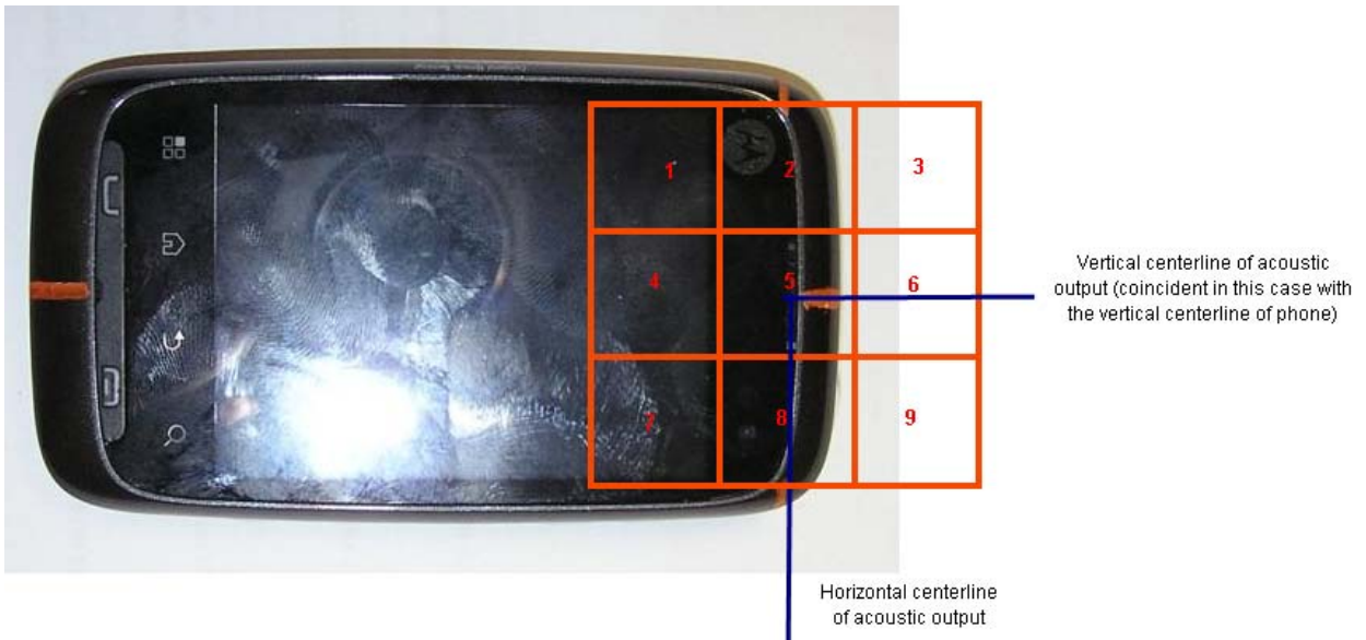
Figure 4. Phone Front - Orientation and Measurement Plane for RF Emissions Testing
