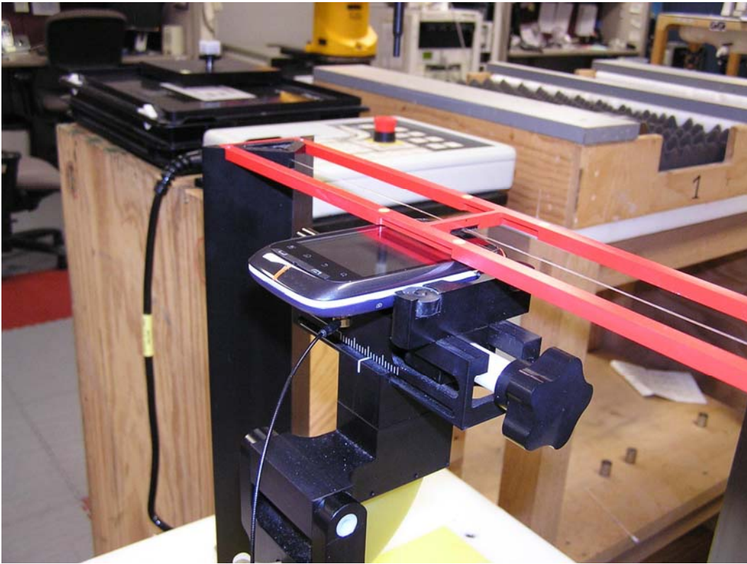
Figure 5. Positioning and Measurement for T-coil
