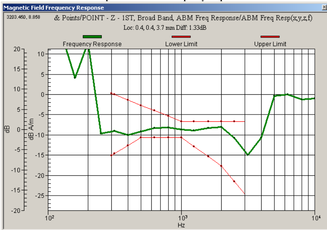
Graph 3: CDMA 1900 Frequency Response
