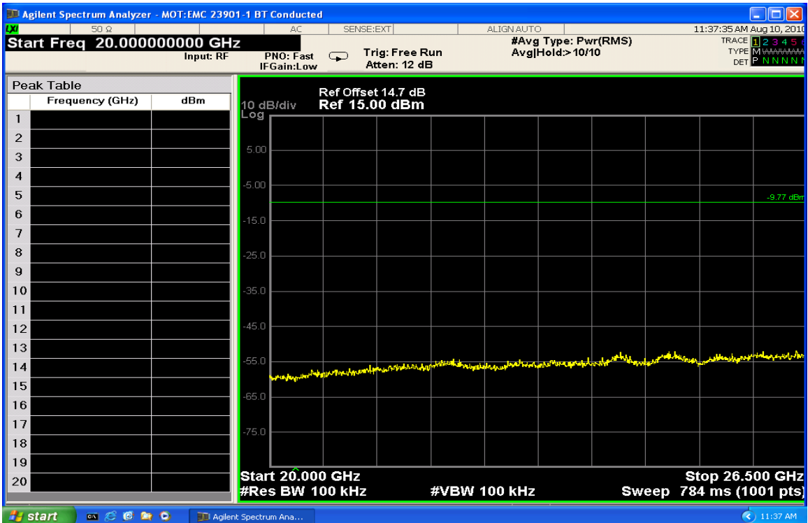
Conducted Spurious Emissions 20-26.5GHz (Low Channel Enabled)
