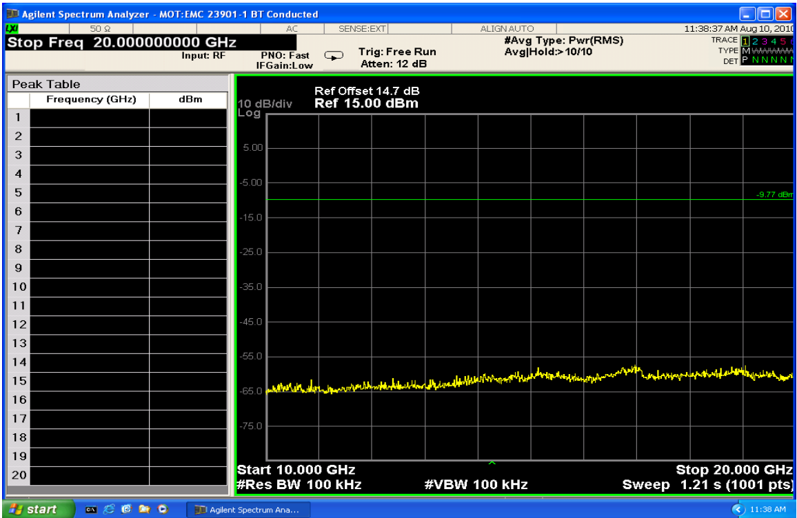
Conducted Spurious Emissions 10-20GHz (Low Channel Enabled)
