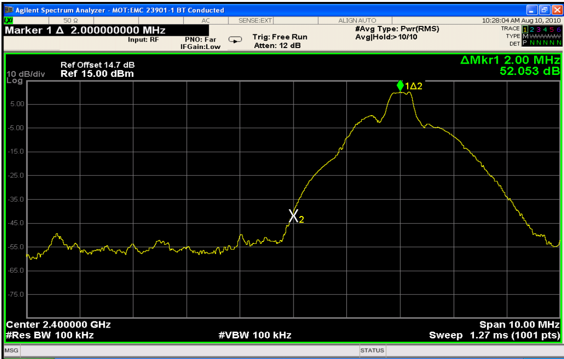
Low Band edge with Hopping Disabled
