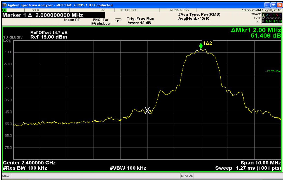
Low Band Edge with Hopping Disabled (EDR MODE)
