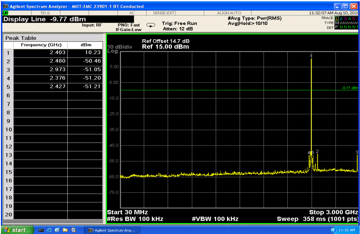
Conducted Spurious Emissions 30-3000MHz (Low Channel Enabled)
