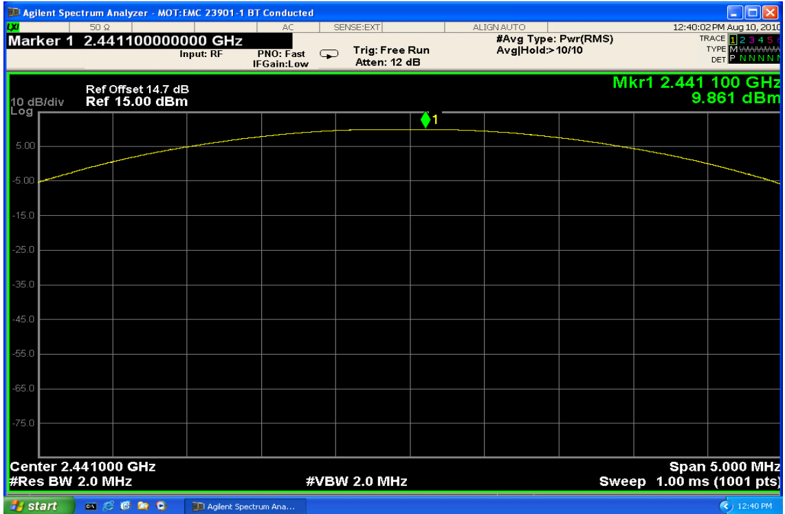
Peak Output Power EDR Mode – Mid Channel
