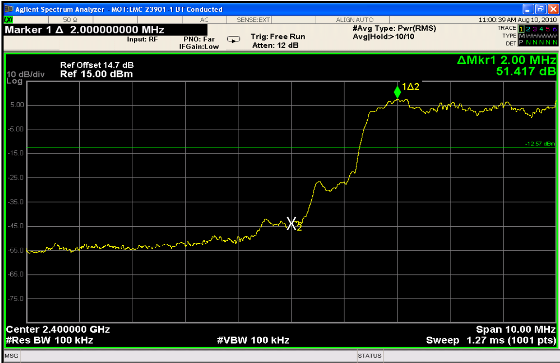
Low Band Edge with Hopping Enabled (EDR MODE)
