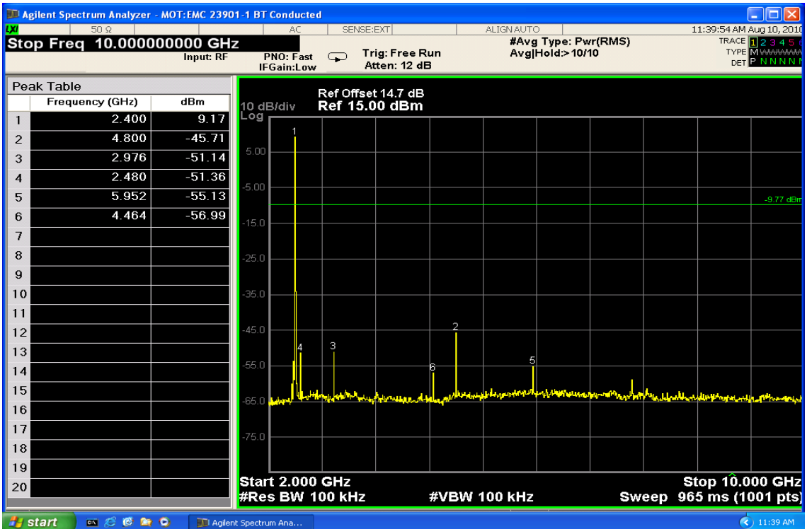
Conducted Spurious Emissions 2-10GHz (Low Channel Enabled)
